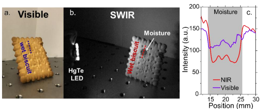
Figure III.41 Visible (a) and SWIR (b) image of a biscuit presenting a moisture stain. (c) Modulation of the intensity of the scattered light from the biscuit around the moisture stain. In the SWIR, the contrast is \approx 3 times higher.
