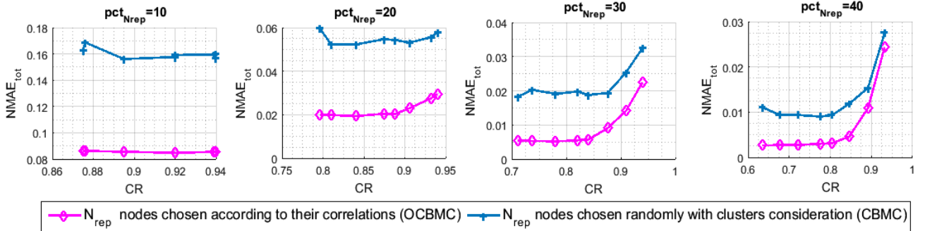
Fig. 4.13. The impact of the representative node selection technique on the NMAE_{tot} .
