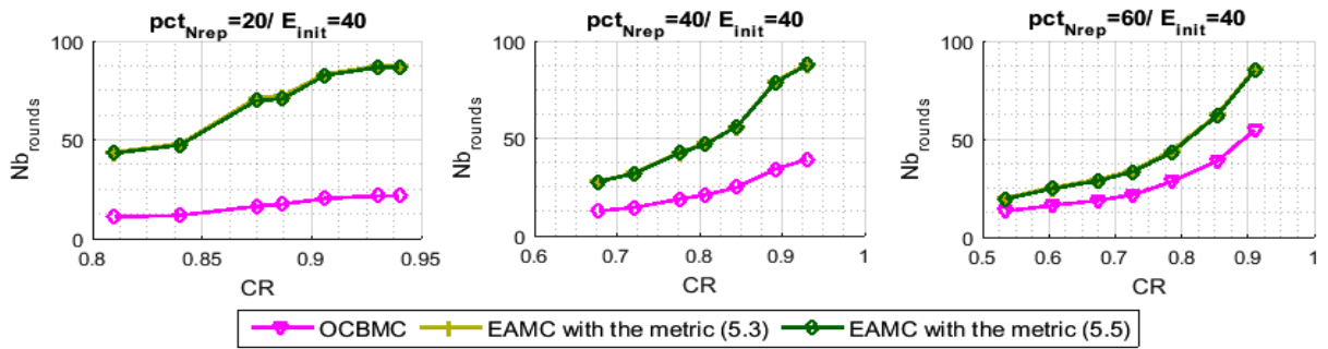
(b) Nb_{rounds} for OCBMC and EAMC approaches.
