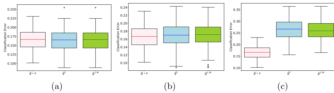
Figure 5.11 – Classification test error of \hat{g} \circ v , \hat{g}^\tau and \hat{g}^{\tau, M} issued from logistic regression (5.6a), random forests (5.6b) and classification trees (5.6c).
