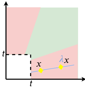
Figure 6.1 – Illustration of an angular classifier g dedicated to extremes \{x, \|x\|_\infty \geq t\} in \mathbb{R}_+^2 . The red and green truncated cones are respectively labeled as +1 and -1 by g .
