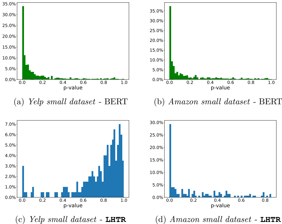
Figure 6.9 – Histograms of the p -values for the non-correlation test between (\Theta(X_i))_{1 \leq i \leq n} and (\|X_i\|)_{1 \leq i \leq n} on embeddings provided by BERT (Figure 6.9a and Figure 6.9b) or LHTR (Figure 6.9c and Figure 6.9d).
