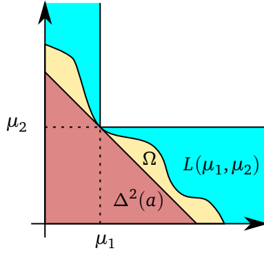
Figure 7.2.: The inclusions \Delta^n(a) \subset \Omega \subset L(\mu_1, \dots, \mu_n) for n = 2
