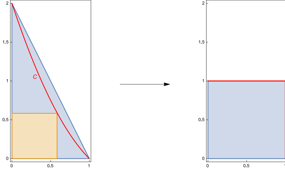
Figure 8.3.: After appropriate rescalings, the map \Phi from Proposition 8.1.1 sends the interior of the ellipsoid E(1, 2) to a product of spheres of area 1, with the preimage of (S^2 \times \{(0, 0, -1)\}) \cup (\{(0, 0, -1)\} \times S^2) contained in \mu^{-1}(C) where C is the red curve at left. Consequently the preimage under \mu of any domain lying below C , such as the small square at left, is embedded into the polydisk P(1, 1)^\circ by a rescaling of (\sigma \times \sigma) \circ \Phi . This gives an explicit knotted embedding P(c, c) \hookrightarrow P(1, 1)^\circ for 1/2 < c < 2 - \sqrt{2} .
