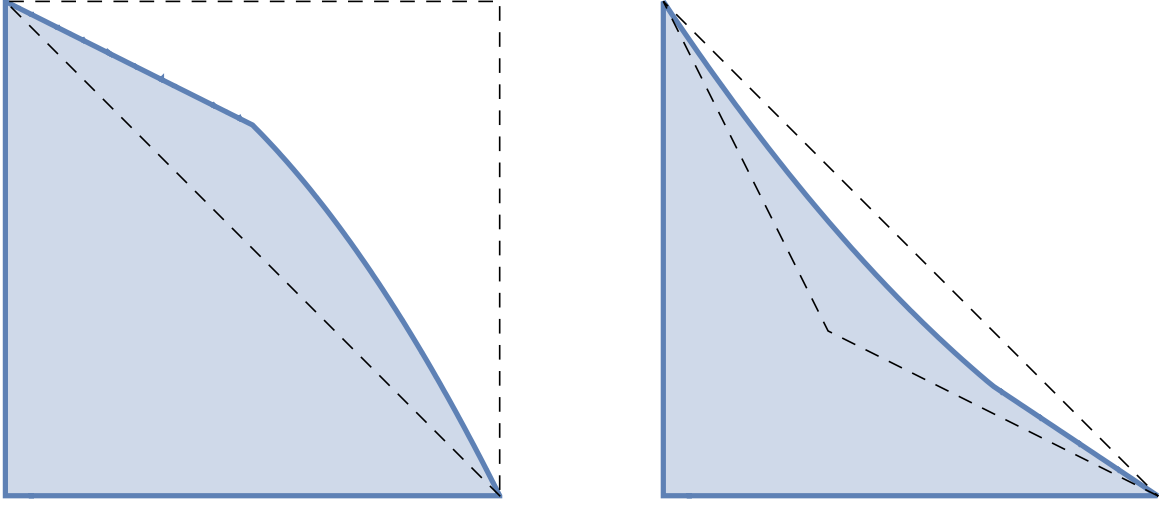
Figure 8.1.: The shaded regions are examples of choices of \Omega such that Theorem 8.0.4 gives knotted embeddings X_\Omega \rightarrow \alpha X_\Omega^\circ for suitable \alpha > 1 . The dashed lines delimit the regions which are assumed to contain (\partial\Omega) \cap (0, \infty)^n in, respectively, Cases (i) and (ii) of the theorem.
