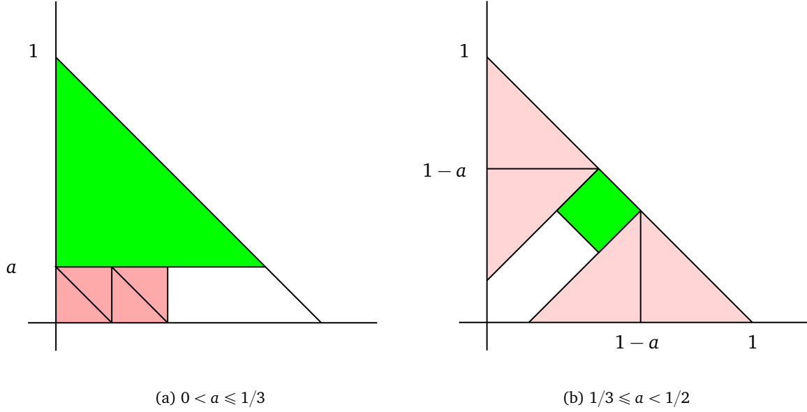
Figure 7.1.: Ball packings
