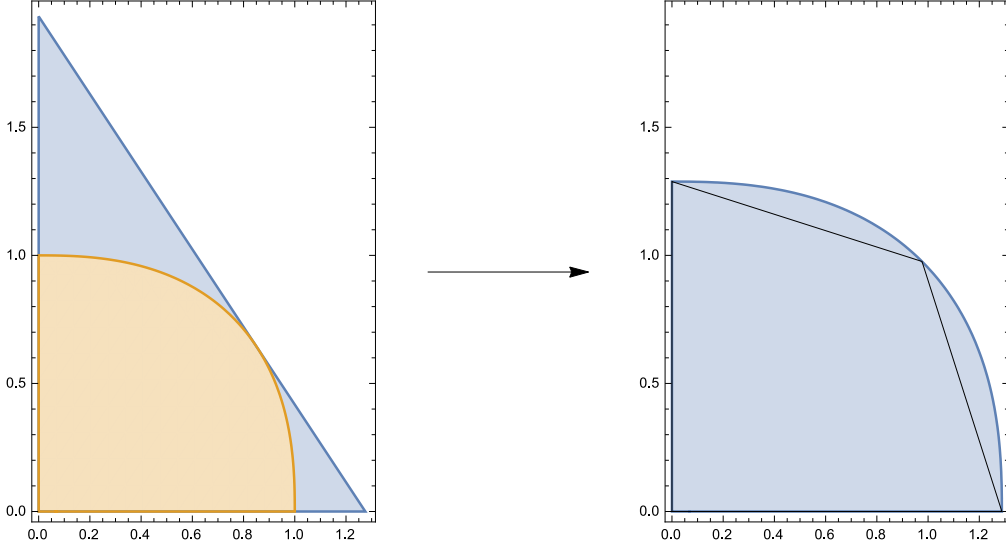
Figure 8.2.: The strategy underlying our knotted embedding in the case that X is the \ell^5 ball of capacity 1, as in Case (i) or (iii) of Theorem 8.0.4 . X is the toric domain associated to the smaller region on the left; the toric domain associated to the triangle on the left is the ellipsoid E = E((3/2)^{3/5}, 3^{3/5}) , which in particular contains X . The larger region at right is obtained by dilating X by \alpha = (1 + \epsilon)(3/2)^{3/5} for a small \epsilon > 0 , and we showed that there is a symplectic embedding \phi: E \rightarrow \alpha X^\circ (in fact, \phi has image contained in the preimage under \mu of the inscribed quadrilateral on the right). Our knotted embedding is \phi|_X ; Theorem 8.0.9(a) implies that any unknotted embedding X \rightarrow \alpha X^\circ that extends to a symplectic embedding E \rightarrow \alpha X^\circ would have \alpha \geq 2^{3/5} , whereas in this construction \alpha can be taken arbitrarily close to (3/2)^{3/5} .
