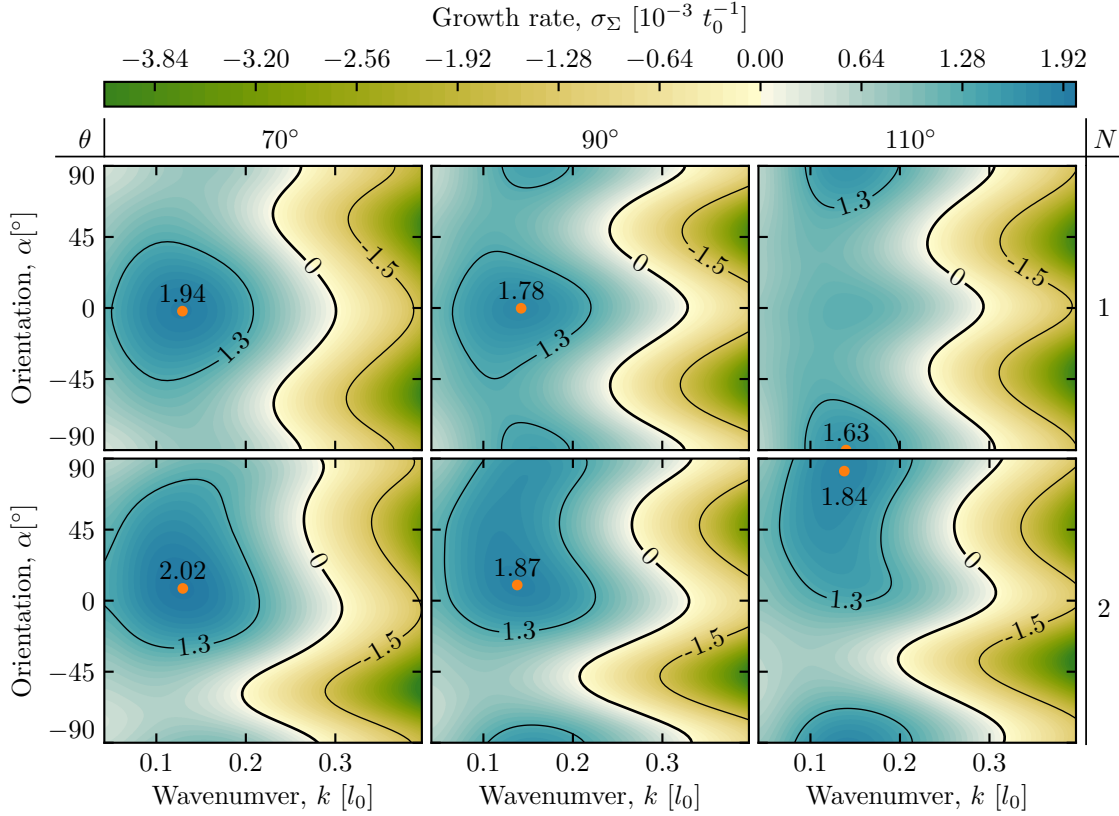
Figure 3.24 – Growth rate \sigma_{\Sigma} in the ReSCAL dune model as a function of the wavenumber k and the orientation \alpha of the bed perturbation for different values of the divergence angle \theta (columns) and the transport ratio N (rows). Orange dots: most unstable mode ( \alpha_{\max}, k_{\max} ) (the corresponding value of \sigma_{\Sigma} has been multiplied by 10^3 for clarity). The signal has been smoothed using a gaussian filter.
