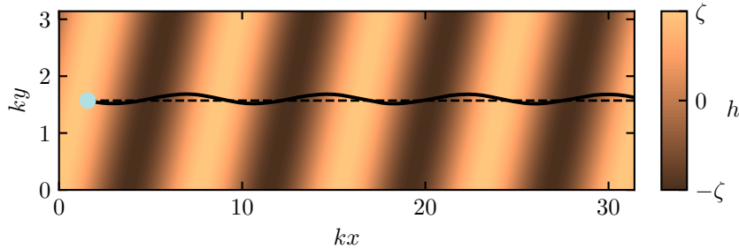
Figure B.1 – Stream line of an inertial flow over a sinusoidal inclined topography at the height of the bed, seen from above. Here, we take k\zeta = 0.25 . The base line is represented in dashes.
