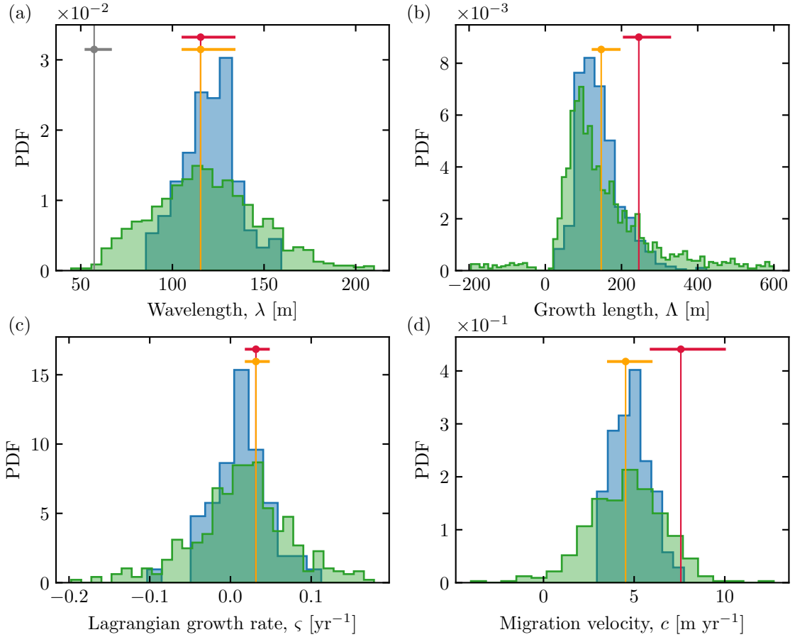
Figure 2.9 – Distributions of incipient dune time and length scales. Blue and green distributions show the results of the global and peak-to-peak methods, respectively. Error bars give the range of values obtained from the spatial linear stability analysis with \mathcal{A} = 3.6 \pm 0.6 and \mathcal{B} = 1.9 \pm 0.3 , and dots show the average. Raw predictions based on a unidirectional wind are in red, and predictions taking into account the correction due to reversing winds are in orange (see table 2.1). The cut-off wavelength \lambda_c is in grey.
