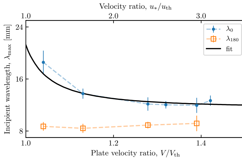
Figure 3.14 – Initial wavelength as a function of the plate velocity ratio for \theta = 0^\circ ( \lambda_0 , blue bullets) and \theta = 180^\circ ( \lambda_{180} , orange squares). Solid line: fit of the linear stability analysis under a unidirectional flow, giving L_{sat} = 0.8 \pm 0.1 mm and C_v = 5 \pm 2
