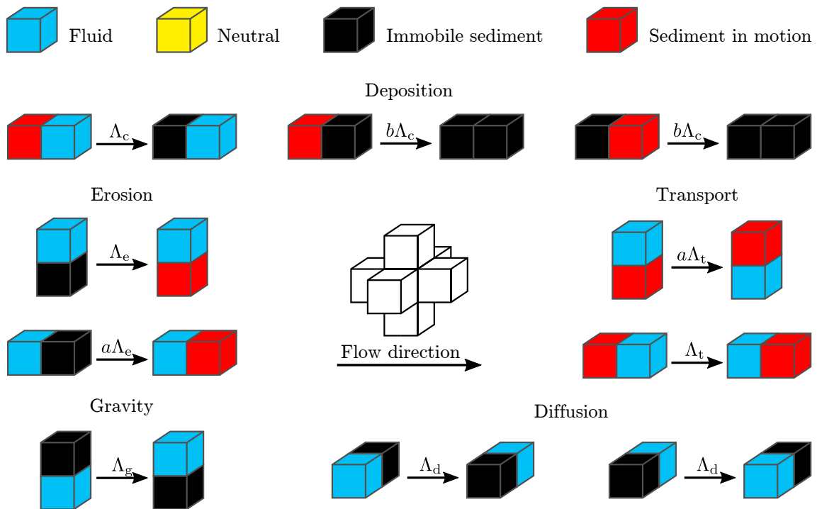
Figure 3.20 – Active transitions in the ReSCAL dune model. The parameters \Lambda_i are transition rates in units of t_0^{-1} . They are constant, except for \Lambda_e that depends on the basal shear stress according to equation (3.59). Here, a and b are positive constants. The central inset shows the direction of the unidirectional flow and the orientation of the nearest neighbors in a regular cubic lattice. Figure from Gao et al. (2015a).
