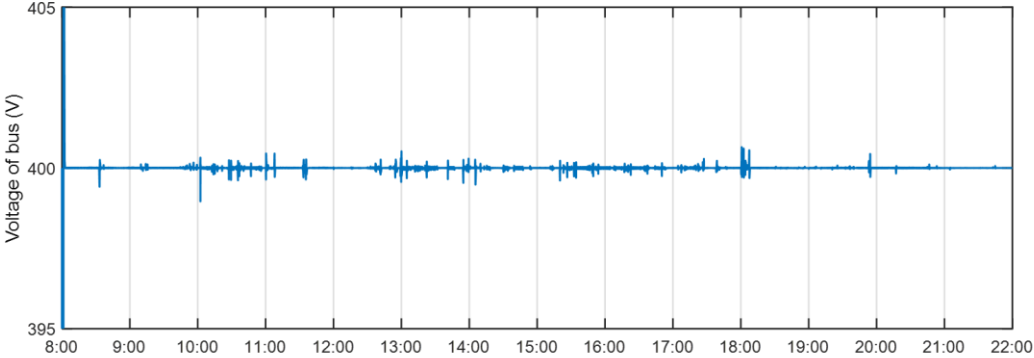
Figure 58. DC bus voltage evolution under SPVA.
