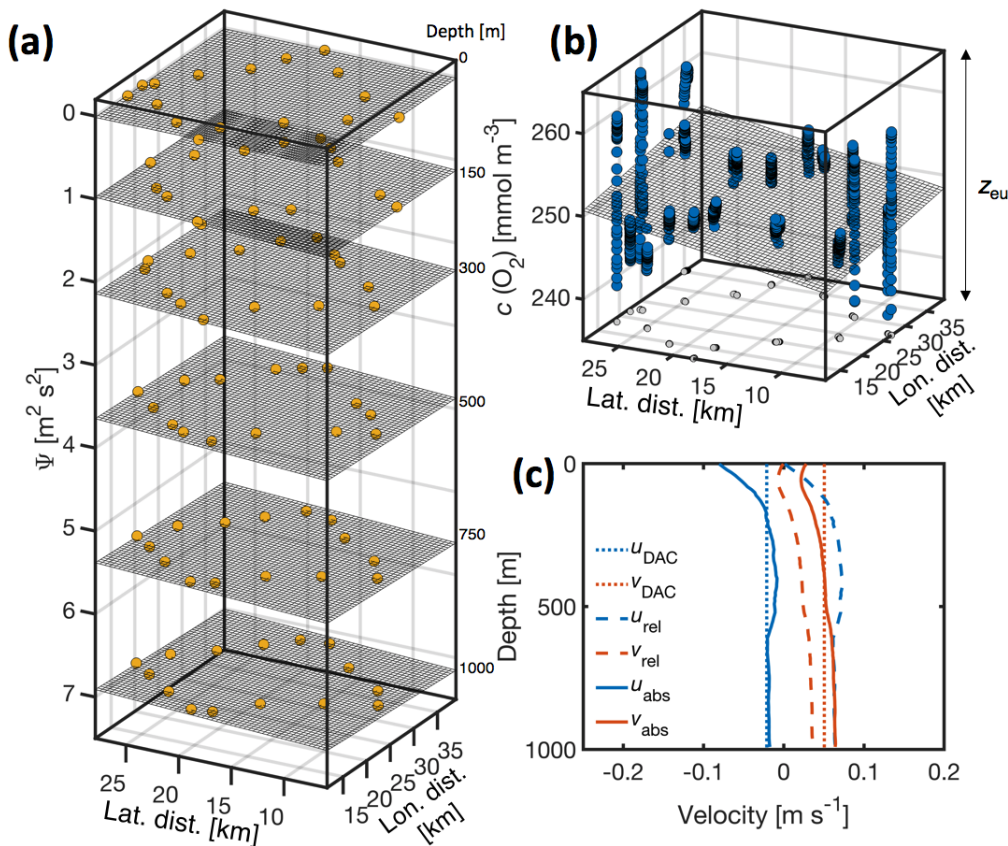
Figure 3.11: (a) Plane-fits of binned geopotential anomalies ( \psi ) at six depths: surface, 150 m, 300 m, 500 m, 750 m and 1000 m. (b) Plane-fit of dissolved oxygen concentrations ( c(\text{O}_2) ) within the euphotic depth ( z_{\text{eu}} ). The grey markers identify the locations of the blue c(\text{O}_2) points. (c) Approximately 5-10 m vertically smoothed relative (dashed line) and absolute (filled line) geostrophic zonal ( u ) and meridional ( v ) velocities. Dive-averaged currents (DACs, dotted line) are displayed for reference. Data shown in (a)-(c) are for March 25.
