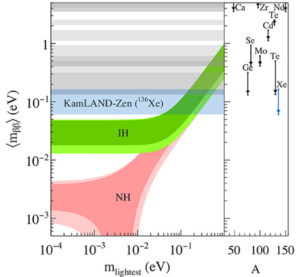
Figure 2.2: The current limits on the m_{\beta\beta} and the allowed regions for both normal and inverse mass ordering.
