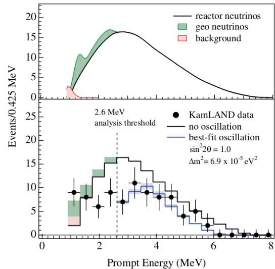
Figure 1.14: The energy spectrum of the neutrinos observed in the KamLAND experiment comparing to the expectations w/o neutrino oscillations. Figure from [43].
