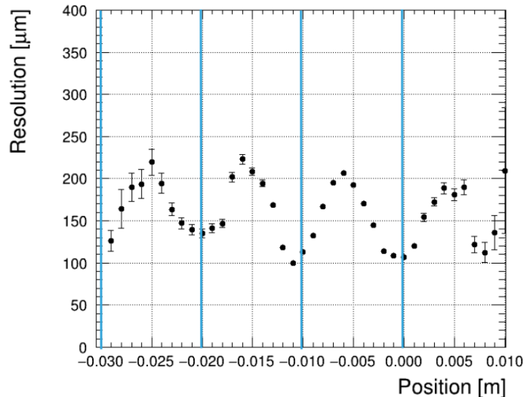
Figure 7.31: The spatial resolution versus the track position in the pad in the particular column. The pad borders are represented with the vertical lines.
