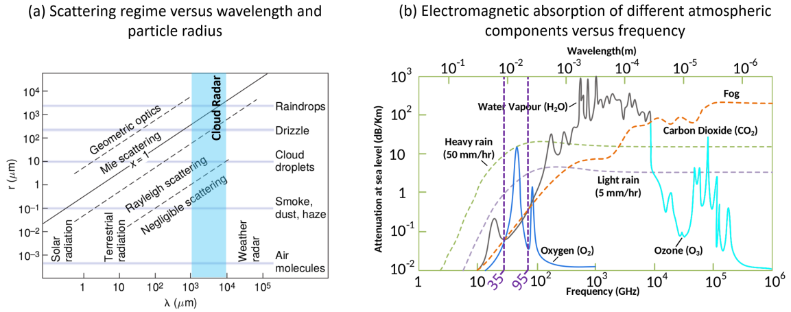
Figure 1.3: (a) Scattering regime depending on wavelength \lambda and particle radius r . Cloud radars usually operate within the wavelengths delimited by the light blue rectangle, where the interaction with cloud droplets is in the Rayleigh Scattering regime. Illustration adapted from Wallace and Hobbs (2006). (b) Electromagnetic absorption of different atmospheric constituents versus frequency. The two most common operating frequencies for cloud radars are indicated by purple dotted lines. Illustration adapted from Britannica (2017).
