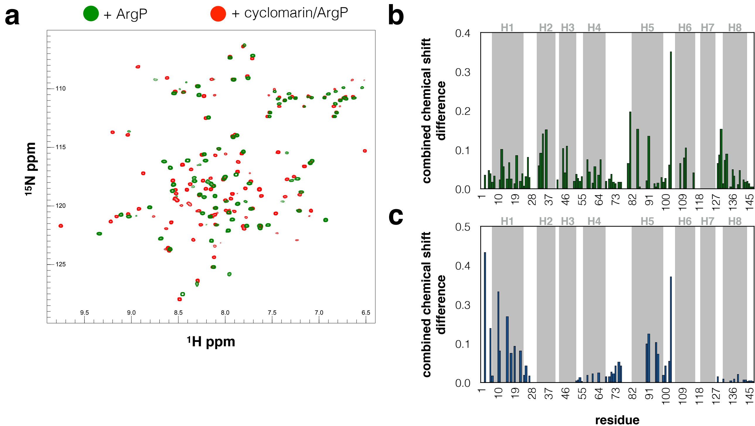
Supporting Figure 6: a) ^1\text{H} - ^{15}\text{N} correlated backbone amide spectrum for ArgP (green) and ArgP/cyclomarin bound NTD (red). b) CSP between cyclomarin bound and cyclomarin/ArgP bound spectrum (for the respective ^1\text{H} - ^{15}\text{N} correlated backbone amide spectra see Fig3c). c) CSP between an ArgP and ArgP/cyclomarin bound NTD spectrum. The CSPs coincide with the binding site of cyclomarin (see Fig2).
