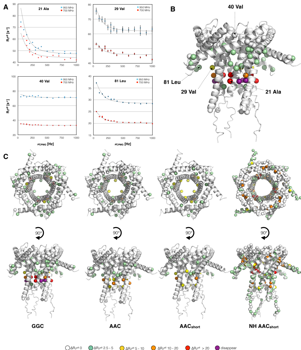
Figure 3.11: CPMG relaxation dispersion of TIM910/substrate complexes. A: CPMG RD curves of four example residues of TIM910 bound to GGC. B: Position of example residues from A on TIM910. C: R_{2,eff} difference of TIM910 in TIM910/substrate samples plotted on the structure. From left to right: TIM910-GGC (ALV methyl groups), TIM910-AAC (ALV methyl groups), TIM910-AAC short (LV methyl groups) and TIM910-AAC short (backbone amides).
