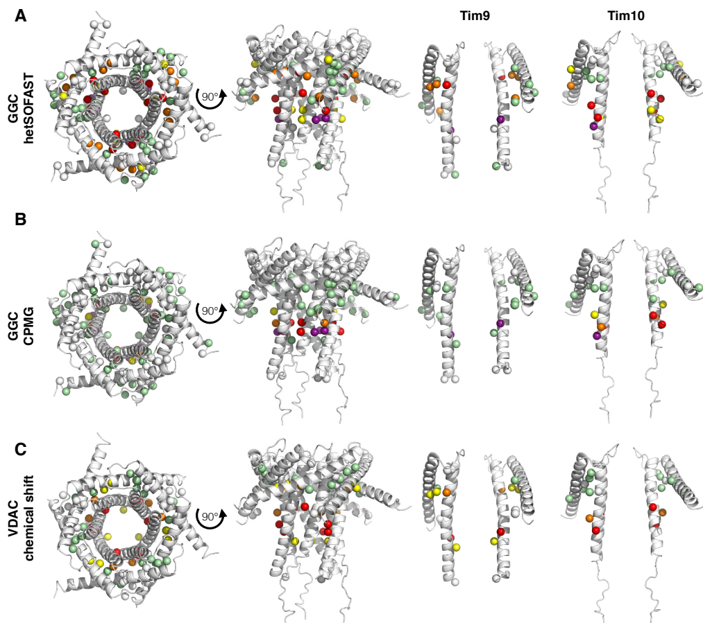
Figure 3.15: Summary of the TIM910 substrate binding site. The substrate binding site is conserved for outer (C) and inner (A/B) membrane substrates. In all three measurements residues in the same area of TIM910 are affected. This region is located between the N- and C-terminal helix on the outside of TIM910.
