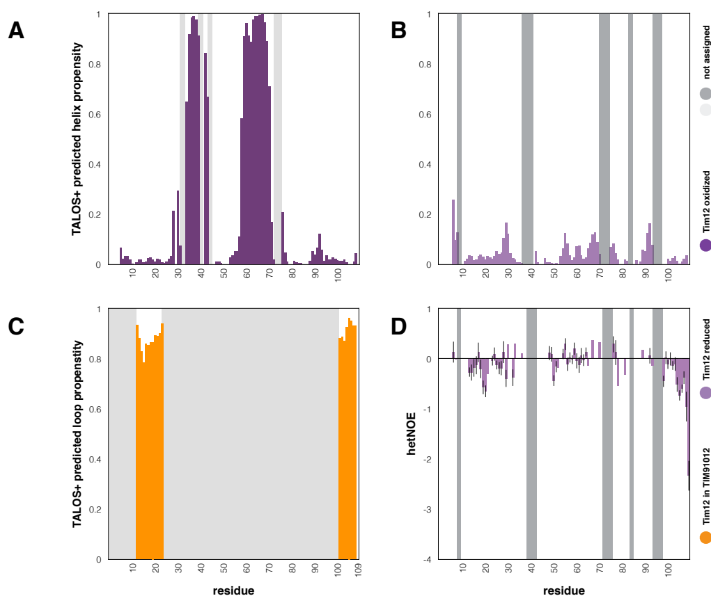
Figure 3.19: Secondary structure of isolated Tim12 and Tim12 in complex with TIM910. A: TALOS+ predicted helix propensity of Tim12 with oxidized twin CX 3 C motif. In light grey part of the sequence that cannot be seen in NMR spectra or residues that were not assigned. B: TALOS+ predicted helix propensity of Tim12 with reduced twin CX 3 C motif. C: TALOS+ predicted loop propensity of assigned residues of Tim12 in a TIM91012 complex. NMR invisible or unassigned parts are shown in grey. As can be seen in the graph, only flexible loop residues of the N- and C-terminus can be detected by NMR. D: hetNOE of Tim12 with reduced twin CX 3 C motif. NMR invisible or unassigned residues are shown in light grey.
