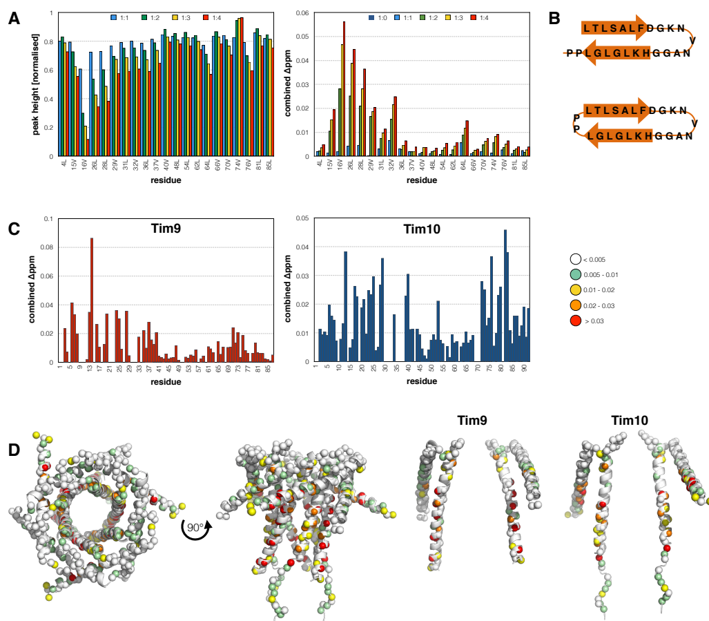
Figure 3.13: Chemical shift/peak height changes of TIM910 spectra upon binding of a cyclic VDAC peptide. A: Peak intensity and chemical shift changes of LV methyl sidechains in TIM910 upon addition of cyclic VDAC peptide. 0.15 mM of methyl labelled TIM910 were mixed with cyclic VDAC and NMR spectra recorded at ratios of TIM910:VDAC 1:1 (blue), 1:2 (green), 1:3 (yellow) and 1:4 (red). B: Sequence of the linear and cyclic VDAC peptide. An arrow indicates the presence of a \beta -strand in the membrane inserted form. C: Chemical shifts in a ^1\text{H} - ^{15}\text{N} correlated TIM910 NMR spectrum upon addition of 1:6 ratio of cyclic VDAC. D: Chemical shift values of C plotted on a TIM910 model.
