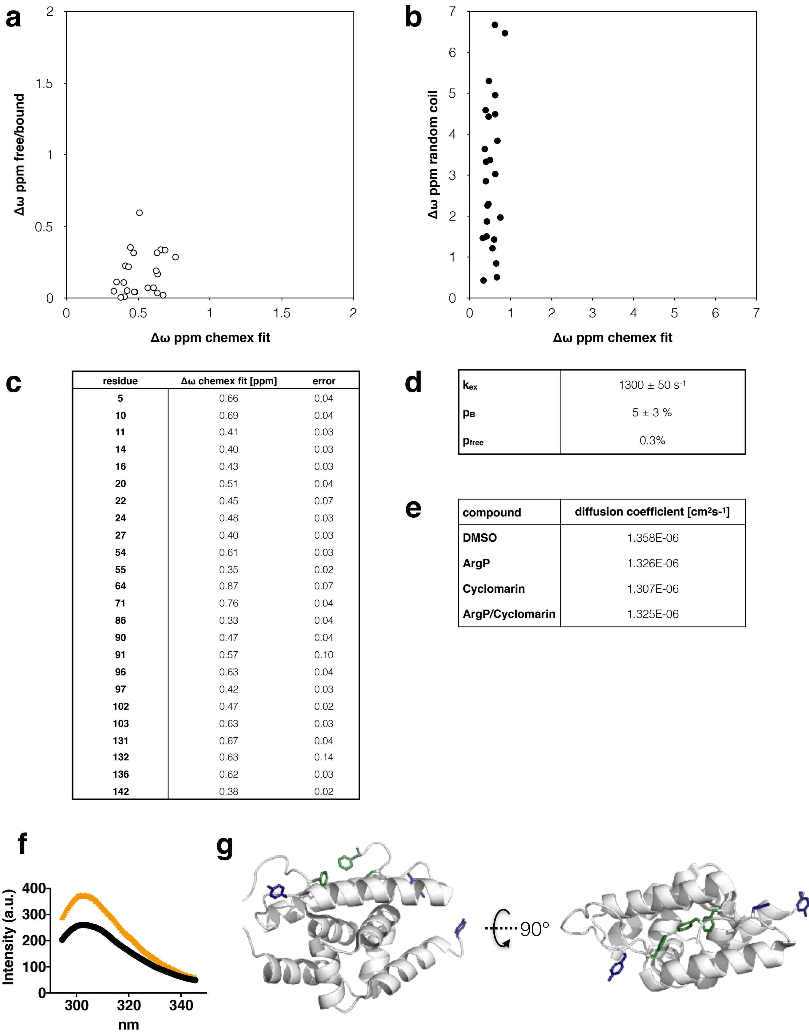
Supporting figure 5: a) Correlation between the theoretical chemical shift differences of the excited state derived from fitting of the CPMG RD data and experimental chemical shift differences between apo and bound state. b) Correlation between the chemical shift differences derived from Chemex fits of the CPMG RD data and chemical shift differences between the folded NTD and calculated random coil shifts derived from nclDP. c) Table of chemical shift differences of all fitted residues from Chemex CPMG RD data fit. d) Parameters of the Chemex CPMG RD fit. e) Diffusion coefficients of MtbClpC1 NTD in the presence of different ligands, derived from diffusion ordered spectroscopy (DOSY) NMR measurements. f) Intrinsic fluorescence spectrum of apo (black) and ArgP bound MtbClpC1 NTD (orange). g) Aromatic residues distribution in MtbClpC1 NTD - tyrosine side chains in blue, phenylalanine side chains in green.
