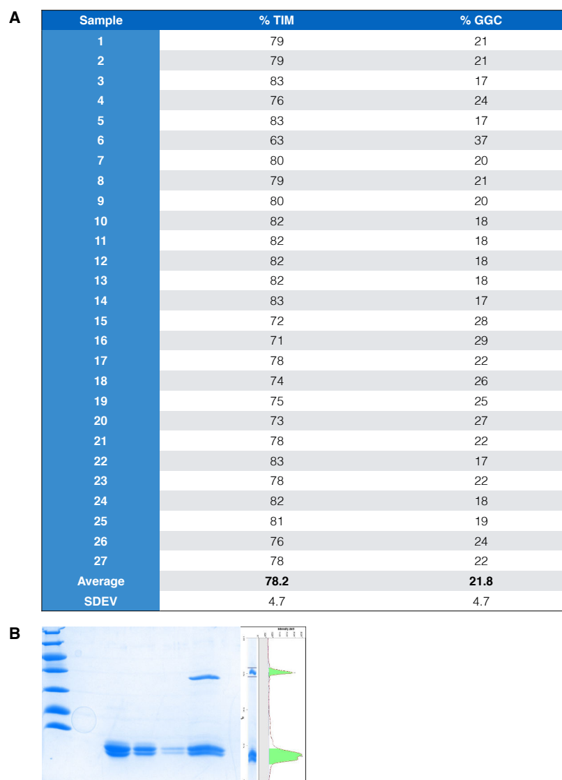
Figure A.2: SDS-PAGE statistics for TIM910-GGC stoichiometry. A: Average ratios of the integrated bands of 27 TIM910-GGC samples. B: Example peak integration of a TIM910-GGC SDS PAGE sample.
