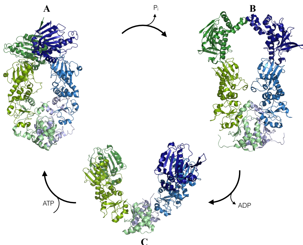
Figure 1.3: X-ray structures of the Hsp90 ATP, ADP and nucleotide free states. Hsp90 in its ATP bound closed state (A, PDB: 2CG9), in the compact ADP state (B, PDB: 2IOP) and the open nucleotide free state (C, PDB: 2IOQ). The NTDs are shown in dark blue/green, the MDs in middle blue/green and the CTDs in light blue/green.
