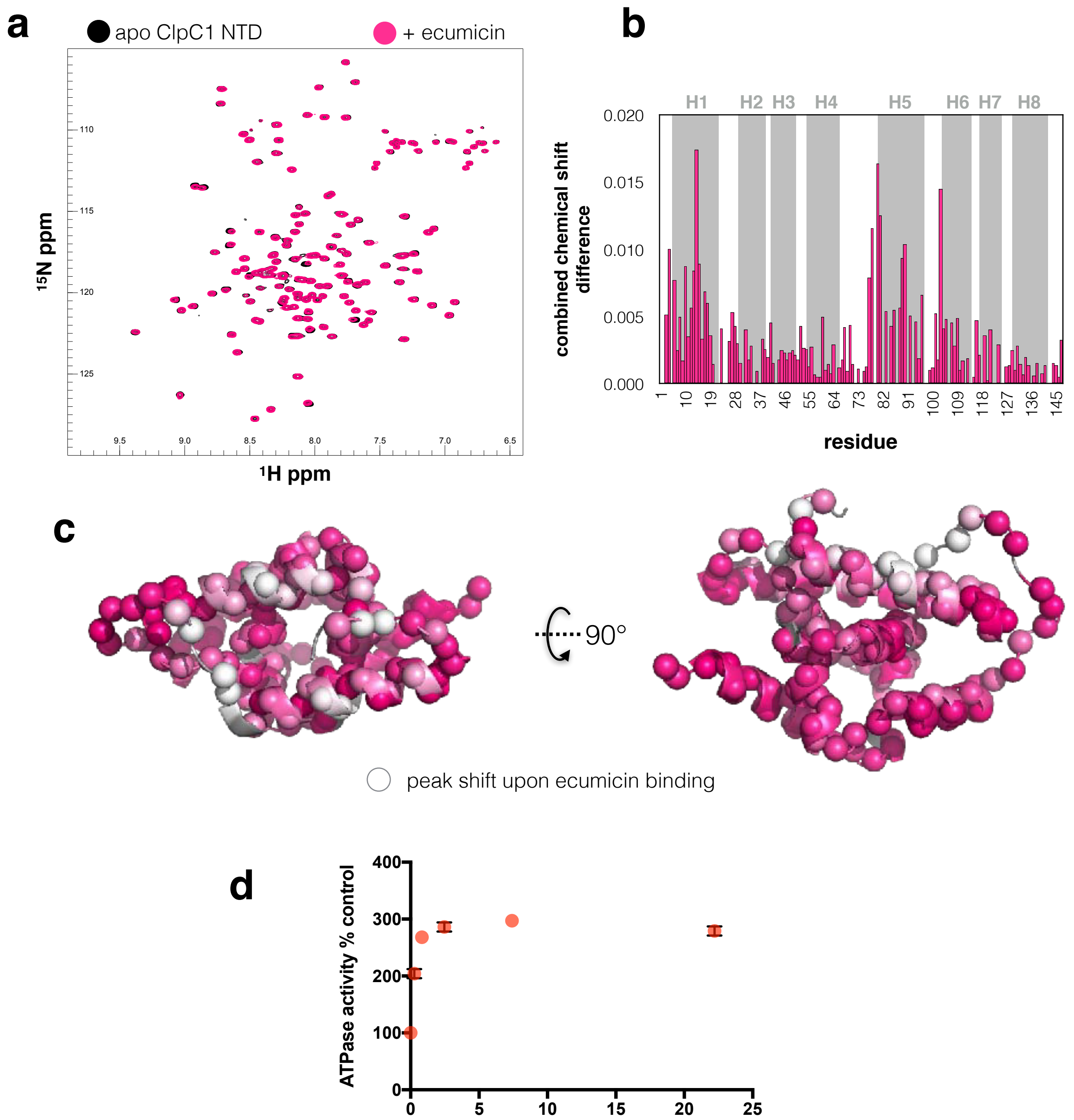
Supporting Figure 2: Ecumicin binding results in only modest changes in the backbone spectra of Mtb ClpC1 NTD compared with cyclomarin (see Fig2a). a) ^1\text{H} - ^{15}\text{N} correlated backbone amide spectrum for apo (black) and ecumicin-bound (pink) Mtb ClpC1 NTD. b) CSP induced by ecumicin, compare with Fig2c for cyclomarin induced CSP. c) Ecumicin induced CSP are mapped onto the NTD structure. d) Ecumicin is able to activate Mtb ClpC1 ATPase activity. Results expressed as a ratio to the control experiment.
