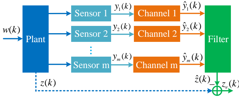
Figure 4-1 Filtering problem setup
