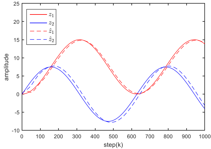
Figure 6-6 Filtering performance
