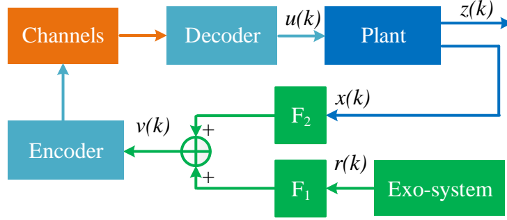
Figure 3-1 System setup
