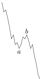
Figure 1.1: Potential with a trap between a and b
