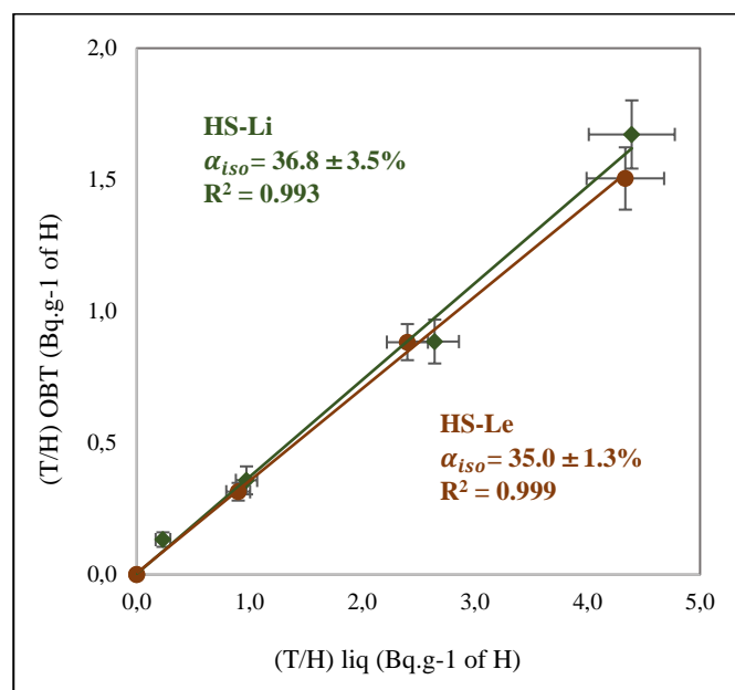
Fig. 3: (T/H) of HS-Li and HS-Le at the steady state after freeze-drying versus measured set (T/H) of saline solutions with the associated exchangeable hydrogen pool ( \alpha_{iso} ) parameter. Note the accurate values of the ( \alpha_{iso} ) parameter of 36.8 and 35.0 (SD = 3.5% and 1.3%, R^2 = 0.993 and 0.999, respectively) are obtained for HS-Li and HS-Le, respectively. SD = standard deviation.
