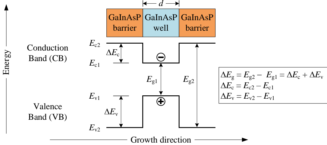
Fig. 2.5. Schematic diagram of a GaInAsP quantum-well and its bandgap profile.
