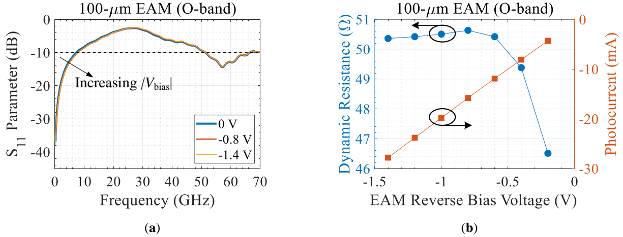
Fig. 3.35. (a) S_{11} parameter of the driving circuit of the 100- \mu\text{m} long O-band EAM, (b) effective resistance of the circuit as a function of reverse bias voltage.
