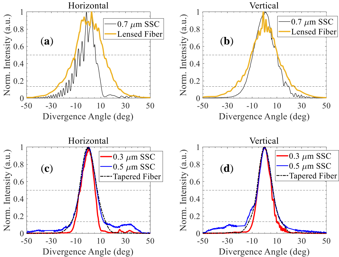
Fig. 3.10. Measured far-field intensity profiles of (a), (b) 0.7- \mu\text{m} SSC and a lensed fiber, (c), (d) 0.3- \mu\text{m} SSC, 0.5- \mu\text{m} SSCs and a commercial tapered fiber in the horizontal (left) and vertical (right) directions.
