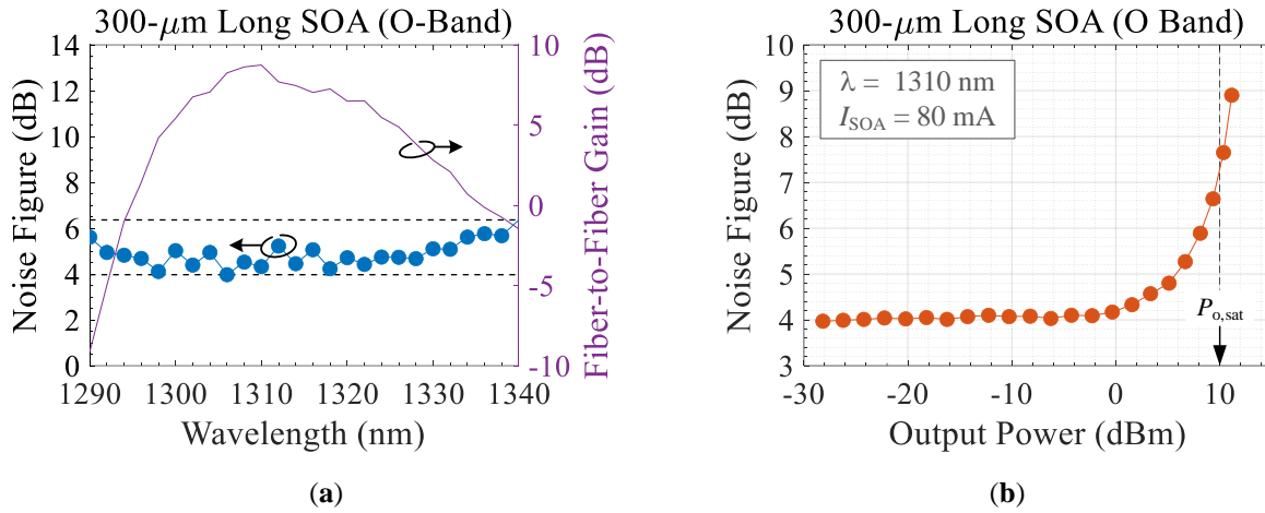
Fig. 3.25. Noise figure of the 300- \mu\text{m} long O-band SOA in a reflective configuration as a function of (a) wavelength of the input light ( P_{\text{in}} = -15 dBm), (b) output power ( \lambda = 1310 nm, I_{\text{SOA}} = 80 mA, T = 25^\circ\text{C} ).
