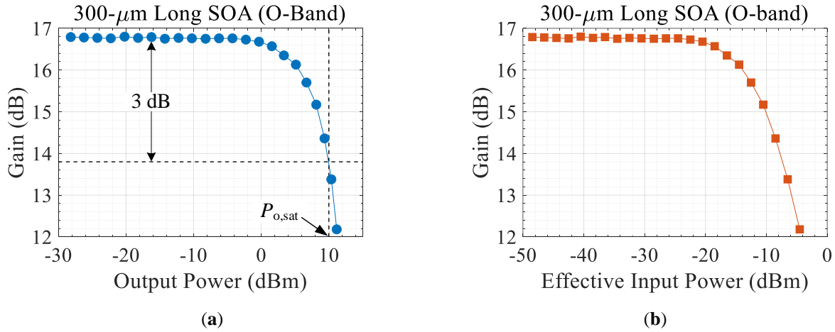
Fig. 3.20. Signal gain of a 300- \mu\text{m} long O-band SOA in a reflective configuration as a function of (a) output power, (b) effective input power. \lambda = 1310 nm, I_{SOA} = 80 mA, T = 25^\circ\text{C} .
