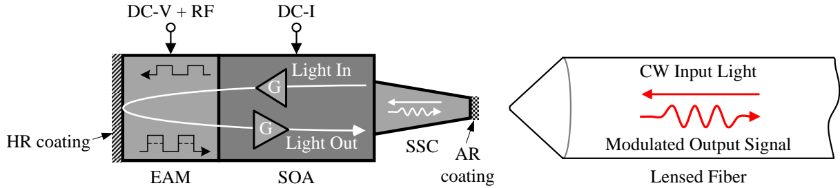
Fig. 2.32. Schematic diagram of an REAM-SOA PIC with integrated SSC. A lensed fiber is used for coupling light to and from the PIC.
