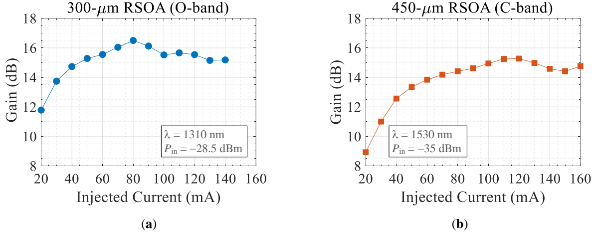
Fig. 3.17. Signal gain as a function of SOA pump current: (a) 300-μm long O-band SOA operating at 1310 nm (effective P_{\text{in}} = -28.5 \text{ dBm} ), (b) 450-μm long C-band SOA operating at 1530 nm ( P_{\text{in}} = -35 \text{ dBm} ). T = 25^\circ\text{C} . Both SOAs are in a reflective configuration.
