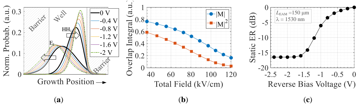
Fig. 2.18. (a) Simulated evolution of electron and hole wave functions with applied reverse bias voltage (field) and (b) their overlap integrals ( M and M^2 ) as a function of applied field, (c) static extinction ratio of a 150-μm long REAM at 1530 nm and 25°C.
