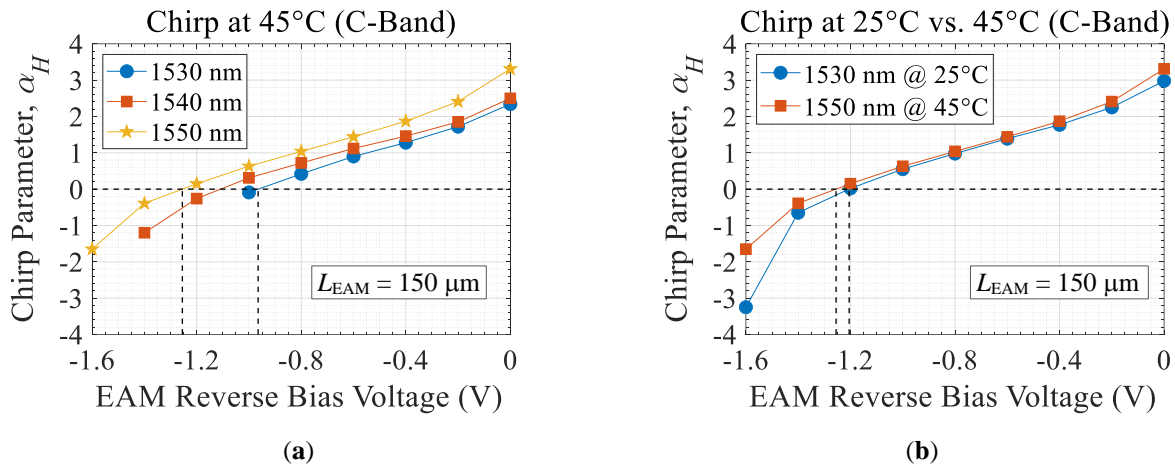
Fig. 3.48. (a) Small-signal chirp parameter of the 150\text{ }\mu\text{m} long EAM as a function of reverse bias voltage at 45^\circ\text{C} for different input wavelengths, (b) comparison of chirp performances at 25^\circ\text{C} and 45^\circ\text{C} .
