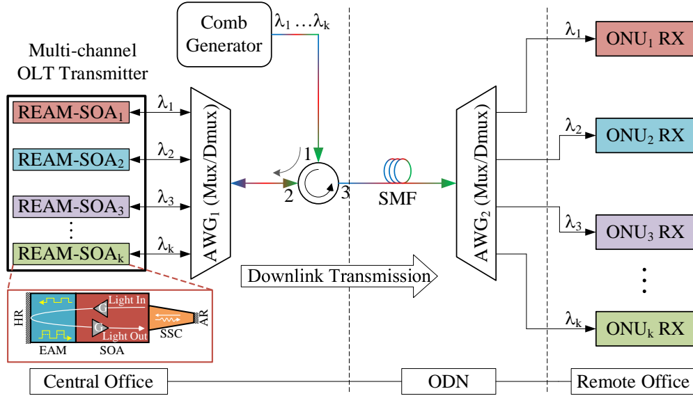
Fig. 1.6. Schematic diagram of a WDM-PON based on array of REAM-SOAs for downlink transmission. Inset: schematic of an REAM-SOA with an integrated spot-size converter.
