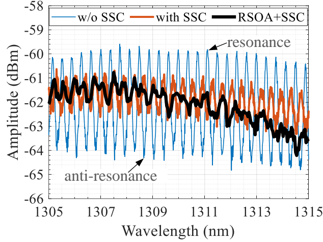
Fig. 3.3. ASE ripple in a single-pass (transmittive) Fabry-Perot cavity with and without a tilted output waveguide, and a double-pass (reflective) SOA with an integrated SSC.
