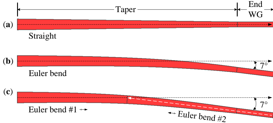
Fig. 3.4. Tapers with and without a bend: (a) straight taper, (b) taper with a single clothoid curve, and (c) taper with double clothoid curves.
