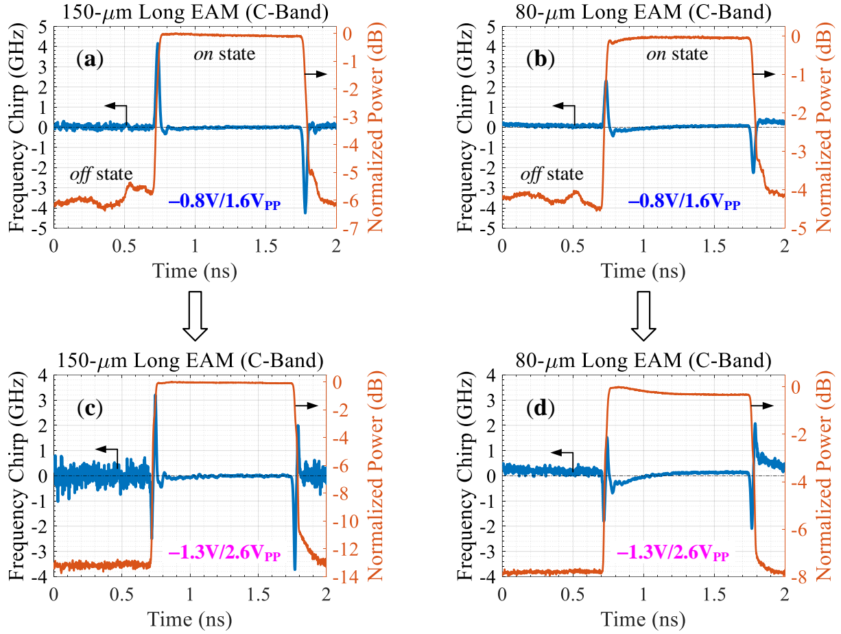
Fig. 3.49. Time-resolved frequency chirp induced by (a), (c) 150- \mu\text{m} EAM ( I_{\text{SOA}} = 90 mA), (b), (d) 80- \mu\text{m} EAM ( I_{\text{SOA}} = 120 mA) under large-signal operating condition. The top figures are obtained at -0.8 V/1.6 V PP whereas the bottom ones are at -1.3 V/2.6 V PP . \lambda = 1545 nm, T = 25^\circ\text{C} . Both PICs are in an REAM-SOA configuration.
