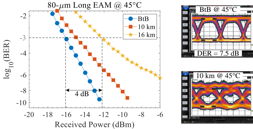
Fig. 4.6. BER performance of an 80- \mu\text{m} long EAM in an REAM-SOA configuration at 45^\circ\text{C} and 1545 nm ( -1.3 \text{ V}/2.6 \text{ V}_{\text{PP}} ). I_{\text{SOA}} = 120 \text{ mA} . [Inset: unfiltered 25G NRZ eye diagrams in BtB (top) and after 10 km (bottom).]
