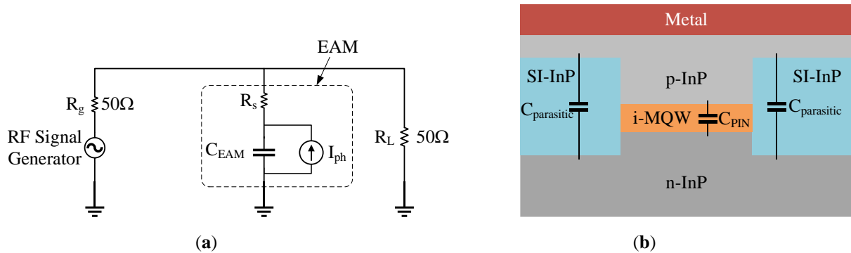
Fig. 3.32. (a) Equivalent circuit model of an EAM as a lumped element, (b) schematic illustration of modulator capacitances due to reverse biased PIN junction as well as parasitic contributions (pad capacitance not shown).
