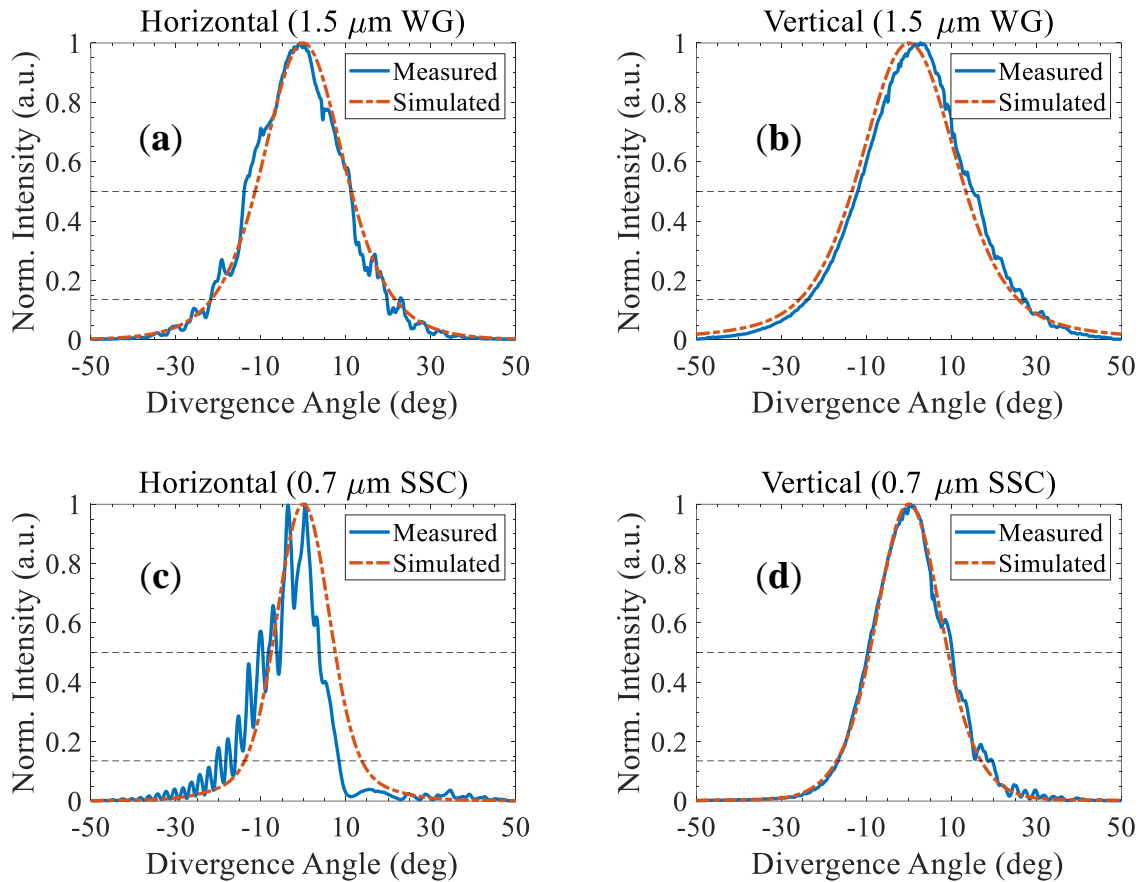
Fig. 3.9. Simulated and measured far-field intensity distributions of (a), (b) 1.5 \mu\text{m} (straight output waveguide without a taper), (c), (d) 0.7 \mu\text{m} waveguide ( 7^\circ -tilted output waveguide) in the horizontal (left) and vertical (right) directions.
