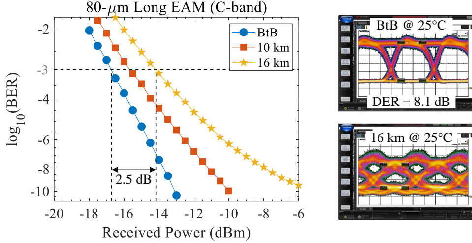
Fig. 4.5. BER performances of an 80- \mu\text{m} long EAM in an REAM-SOA configuration at 1530 nm ( -1.1 \text{ V}/2.2 \text{ V}_{\text{PP}} ). T = 25^\circ\text{C} . I_{\text{SOA}} = 120 \text{ mA} . [Inset: 25 Gb/s NRZ eye diagrams in BtB (top) and after 16 km (bottom).]
