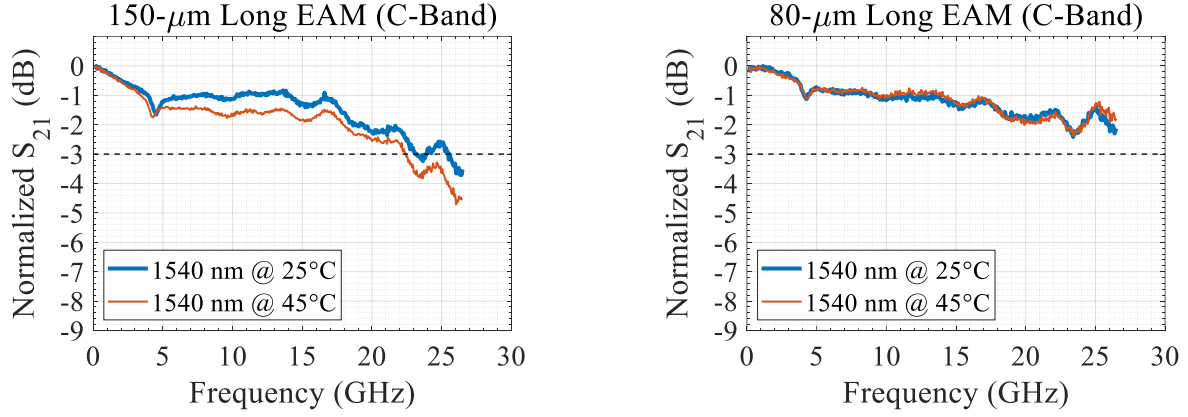
Fig. 3.37. Comparison of S_{21} parameters at 25°C vs. 45°C for (a) 150- \mu\text{m} long EAM, (b) 80- \mu\text{m} long EAM. Both PICs are in an REAM-SOA configuration. V_B = -1 V to -1.2 V, P_{in} \approx 0 dBm, I_{SOA} = 90 mA for (a) and 120 mA for (b).
