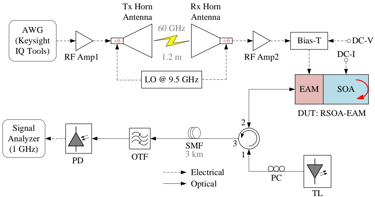
Fig. 4.16. Schematic diagram of experimental setup for a multichannel V-band/IFoF uplink transmission.
