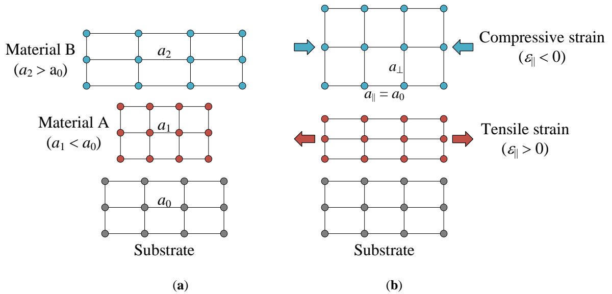
Fig. 2.10. Illustration of two types of materials, one with a larger lattice constant and another with smaller lattice constant than the substrate in their (a) unstrained states, (b) strained states (after [54]).
