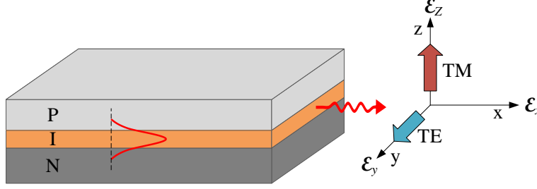
Fig. 2.14. Schematic of light propagating either in TE or TM mode (after [52]).
