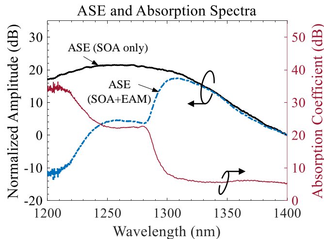
Fig. 3.15. ASE spectra of an O-band RSOA as a standalone element and in an integrated circuit in an RSOA-EAM configuration together with the EAM's absorption spectrum. The ASE amplitudes are normalized to 1400 nm.
