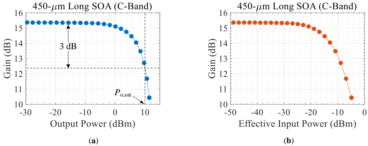
Fig. 3.22. Signal gain of a 450- \mu\text{m} long C-band SOA in a reflective configuration as a function of (a) output power, (b) effective input power. \lambda = 1530 nm, I_{SOA} = 120 mA, T = 25^\circ\text{C} .
