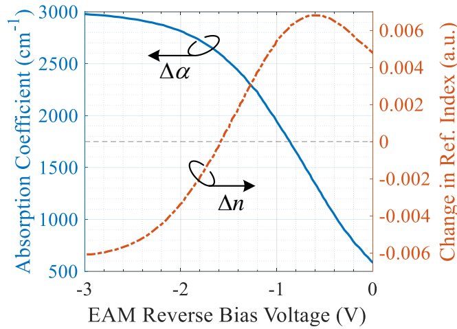
Fig. 3.42. Calculated changes in absorption coefficient (left y-axis) and refractive index (right y-axis) as a function of reverse bias voltage of an EAM (after [98]).
