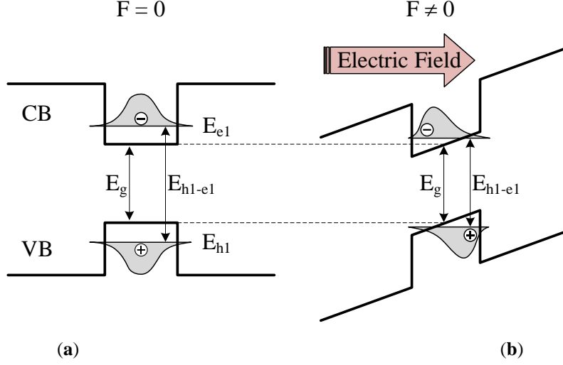
Fig. 2.15. Schematic illustration of bandgap profile and wave functions of ground state electrons and holes inside a QW (a) without and (b) with externally applied electric field.
