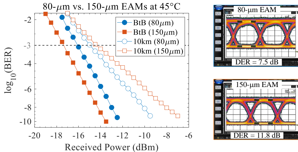
Fig. 4.7. BER performances of 80- \mu\text{m} and 150- \mu\text{m} long EAMs in an REAM-SOA configuration at 25 Gb/s NRZ and 45°C for an input wavelength of 1545 nm ( -1.3 V/ 2.6 V PP ). I_{\text{SOA}} = 90 mA for the PIC based on a longer EAM and 120 mA for the one based on a shorter EAM. [Inset: 25G NRZ BtB eye diagrams obtained from the 80- \mu\text{m} long EAM (top) and the 150- \mu\text{m} long EAM (bottom).]
