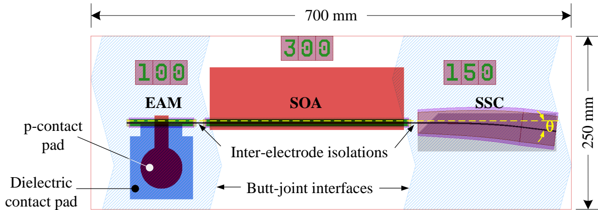
Fig. 2.37. Mask layout of a reflective EAM-SOA PIC with integrated SSC using butt-joint integration technique.
