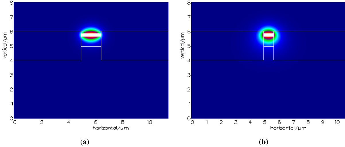
Fig. 2.29. Simulated mode profiles of SI-BH waveguides of (a) 1.5 \mu\text{m} and (b) 0.7 \mu\text{m} ridge widths.
