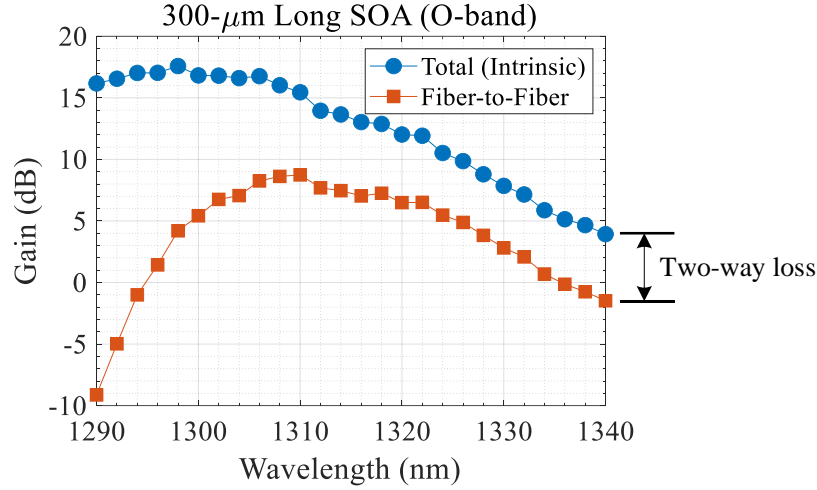
Fig. 3.18. Intrinsic and fiber-to-fiber gain spectra of a 300- \mu\text{m} long RSOA. I_{\text{SOA}} = 60 \text{ mA} , P_{\text{in}} = -28.5 \text{ dBm} , T = 25^\circ\text{C} .
