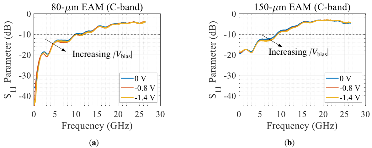
Fig. 3.34. Reflection ( S_{11} ) parameters of the driving circuits of (a) 80- \mu\text{m} long and (b) 150- \mu\text{m} long C-band EAMs.
