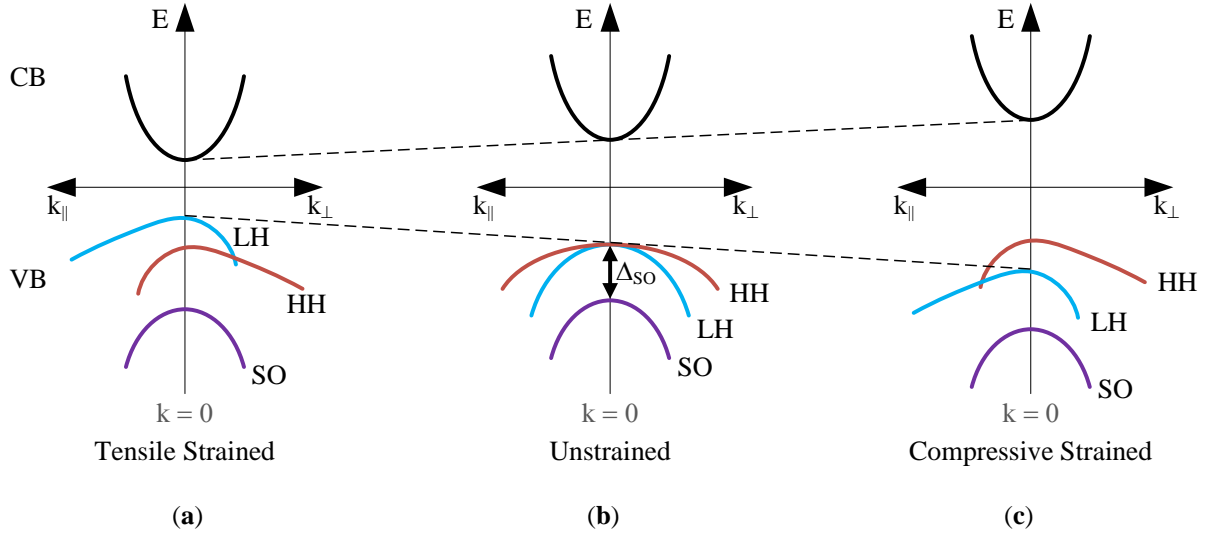
Fig. 2.11. Illustration of electronic band structures of (a) tensile strained, (b) unstrained, and (c) compressive strained bulk-like direct bandgap material. k_{\perp} is the wave vector along the growth ( z ) axis whereas k_{\parallel} is the in-plane ( xy ) wave vector (after [18]).
