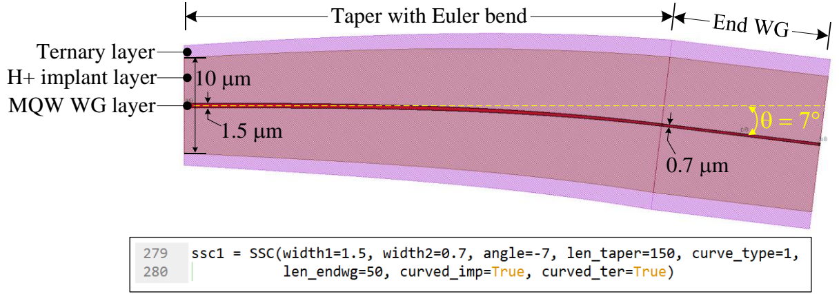
Fig. 2.36. Mask layout of a 7°-tilted SSC running from 1.5 μm to 0.7 μm with its epitaxial layers created using Nazca. Inset: excerpt of the code for creating the PCell object.
