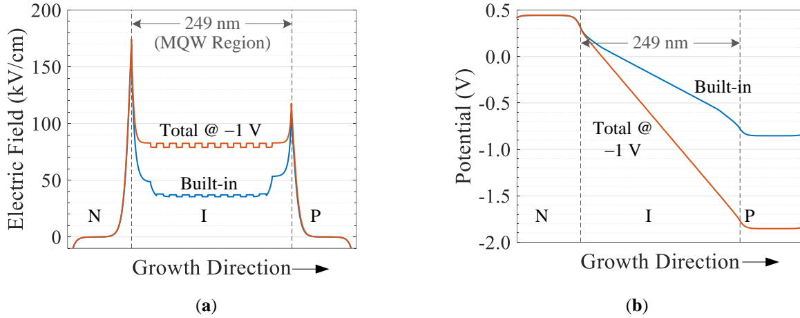
Fig. 2.16. (a) Simulated electric field distribution inside a GaInAsP MQW structure with and without applying an external field perpendicular to the QW layers, (b) total voltage drop across the MQW structure.
