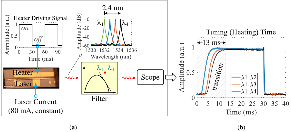
Fig. 1.4. (a) SEM image of a DML with integrated heater, and shape of the heater driving signal applied to tune the laser by 2.4 nm ( 4 \times 100 \text{ GHz} ), (b) signal captured by a sampling oscilloscope after the CW light passes through a tunable optical filter. \lambda_1 = 1532 \text{ nm} , \lambda_2 = 1532.8 \text{ nm} , \lambda_3 = 1533.6 \text{ nm} , \lambda_4 = 1534.4 \text{ nm} , V_{\text{scope}} \propto 1/f .
