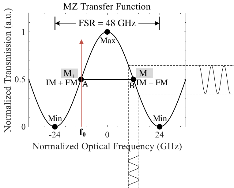
Fig. 3.43. Schematic illustration of the transfer function of a Mach-Zehnder interferometer and the control points for chirp measurement.
