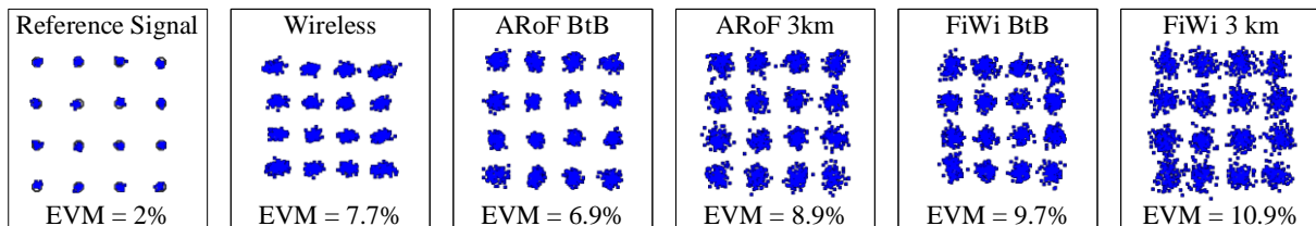
Fig. 4.19. Constellation diagrams of worst-performing channels, and measured EVMs of the corresponding subcarriers at different stages of the transmission system.
