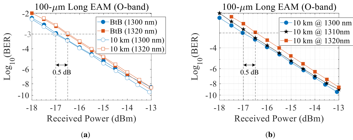
Fig. 4.9. BER performance of a 100-μm long EAM in an REAM-SOA configuration (a) at 1300 nm ( -1 \text{ V}/2 \text{ V}_{\text{PP}} ) and 1320 nm ( -1.4 \text{ V}/2.8 \text{ V}_{\text{PP}} ) nm in BtB and after 10 km, (b) 10-km BER performances with an intermediate wavelength of 1310 nm between the two extrema (i.e., 1300, 1310, and 1320 nm). T = 25^\circ\text{C} , I_{\text{SOA}} = 40 \text{ mA} .
