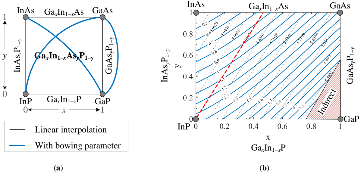
Fig. 2.3. (a) Schematic illustration of bandgaps with and without bowing parameter for GaInAsP (after [47]) [straight lines: linear interpolation, curved lines: with bowing parameter], (b) composition diagram of GaInAsP [solid lines: bandgap energies in eV, dashed lines: lattice constants in Å, hatched region: GaInAsP becomes indirect bandgap].
