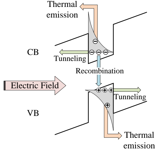
Fig. 2.23. Schematic of carrier escape mechanisms under the influence of an externally applied field (after [58]).
