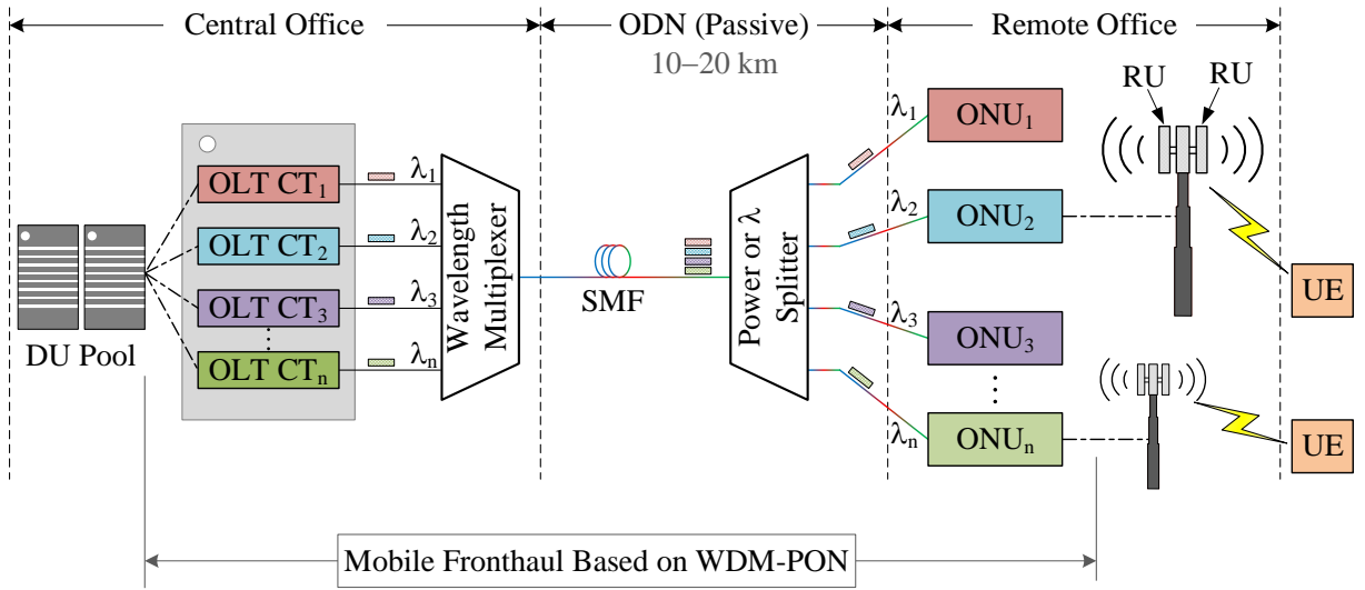
Fig. 1.1. Schematic diagram of a WDM-PON system supporting 5G fronthauling in a C-RAN architecture. CT: channel termination, SMF: single-mode fiber.
