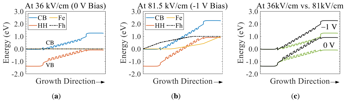
Fig. 2.17. Simulated band edge profiles of compressive strained GaInAsP MQW structure on an InP substrate (a) without applied field (at 0 V, 36 kV/cm built-in field), (b) with applied field ( -1 V, 81.5 kV/cm total field), and (c) comparison of the band structures with and without external DC field.
