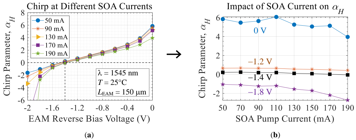
Fig. 3.47. Small-signal chirp parameter of a 150 \mu\text{m} long EAM (a) as a function reverse bias voltages at different SOA currents, (b) as a function of SOA pump current for different EAM reverse bias voltages. \lambda = 1545\text{nm} .
