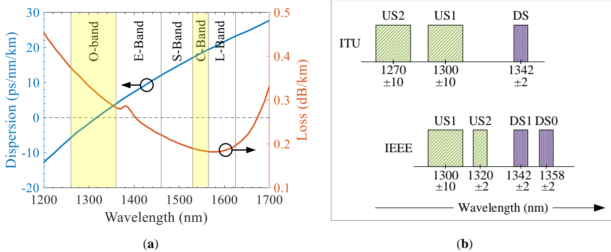
Fig. 1.3. (a) Dispersion and loss spectra of standard single-mode fiber, (b) wavelength plans for 50G PON applications defined by ITU's 50G PON (top) and IEEE's 50G EPON (bottom). US: upstream, DS: downstream.
