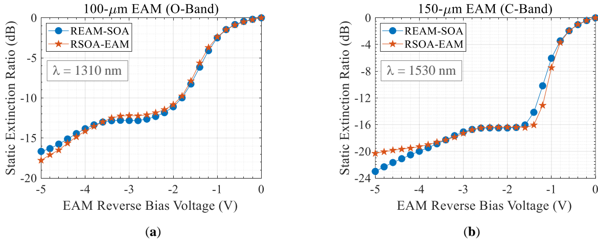
Fig. 3.31. Comparison of static extinction ratios of REAM-SOA and RSOA-EAM configurations for (a) 100- \mu\text{m} long O-band EAM at 1310 nm, (b) 150- \mu\text{m} long C-band EAM at 1530 nm.
