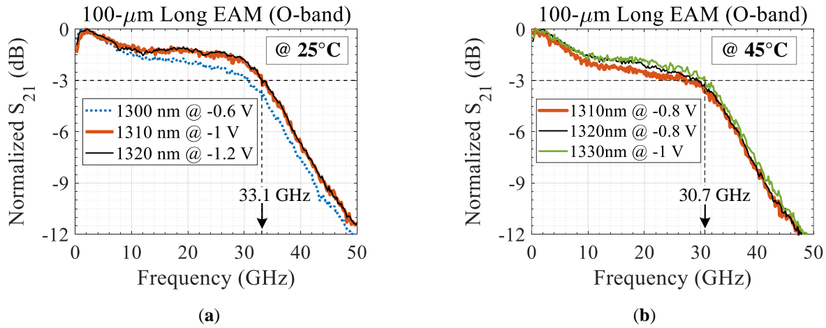
Fig. 3.39. Small-signal frequency response ( S_{21} parameter) of a 100- \mu\text{m} long O-band EAM for different input wavelengths, operating at (a) 25°C, (b) 45°C. P_{\text{in}} = 0 dBm, I_{\text{SOA}} = 40 mA.
