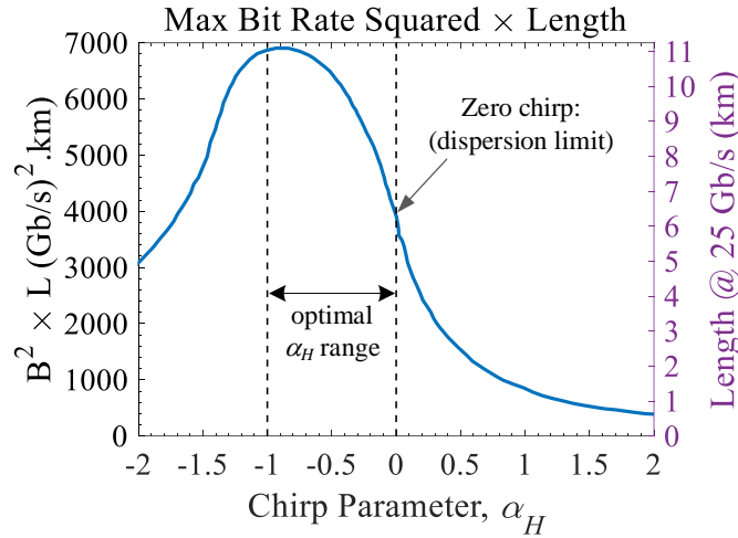
Fig. 3.51. Bandwidth squared-distance product of a standard SMF at 1550 nm (17 ps/nm/km dispersion) using NRZ modulation format and estimated fiber length for 25 Gb/s transmission (after [104]).
