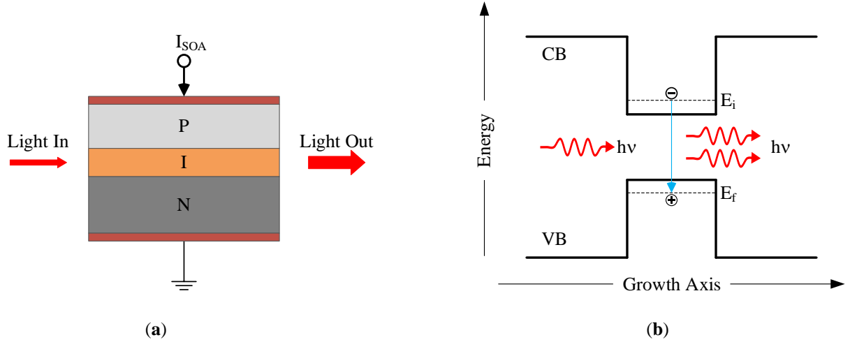
Fig. 2.24. Schematic diagram of (a) an SOA, and (b) the process of light amplification through stimulated emission.
