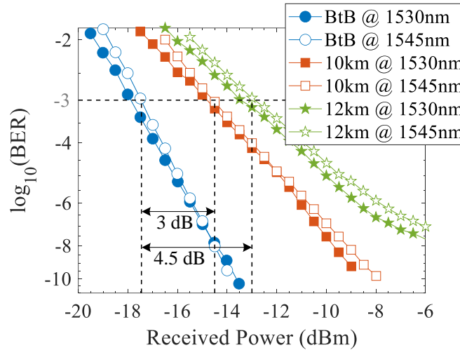
Fig. 4.3. BER performance of a 150- \mu\text{m} long EAM in an REAM-SOA configuration operating at 25 Gb/s NRZ. T = 25^\circ\text{C} , I_{\text{SOA}} = 90 mA, EAM bias: -1.1 V/2.2 V PP at 1530 nm and -1.3 V/2.6 V PP at 1545 nm.
