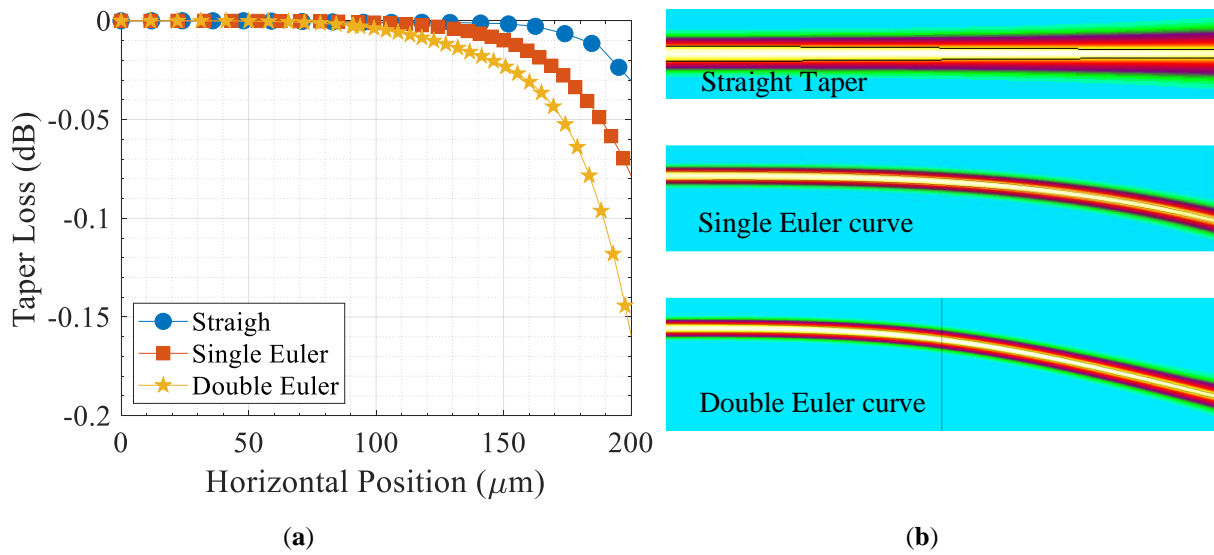
Fig. 3.5. (a) Simulated loss of an SSC based on SI-BH waveguides, without considering material absorptions, (b) simulated modal propagations inside the SCC.
