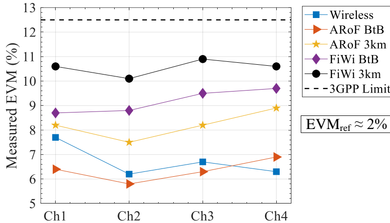
Fig. 4.20. Measured error vector magnitudes (EVMs) of the four 16-QAM subcarriers at different stages of transmission. EVM_{ref} : measured EVM of the signal generated by the AWG (used as a reference).
