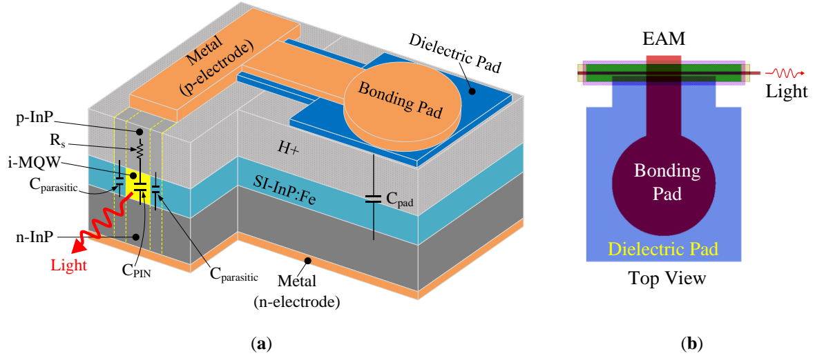
Fig. 2.30. (a) Schematic of an EAM showing different capacitive effects, (b) top view of the layout of an EAM.
