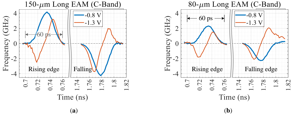
Fig. 3.50. Enhanced view of the large-signal frequency chirp of (a) the 150-μm long EAM and (b) the 80-μm long EAM, both in an REAM-SOA PIC configuration. \lambda = 1545 nm, T = 25^\circ\text{C} .
