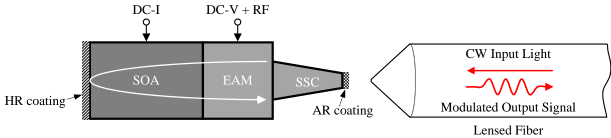
Fig. 2.33. Schematic diagrams of an RSOA-EAM and a lensed fiber used for input/output coupling.
