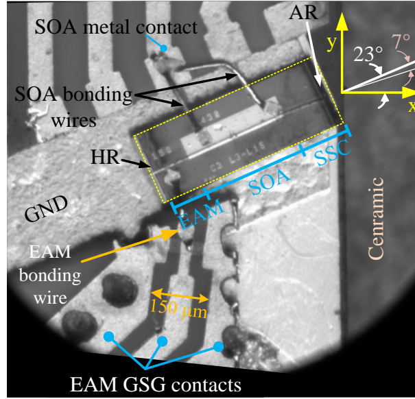
Fig. 3.33. Picture of an REAM-SOA mounted on a 23°-tilted HF carrier.
