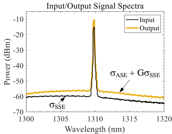
Fig. 3.24. Spectra of input and output signals which are used in estimating amplifier noise figure.
