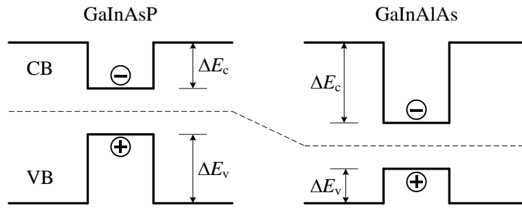
Fig. 2.6. Schematic illustration of electronic band profiles of GaInAsP (left) and GaInAlAs (right) MQWs.
