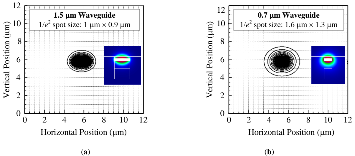
Fig. 3.8. Simulated intensity profiles of (a) 1.5 \mu\text{m} and (b) 0.7 \mu\text{m} waveguides expressed in terms of horizontal and vertical waveguide dimensions. Insets: color plots of the mode profiles.
