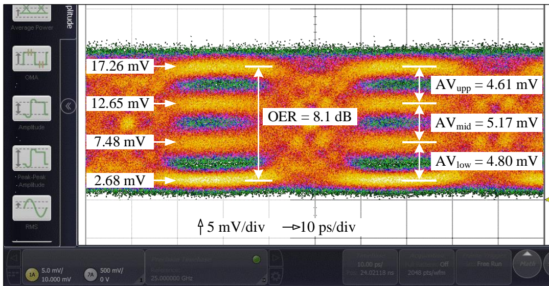
Fig. 4.14. 25 Gbaud PAM-4 eye diagrams obtained from a 100- \mu\text{m} long EAM in an REAM-SOA configuration operating. \lambda = 1310\text{ nm} , V_{\text{bias}} = -1.1\text{ V} , V_{PP} = 1.9\text{ V} , T = 25^\circ\text{C} .
