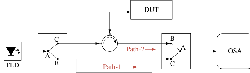
Fig. 3.23. A simplified schematic of the experimental setup used for RSOA gain and NF measurement (cf. Fig. 3.14).
