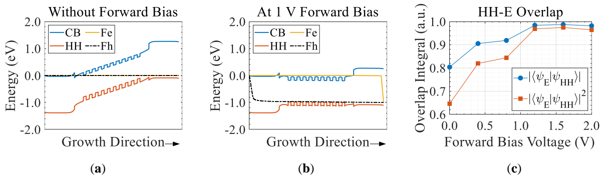
Fig. 2.25. Simulated electronic band structure of a compressive strained GaInAsP MQW (a) without and (b) with applied forward bias, (c) heavy-hole to conduction band overlap integral as a function of forward bias voltage.
