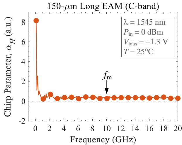
Fig. 3.44. Small-signal chirp parameter as a function of modulation frequency obtained from a 150- \mu\text{m} long EAM in an REAM-SOA configuration.
