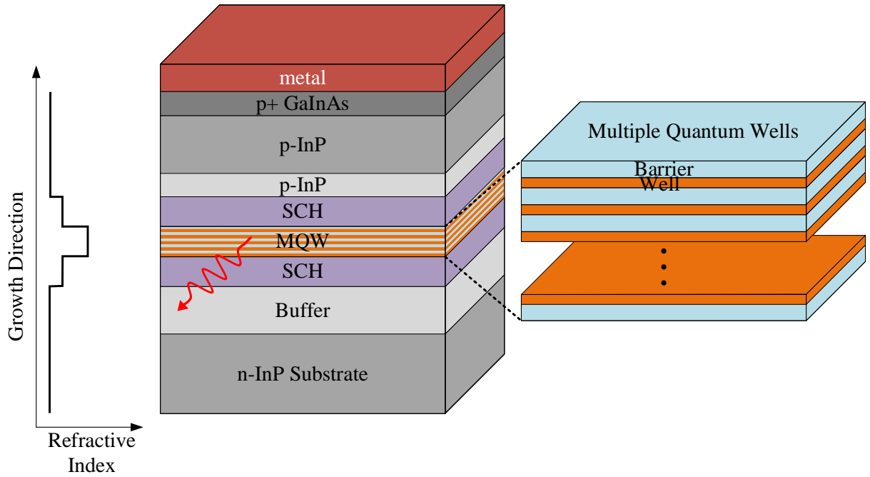
Fig. 2.4. Schematic diagram of multiple quantum well structure based on separate carrier confining heterostructures. Inset: schematic of refractive indices of the epitaxial layers (left) and enhanced view the MQW stack (right).
