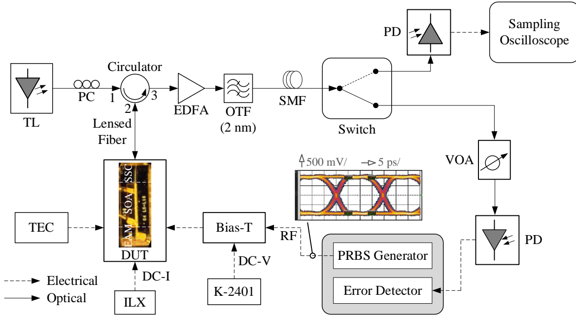
Fig. 4.1. Schematic diagram of a standard experimental setup for 25 Gb/s NRZ transmission.
