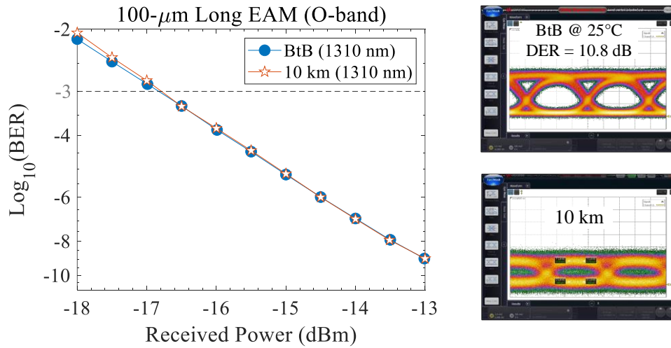
Fig. 4.8. BER performance of a 100- \mu\text{m} long EAM in an REAM-SOA configuration at 25 Gb/s NRZ, for an input wavelength of 1310 nm. T = 25^\circ\text{C} , EAM bias: -1.3 V/2.6 V PP , I_{\text{SOA}} = 40 mA.
