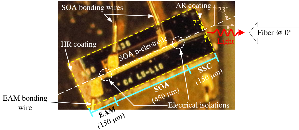
Fig. 2.34. Picture of an REAM-SOA chip-on-carrier mounted on a 23°-tilted high frequency carrier.
