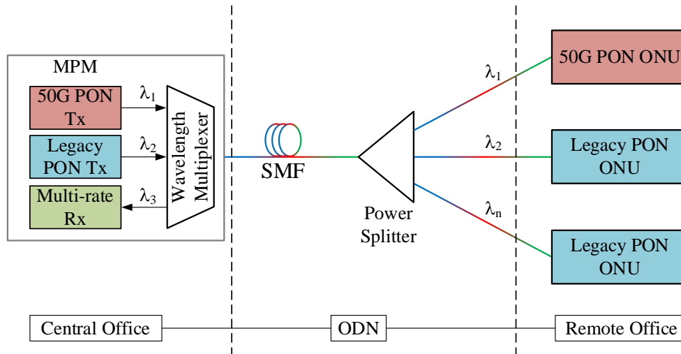
Fig. 1.2. Schematic diagram of a 50G PON system in coexistence with legacy PONs (after [13]). MPM: multi-PON module, Tx: Transmitter, Rx: Receiver.
