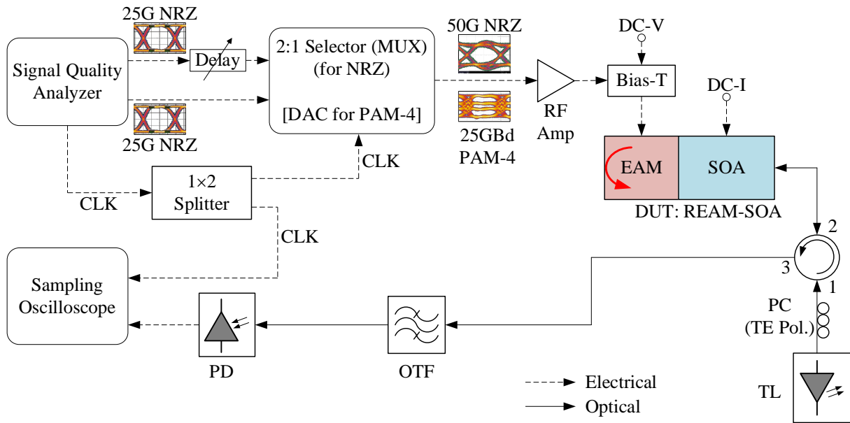
Fig. 4.10. Schematic diagram of experimental setup for generating and transmitting 50 Gb/s NRZ and PAM-4 signals.
