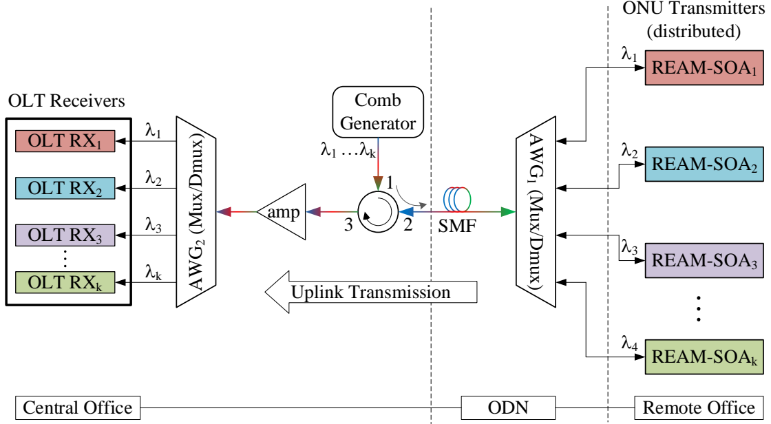
Fig. 1.7. Schematic diagram of a WDM-PON system based on REAM-SOAs as ONU transmitters.
