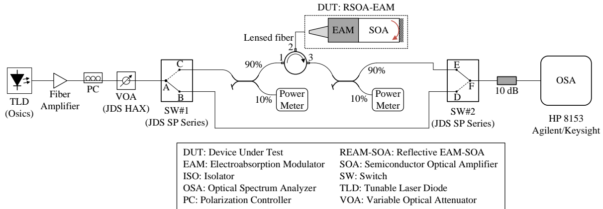
Fig. 3.14. Experimental setup for SOA gain and noise figure measurement in a reflective device configuration.
