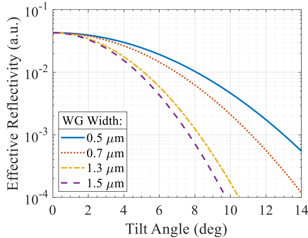
Fig. 3.2. Calculated facet reflectivity versus tilt angle for different waveguide widths at 1550 nm ( n_1 = 3.46 , n_2 = 3.32 ).
