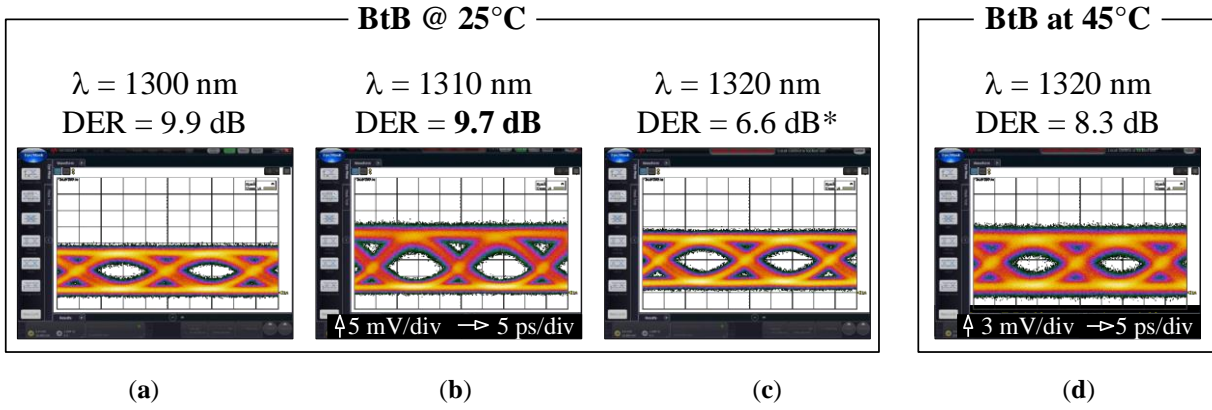
Fig. 4.12. Back-to-back 50G NRZ eye diagrams obtained from a 100- \mu m long EAM in an REAM-SOA configuration at 25°C for input wavelengths of (a) 1300 nm at -0.6 V, (b) 1310 nm at -1.3 V, (c) 1320 nm at -1.4 V, (d) 1320 nm at 45°C and -1 V. I_{SOA} = 40 mA. [* Lower DER at 1320 nm because of limited voltage swing, \sim 2.8 V PP required.]
