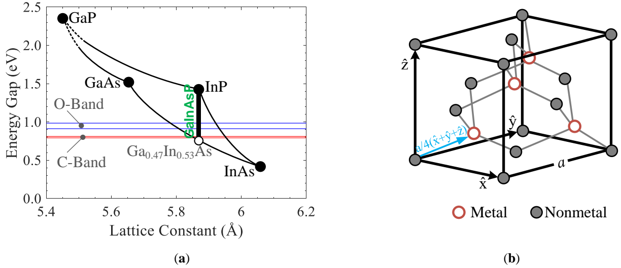
Fig. 2.1. (a) Bandgaps of constituent binaries of GaInAsP as a function of lattice constant (after [39]), (b) zincblende crystal structure (after [40]).
