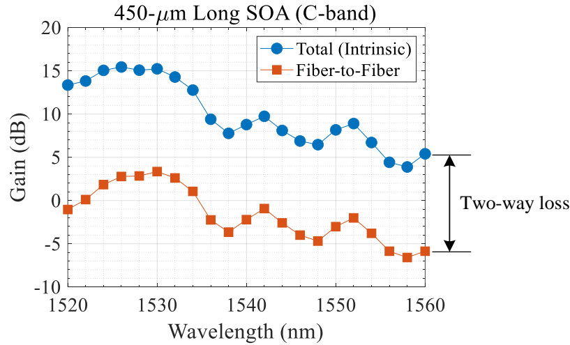
Fig. 3.19. Intrinsic and fiber-to-fiber gain spectra of the 450- \mu\text{m} long SOA in a reflective configuration at a pump current of 120 mA. P_{\text{in}} = -28.5 \text{ dBm} , T = 25^\circ\text{C} .
