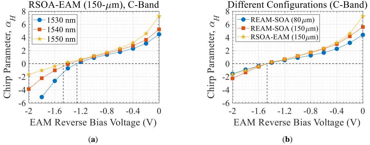
Fig. 3.46. Small-signal chirp parameters of (a) 150 \mu\text{m} long EAM in an RSOA-EAM configuration ( I_{\text{SOA}} = 90 mA), (b) comparison of chirp performances of the 80- \mu\text{m} long EAM in REAM-SOA and the 150- \mu\text{m} long EAM in both REAM-SOA and RSOA-EAM configurations ( \lambda = 1550 nm). T = 25^\circ\text{C} . I_{\text{SOA}} = 90\text{--}120 mA.
