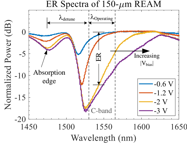
Fig. 3.27. Spectrum of static extinction ratio of a 150- \mu\text{m} long REAM as a function of reverse bias voltage. T = 25^\circ\text{C} .
