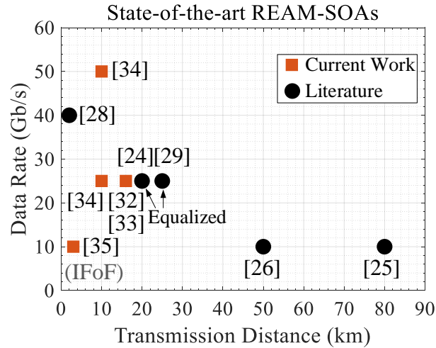
Fig. 1.8. State-of-the-art of REAM-SOAs based on NRZ modulation format ([35] is based on 16-QAM ARoF).
