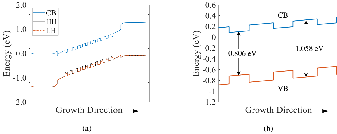
Fig. 2.12. (a) Simulated native bandgap profile of compressive strained GaInAsP QWs surrounded by unstrained GaInAsP barriers, grown on InP substrate, (b) enhanced view of the band structure showing transition energies.
