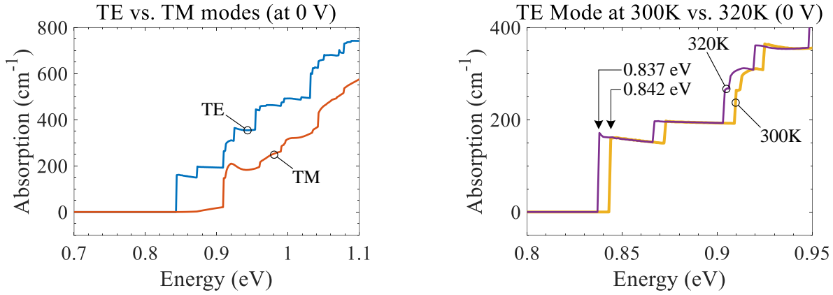
Fig. 2.21. Simulated modal absorption spectra of compressive strained GaInAsP MQW without a DC field (0 V bias): (a) for TE versus TM modes, (b) TE mode at 300K (26.85°C) vs. 320K (46.85°C).
