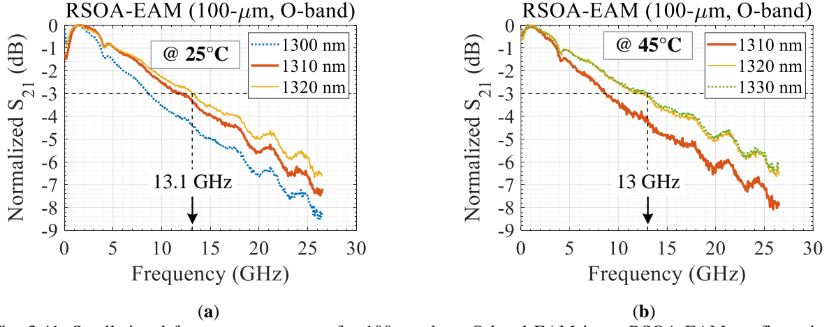
Fig. 3.41. Small-signal frequency response of a 100- \mu\text{m} long O-band EAM in an RSOA-EAM configuration for different input wavelengths, operating at (a) 25°C and (b) 45°C. P_{\text{in}} = 0 dBm, I_{\text{SOA}} = 40 mA. The EAM's reverse bias voltages are -0.6 V, -0.8 V, and -1.2 V in order of increasing wavelength for both (a) and (b).
