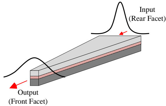
Fig. 3.1. Schematic diagram of a taper and shapes of the optical modes at its input and output (after [18]).
