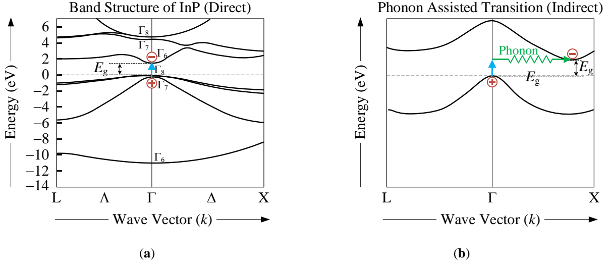
Fig. 2.2. (a) Band structure of InP in the Brillouin zone centered at the \Gamma point ( k = 0 ) (after [41]), (b) illustration of phonon assisted electronic transition in indirect bandgap materials.
