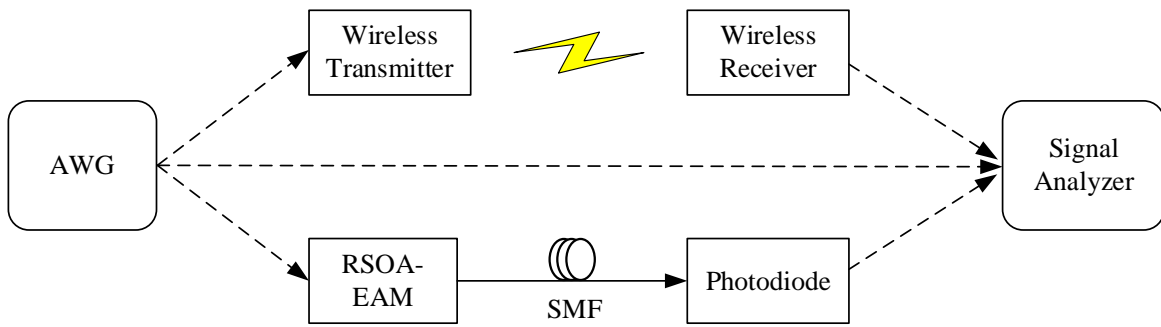
Fig. 4.18. Schematic of the experimental setup for analyzing EVM contributions of the wireless and optical links.
