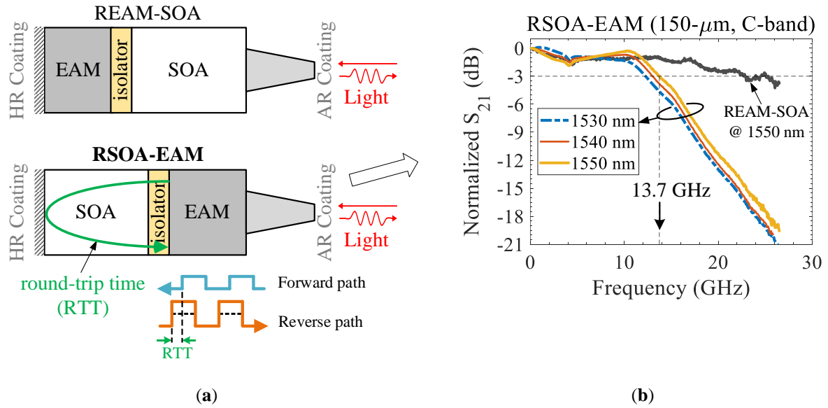
Fig. 3.38. (a) Schematics of REAM-SOA (top) and RSOA-EAM (bottom) PIC configurations, (b) small-signal frequency response ( S_{21} parameter) of the 150- \mu\text{m} long EAM in an RSOA-EAM configuration ( L_{EAM} = 150 \mu\text{m} , L_{ISO} = 10 \mu\text{m} ). P_{in} = 0 dBm, I_{SOA} = 90 mA, T = 25^\circ\text{C} . Isolator: inter-electrode isolation.
