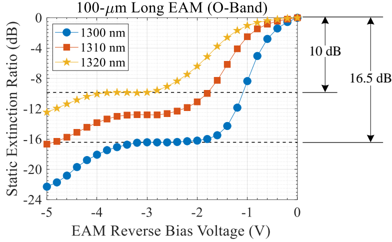
Fig. 3.30. Static extinction ratios of a 100- \mu\text{m} long O-band REAM at different operating wavelengths. T = 25^\circ\text{C} .
