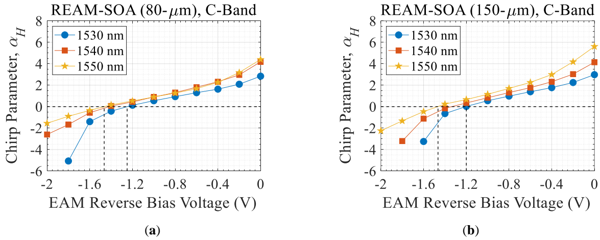
Fig. 3.45. Small-signal chirp parameters of (a) 80 \mu\text{m} (b) 150 \mu\text{m} long EAMs, both devices being in an REAM-SOA PIC configuration. T = 25^\circ\text{C} . I_{\text{SOA}} = 120 \text{ mA} for (a) and 90 mA for (b).
