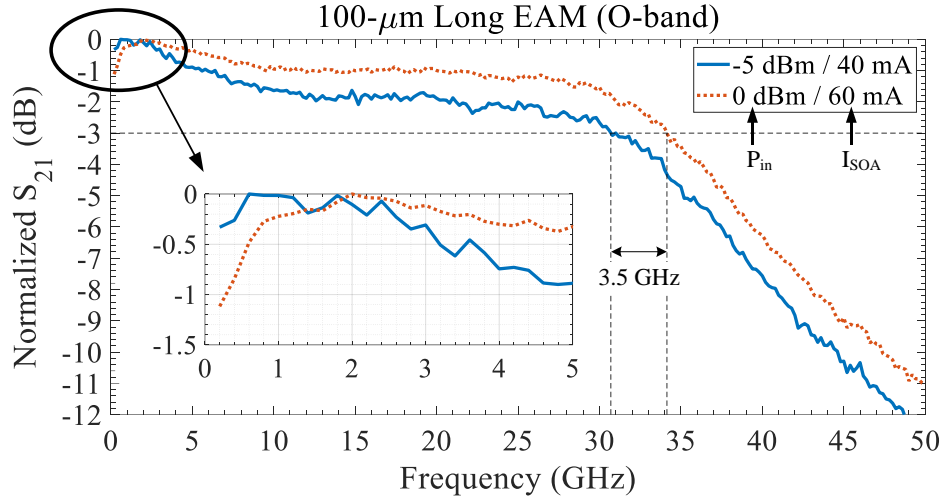
Fig. 3.40. S_{21} parameter of a 100- \mu\text{m} long O-band EAM in an REAM-SOA configuration for different input power levels (−5 dBm and 0 dBm) and SOA pump currents (40 mA and 60 mA) at 1310 nm. V_{\text{bias}} = -1 V, T = 25^\circ\text{C} .
