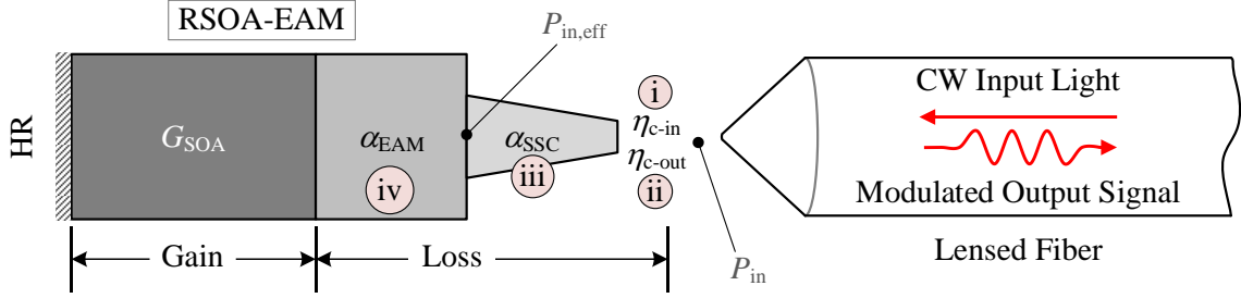
Fig. 3.11. Schematic diagram of an RSOA-EAM with integrated SSC, and the various insertion loss contributions. The labels represent losses: (i) input coupling loss, (ii) output coupling loss, (iii) SSC loss (absorption and bending), (iv) EAM absorption loss at 0 V. Coupling losses in dB are obtained as: C_{in/out} [\text{dB}] = 10\log_{10}(\eta_{c-in/out}) .
