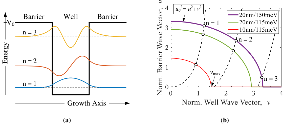
Fig. 2.8. Illustration of (a) wave functions of the first three confined states of an electron in the conduction band, (b) matching conditions for confined states of a GaInAsP QW of different well thicknesses (10 and 20 nm) and barrier potentials (115 and 150 meV). m^* = 0.045m_0 used for GaInAsP [39].
