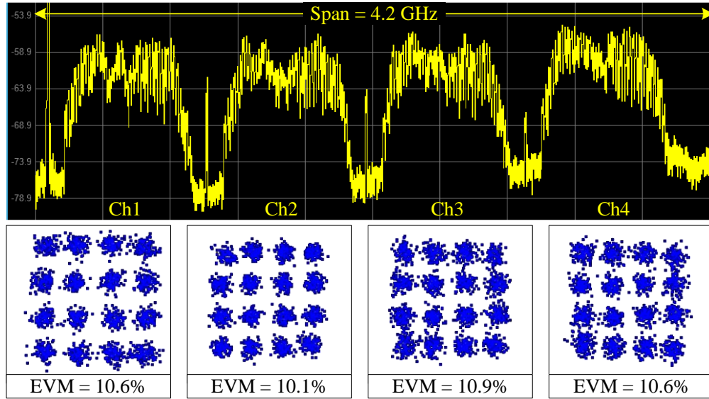
Fig. 4.17. Received spectrum (top) of a four-channel 16-QAM signal after V-band/IFoF uplink transmission using an RSOA-EAM, and the corresponding constellation diagrams (bottom). \uparrow 5 dB/div, \rightarrow 420 MHz/div.
