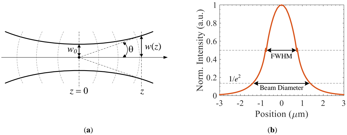
Fig. 3.7. (a) Schematic representation of an optical beam propagation, (b) its intensity field profile.
