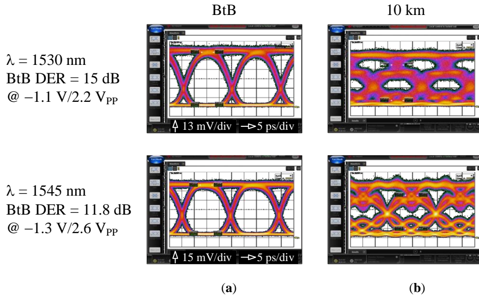
Fig. 4.2. Eye diagrams of a 150- \mu m long EAM in an REAM-SOA PIC configuration operating at 25 Gb/s NRZ in (a) back-to-back, (b) 10 km configurations. T = 25^\circ\text{C} , I_{\text{SOA}} = 90 mA.
