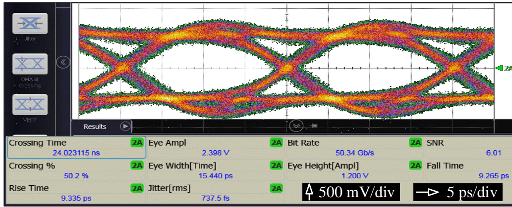
Fig. 4.11. Eye diagram of 50 Gb/s NRZ electrical signal generated using the experimental setup shown above.
