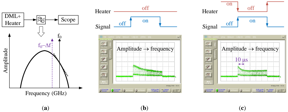
Fig. 1.5. (a) Schematic diagram of experimental setup for measuring emission wavelength of a laser operating in burst-mode, (b) measured wavelength (frequency) without counter-heating, and (c) with counter-heating.
