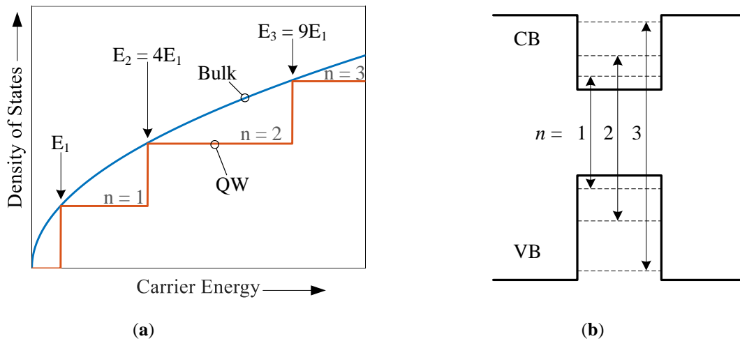
Fig. 2.9. (a) Dependence of density of states on carrier energy in bulk (smooth curve) and quantum wells (step-like curve), (b) schematic illustration of quantized energy levels in the valence and conduction bands of a GaInAsP QW.
