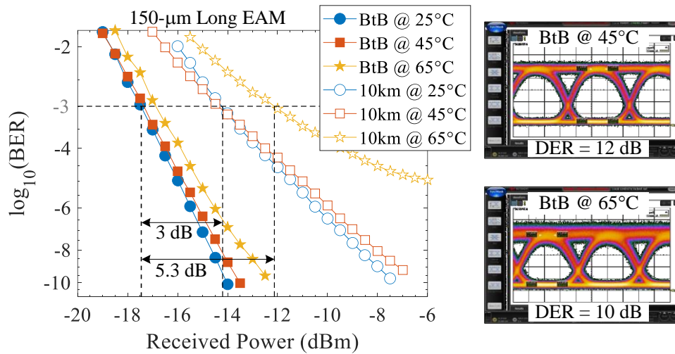
Fig. 4.4. BER performances of a 150- \mu\text{m} EAM in an REAM-SOA between 25°C and 65°C submount temperatures, at 25 Gb/s NRZ. \lambda = 1545\text{ nm} , I_{\text{SOA}} = 90\text{ mA} . EAM bias conditions: -1.3\text{ V}/2.6\text{ V}_{\text{PP}} at 25°C, -1.1\text{ V}/2.2\text{ V}_{\text{PP}} at 45°C, -0.8\text{ V}/1.6\text{ V}_{\text{PP}} at 65°C. [Inset: unfiltered 25 Gb/s NRZ BtB eye diagrams at 45°C (top) and 65°C (bottom).]
