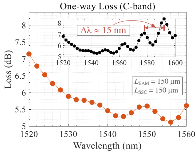
Fig. 3.13. Measured one-way loss spectrum of a C-band PIC based on a 150- \mu\text{m} long EAM and a 150- \mu\text{m} long SSC. Inset: extended view of the loss spectrum showing ripples up to 1600 nm.
