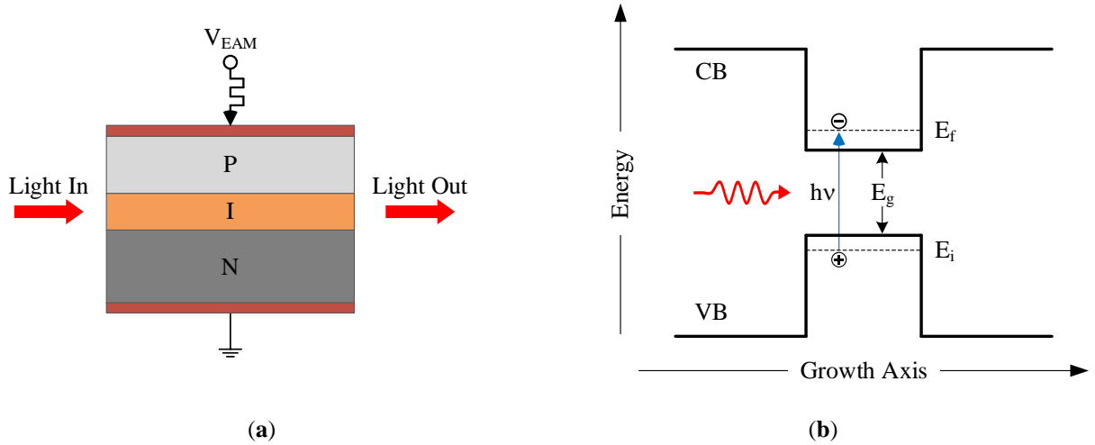
Fig. 2.13. Schematic diagram of (a) an EAM and (b) photon-assisted electronic transition through the bandgap.
