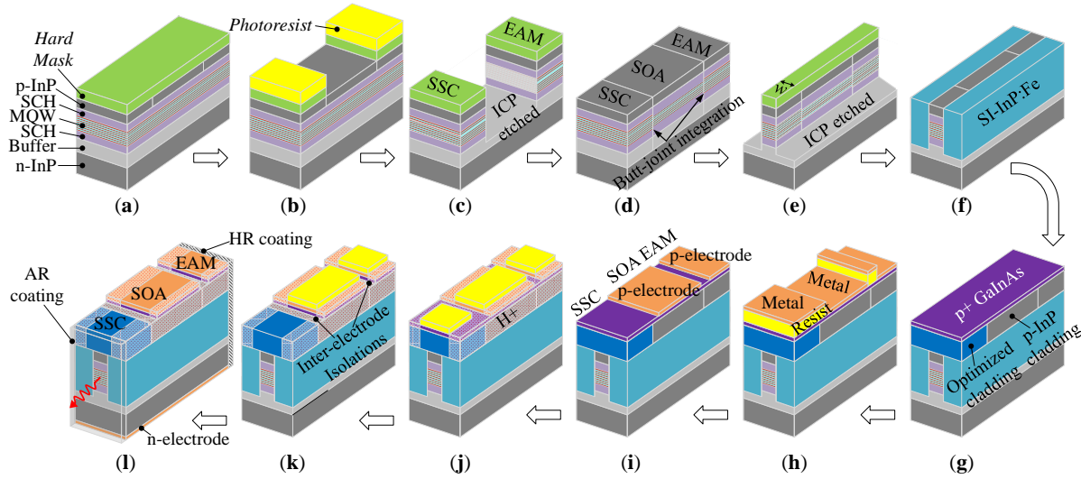
Fig. 2.26. Schematic illustration of epitaxial growth process flow based on butt-joint integration technique and SI-BH waveguide definition: (a) hard mask deposition on the EAM's MQW structure grown in the first epitaxy step, (b) hard mask etching using photoresist, (c) ICP etching of the region outside the EAM and the SSC, (d) SOA's MQW regrowth, (e) ICP etching to define a ridge width of w ( w = 1.3\text{--}1.5\ \mu\text{m} ), (f) SI-BH regrowth (laterally growing Fe-doped InP layer), (g) growing p-InP cladding and ternary p-contact layers, (h) metal deposition using photoresist, (i) defining p-electrodes for EAM and SOA sections using lift-off, (j) \text{H}^+ ion implantation laterally as well as in the region between BBs, (k) ternary opening to form inter-electrode isolations, (l) final PIC after removing the photoresist and AR/HR treatments.
