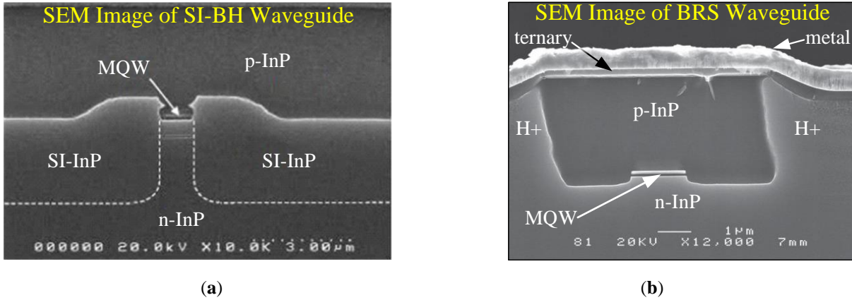
Fig. 2.28. Scanning electron microscope images of (a) SI-BH and (b) BRS waveguides (after [15]).
