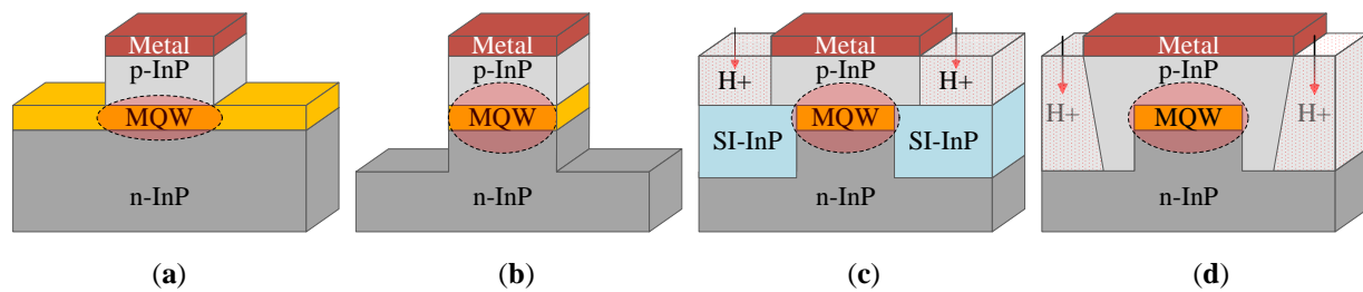
Fig. 2.27. Schematic diagrams of different waveguide technologies: (a) shallow ridge (b) deep ridge, (c) SI-BH, and (d) buried ridge stripe waveguides (adapted from [52]).
