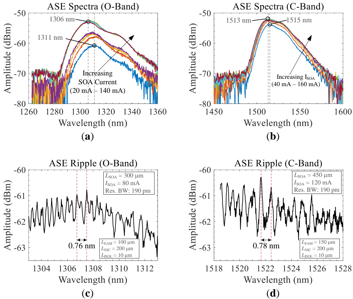
Fig. 3.16. ASE spectra of reflective SOAs at different pump currents: (a) 300- \mu\text{m} long O-band SOA, (b) 450- \mu\text{m} long C-band SOA, and ASE ripples of (c) the O-band SOA at 80 mA, (d) the C-band SOA at 120 mA. Res. BW: 190 pm.
