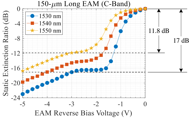
Fig. 3.29. Static extinction ratios of a 150- \mu\text{m} long C-band EAM in a reflective configuration at different operating wavelengths (1530–1550 nm). T = 25^\circ\text{C} .
