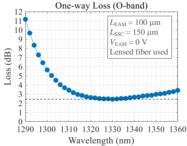
Fig. 3.12. Measured one-way loss spectrum of an O-band PIC based on a 100- \mu\text{m} EAM and a 150- \mu\text{m} SSC.
