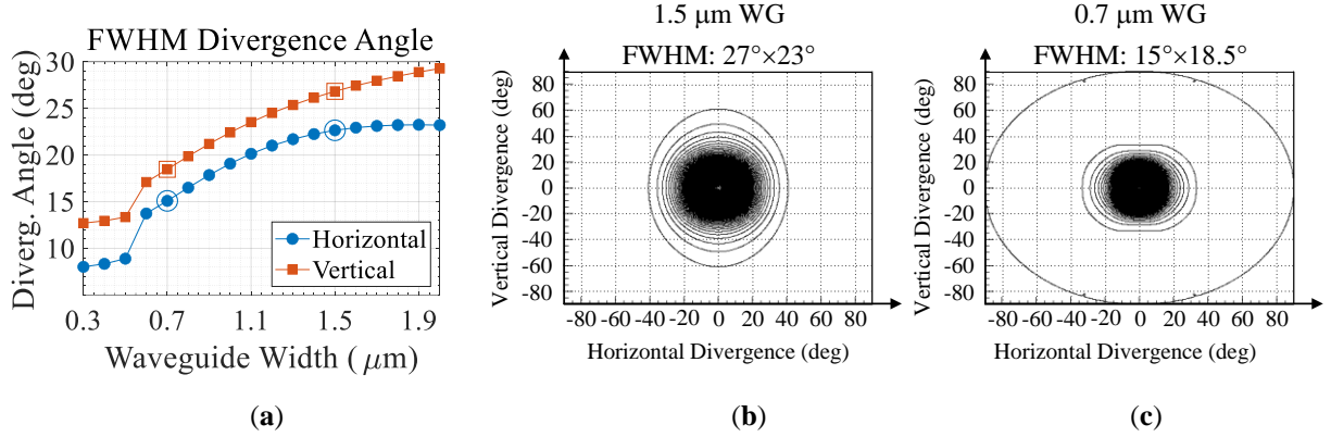
Fig. 3.6. Simulated FWHM divergence angles as a function of waveguide width, and contour plots of far-field intensity distributions of the optical modes of (b) a 1.5- \mu\text{m} , and (c) a 0.7- \mu\text{m} waveguides.
