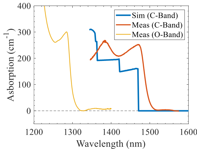
Fig. 2.22. Comparison of simulated and measured absorption spectra of a 150-μm long C-band EAM at 0 V.
