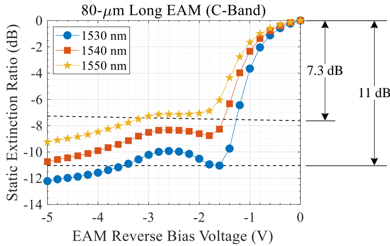
Fig. 3.28. Static extinction ratios of an 80- \mu\text{m} long C-band EAM in a reflective configuration at different operating wavelengths (1530–1550 nm). T = 25^\circ\text{C} .
