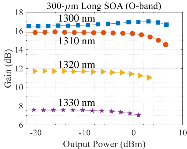
Fig. 3.21. Gain as a function of output signal power at different operating wavelengths. I_{SOA} = 60 mA, T = 25^\circ\text{C} .
