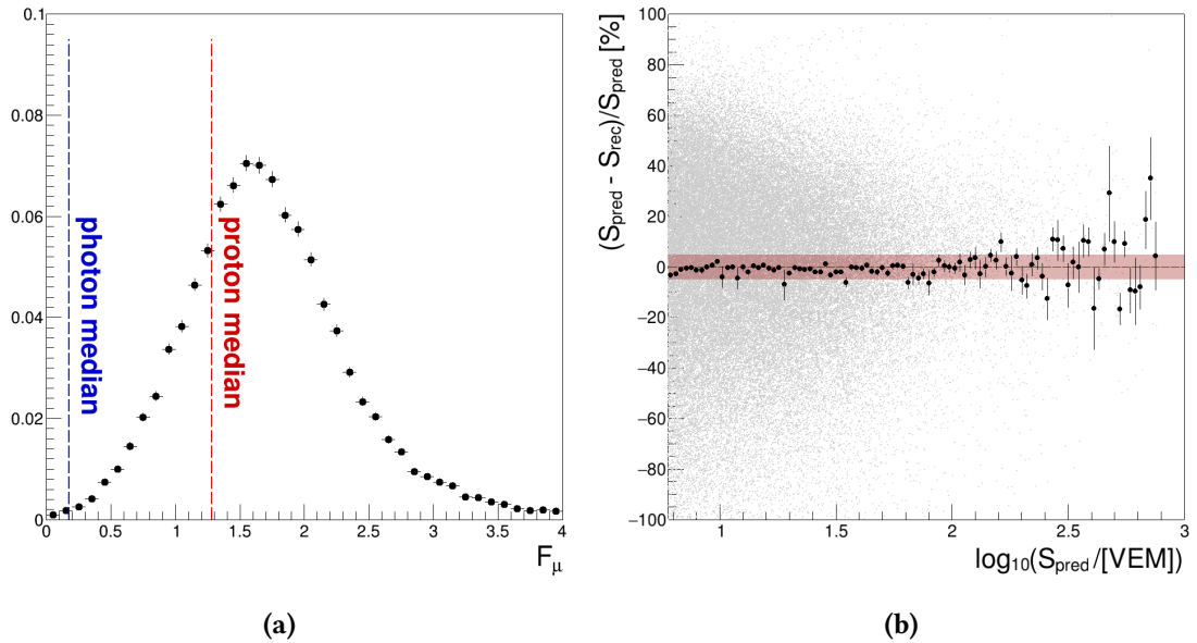
Figure 5.14: (5.14a): Distribution of F_\mu estimated from hybrid data. The vertical dashed lines are the medians of the proton (red) and the photon (blue) distributions. (5.14b): Relative difference between the predicted and the measured signals as a function of the predicted signal. The red band corresponds to 5% difference.
