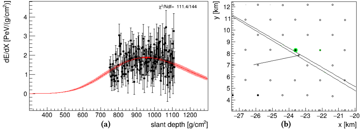
Figure C.19: Longitudinal profile (C.19a) of the candidate 37073026. The red line indicates the reconstructed profile, while the red shaded area represents the uncertainty. The red point shows the reconstructed X_{\max} . (C.19b). Event footprint on the SD array. Each colored circle indicate a triggered station. The colors (from blue to green) represent the trigger times while the dimensions are proportional to the signal size.
