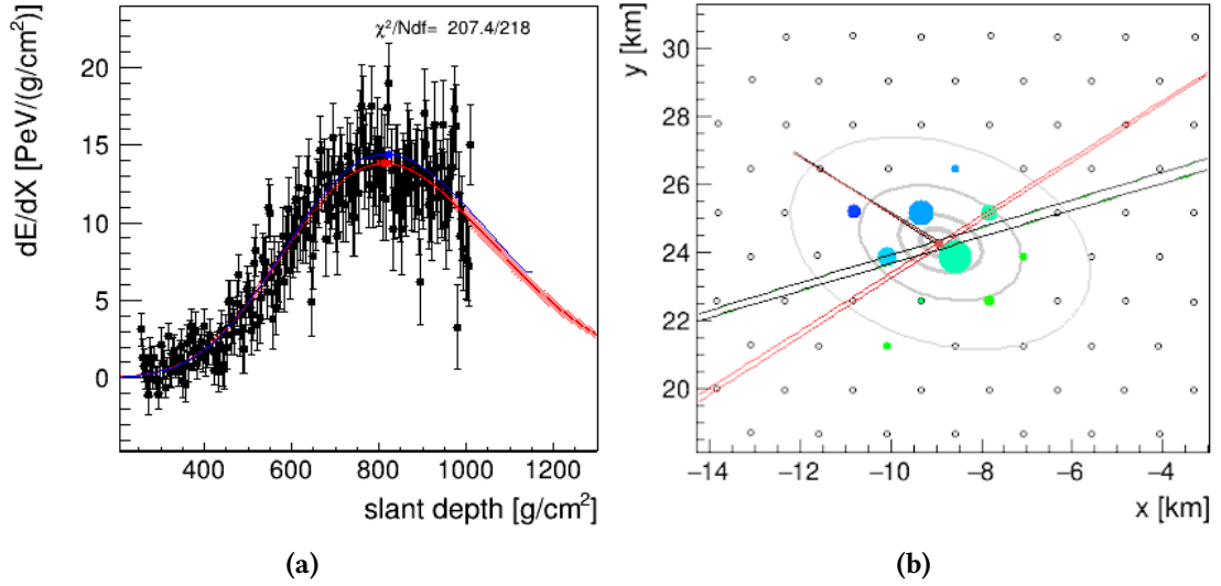
Figure 5.6: Example of a hybrid simulated event generated by a primary proton with E_{MC} = 9.55 \times 10^{18} eV and zenith angle \theta = 40.3^\circ . (a) Longitudinal profile reconstruction. The blue line represents the Monte Carlo profile, while the reconstructed one is shown by the red line. The red shaded area represents the uncertainties in the profile reconstruction. The blue and red points represent the Monte Carlo and reconstructed X_{\text{max}} , respectively. (b) Event footprint on the SD. Each circle represents one of the 10 triggered stations. The colors (from blue to green) represent the trigger times while the dimension is proportional to the signal size.
