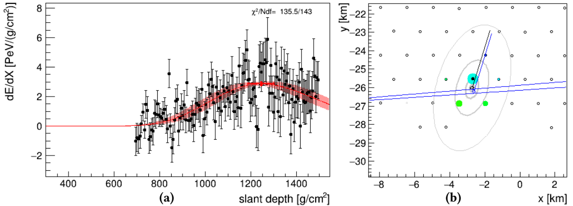
Figure C.3: Longitudinal profile (C.3a) of the candidate 3478968. The red line indicates the reconstructed profile, while the red shaded area represents the uncertainty. The red point shows the reconstructed X_{max} . (C.3b). Event footprint on the SD array. Each colored circle indicate a triggered station. The colors (from blue to green) represent the trigger times while the dimensions are proportional to the signal size.
