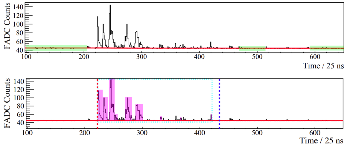
Figure 2.4: Top: illustration of the baseline estimation (red), constructed from the individual segments (highlighted in green) and interpolation, on a high-gain FADC trace of a PMT. Bottom: identification of signal fragments (magenta filled boxes) and the final merged signal window (large dotted cyan box). Based on the number of peaks, this trace probably contains \sim 5 muons with some additional electromagnetic component. Trace start and stop times are denoted with the vertical dashed red and blue lines, respectively. From [62].
