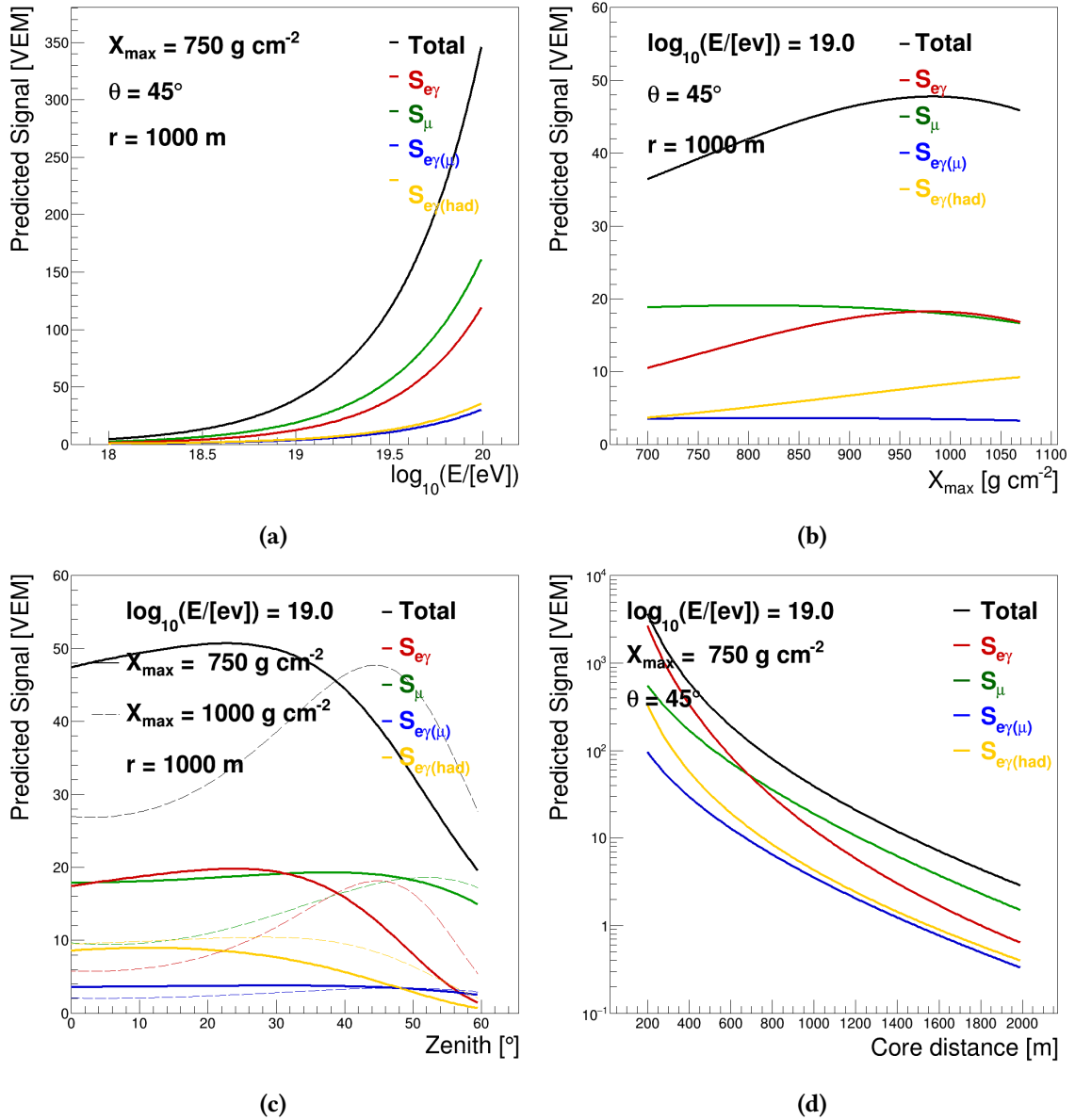
Figure 5.7: Evolution of signal components as a function of energy (5.7a), X_{max} (5.7b), zenith (5.7c) and core distance (5.7d). The predicted total signal (black line) is shown together with each parametrized signal component: e^\pm\gamma (red), \mu (green), e^\pm\gamma(\mu) (blue) and e^\pm\gamma(had) (yellow).
