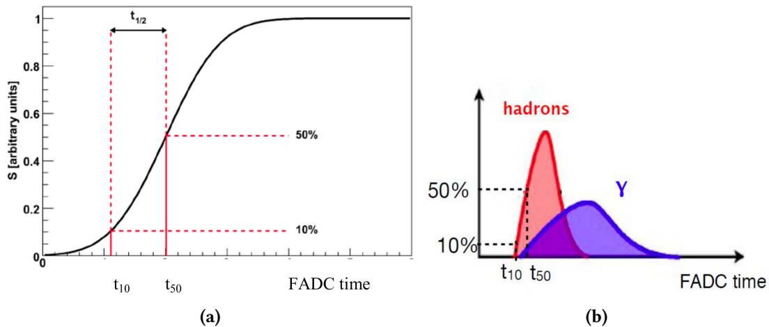
Figure 5.2: Definition of t_{1/2} as the difference between the 10% and 50% time quantiles of the signal trace (5.2a). The differences between a signal induced by a hadron-initiated cascade (red) and a photon-initiated cascade are highlighted in (5.2b). From [165].
