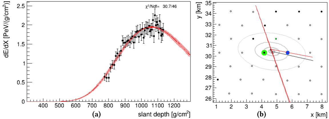
Figure C.17: Longitudinal profile (C.17a) of the candidate 22130573. The red line indicates the reconstructed profile, while the red shaded area represents the uncertainty. The red point shows the reconstructed X_{\max} . (C.17b). Event footprint on the SD array. Each colored circle indicate a triggered station. The colors (from blue to green) represent the trigger times while the dimensions are proportional to the signal size.
