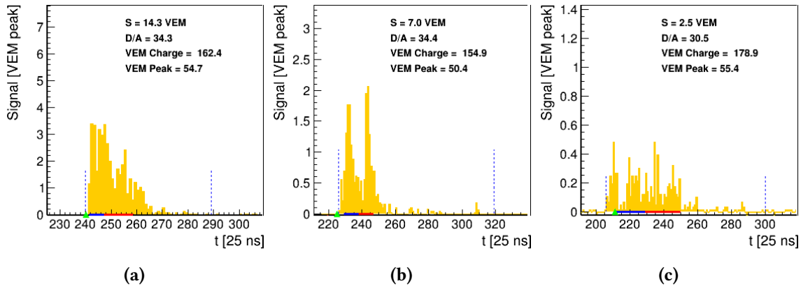
Figure 7.6: Reconstructed signals in the stations used in the most significant candidate for the F_{\mu} calculation. The vertical dashed lines show the start and the stop time of the signals, while the blue and the red horizontal segments show, respectively the risetime and the falltime of the traces.
