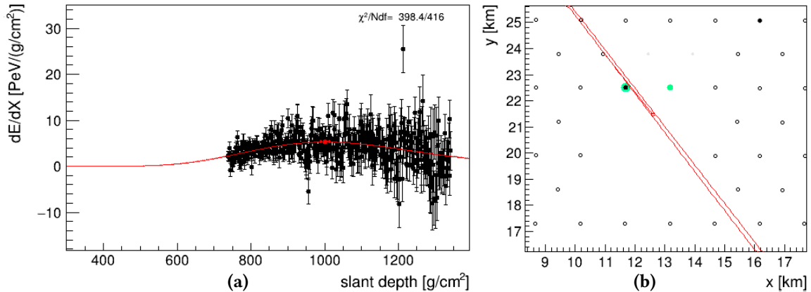
Figure C.18: Longitudinal profile (C.18a) of the candidate 31926471. The red line indicates the reconstructed profile, while the red shaded area represents the uncertainty. The red point shows the reconstructed X_{\max} . (C.18b). Event footprint on the SD array. Each colored circle indicate a triggered station. The colors (from blue to green) represent the trigger times while the dimensions are proportional to the signal size.
