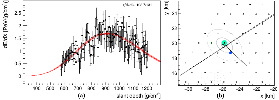
Figure C.5: Longitudinal profile (C.5a) of the candidate 4329935. The red line indicates the reconstructed profile, while the red shaded area represents the uncertainty. The red point shows the reconstructed X_{\max} . (C.5b). Event footprint on the SD array. Each colored circle indicate a triggered station. The colors (from blue to green) represent the trigger times while the dimensions are proportional to the signal size.
