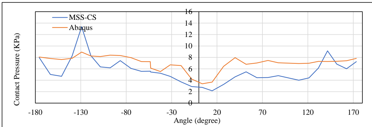
Figure 34. Contact pressure distribution on the horizontal points set
