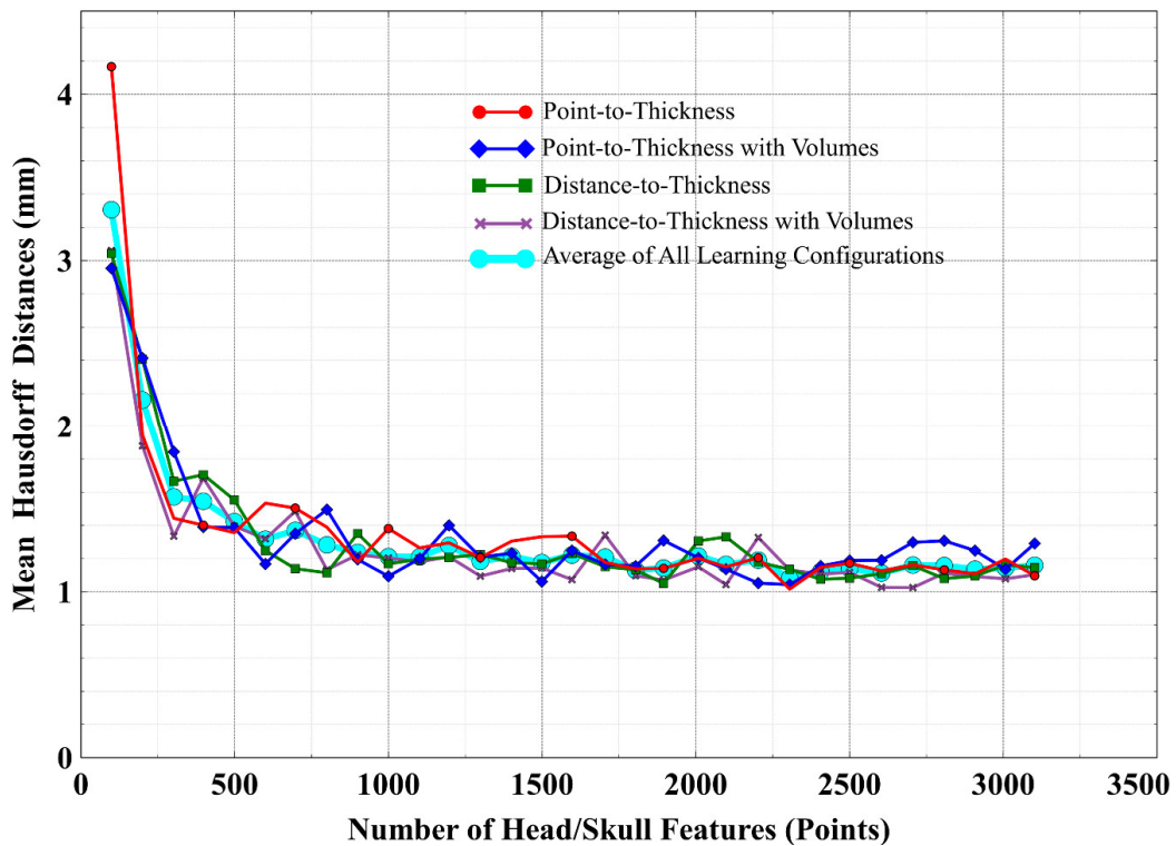
Figure 47. Mean Hausdorff distances computed from the convergence analysis to determine the optimal number of head/skull feature points: the number of head/skull feature points was increased from 100 to 3100 features with the step-size of 100 points. Note that for each learning configurations, the mean Hausdorff distance was computed between the best regressed skull shape and its appropriate CT-based skull shape.
