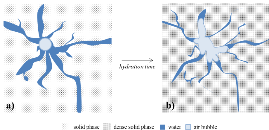
Figure 71. Hypothesis on the evolution of the shape of an air bubble in a water pore surrounded by solid phase.
