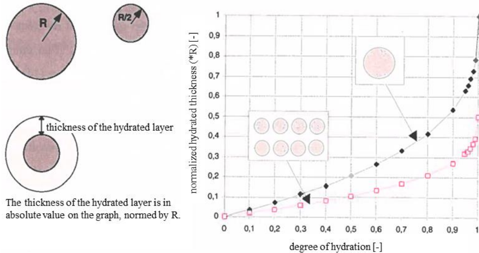
Figure 11. Illustration of the characteristic relation size / hydration: evolution of the normalized thickness of the hydrated layer as a function of degree of hydration for two size particle respectively of R radius and R/2 [19].
