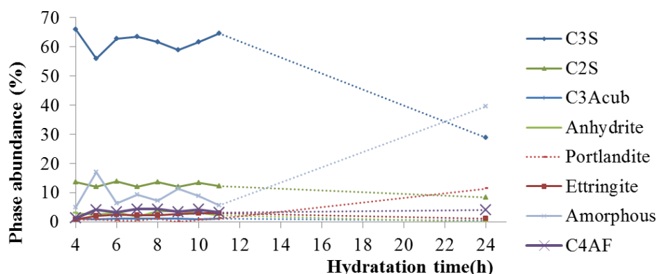
Figure 21. X-Ray diffraction composition as a function of hydration time for paste stopped samples of the reference mix-design.
