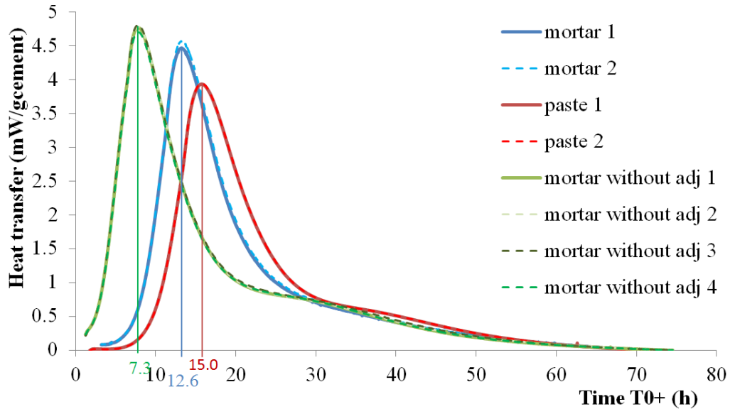
Figure 63. Comparison of calorimetry on paste, mortar and mortar without admixture (adj).
