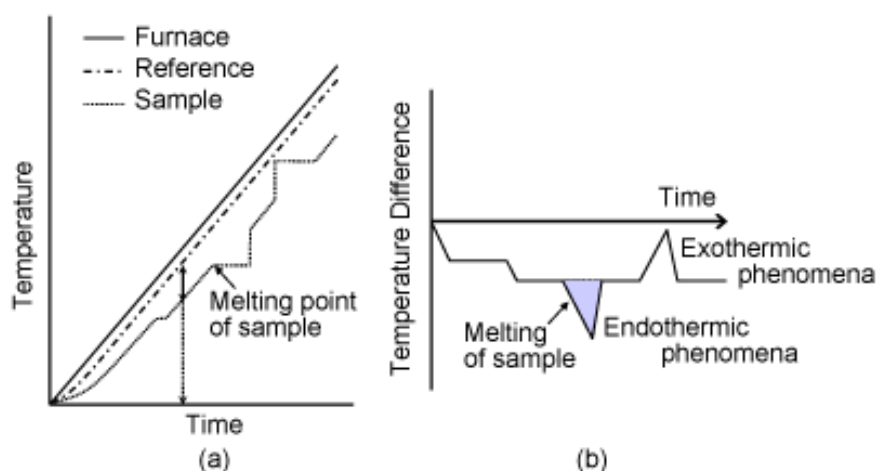
Figure 24. Principle of DTA measurement: evolution of the temperature of the different element on the left which allow to plot the temperature difference on the right.
