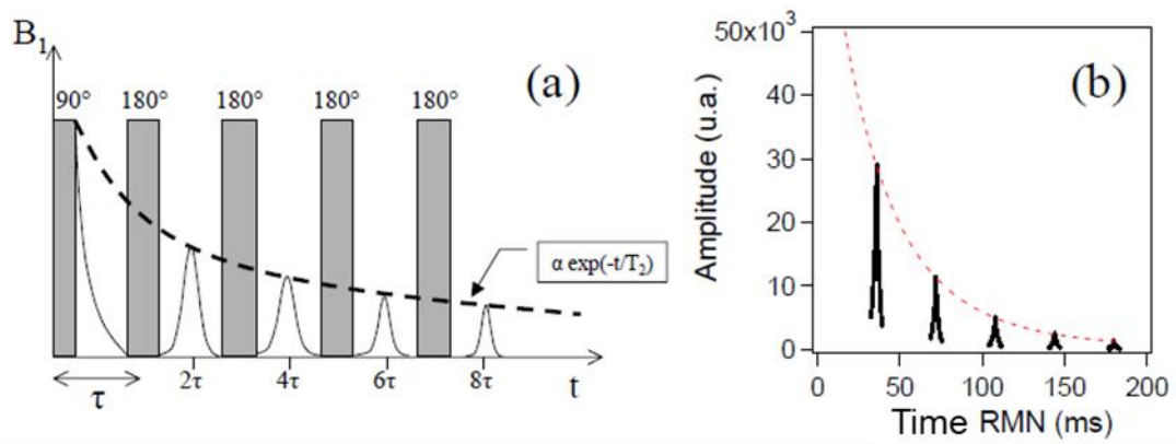
Figure 134. (a) CPMG : decreasing of transversal magnetization M_{xy} . (b) spin echo example [30]
