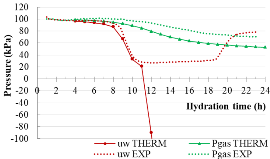
Figure 76. Liquid and gas pressure as a function of time, calculated from calorimetry and MIP experimental data along with calculated phase assemblage and Young Laplace equation.
