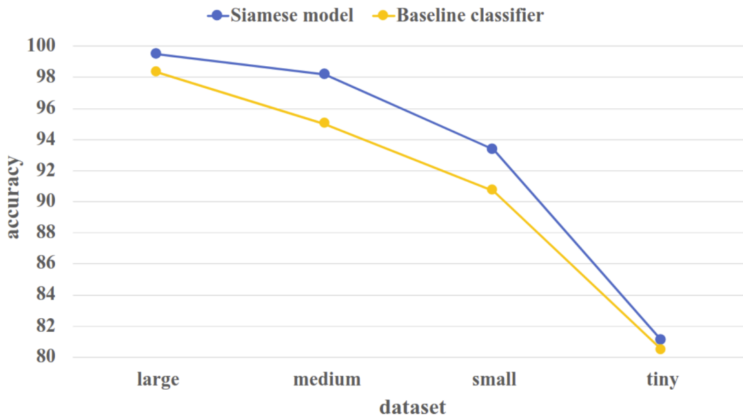
Figure 5.4 – The accuracy (per training dataset) of the Siamese model and the corresponding baseline classifier with shallow architectures.
