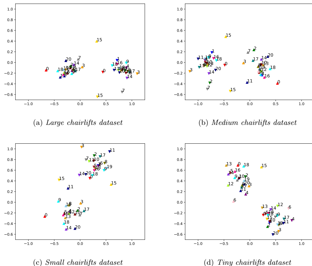
Figure 5.6 – Distribution of all the masks of the 21 chairlifts in the embedding space, after training a Siamese network on the large , medium , small and tiny chairlifts datasets . Up triangles are for open masks while down triangles are for closed masks. The legend numbers are referred to the number of each chairlift.
