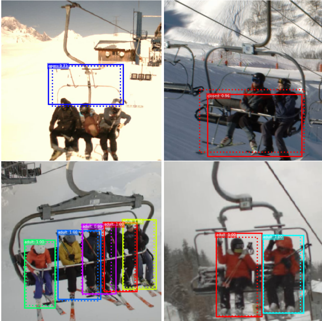
Figure 3.1 – Examples of the desired output. The dotted line represents the ground truth and the solid line represents the detection. Top: safety bar detection, Bottom: people detection.
