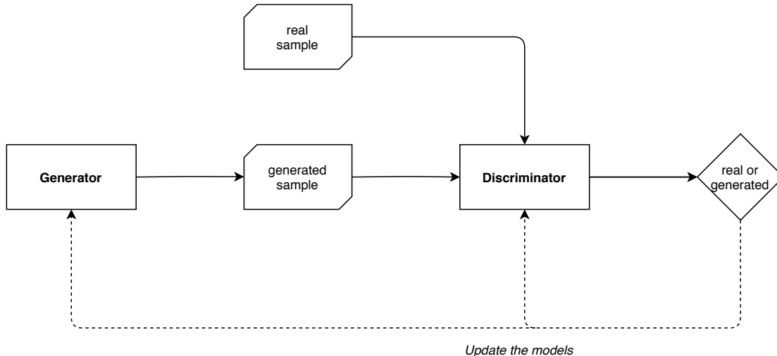
Figure 2.6 – Generative adversarial networks principle.
