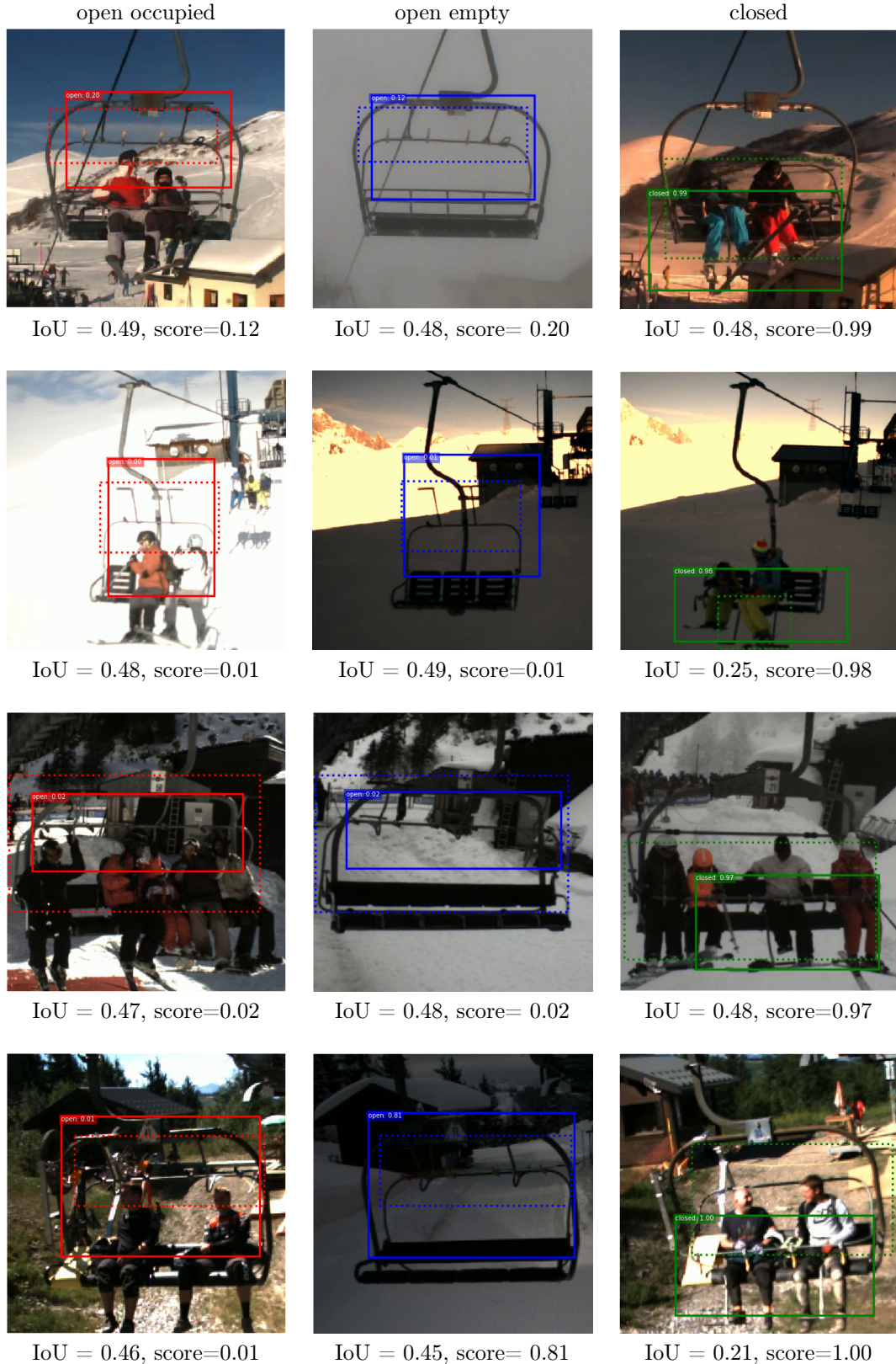
Figure 3.6 – Selected examples of open/closed safety bar object detection results using Faster R-CNN on 2018 chairlifts dataset. The dotted line represents the ground truth and the solid line represents the detection. Under each image we provide IoU between the ground truth bounding box and the predicted one, and the softmax score \in [0,1] . All examples in this figure are false detections. Chairlifts by line are, respectively, C_1 , C_2 , C_{19} and C_{20} .
