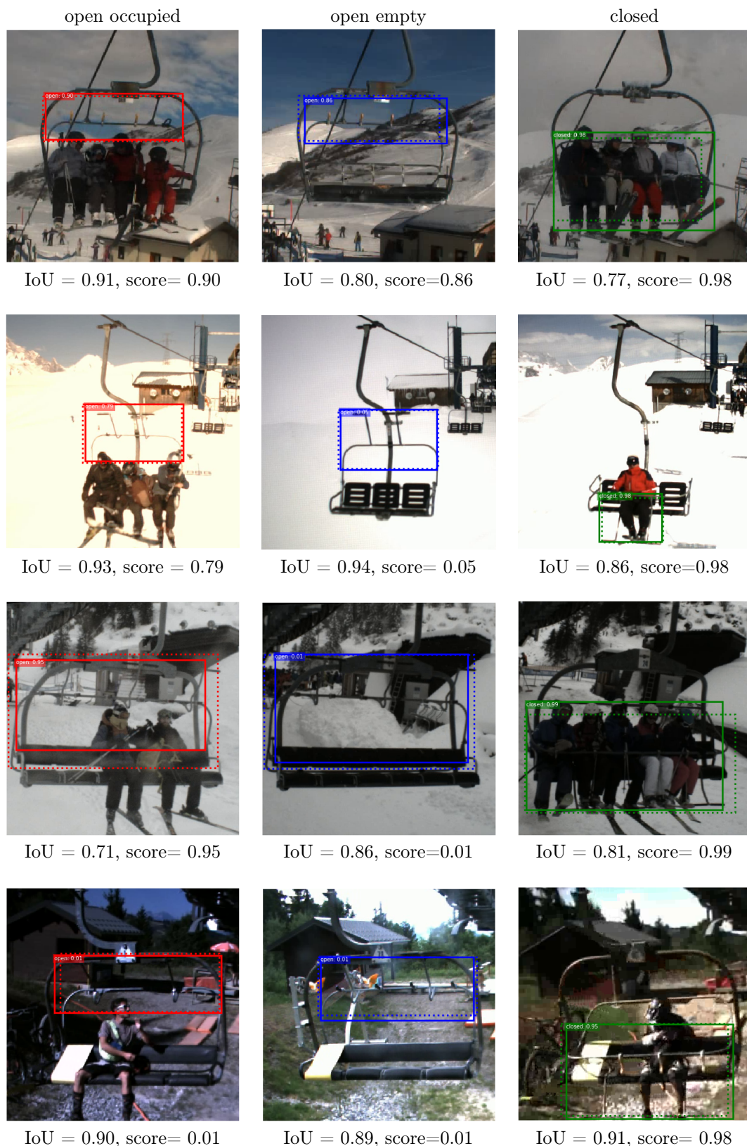
Figure 3.5 – Selected examples of open/closed safety bar object detection results using Faster R-CNN on the 2018 chairlifts dataset. The dotted line represents the ground truth and the solid line represents the detection. Under each image, we provide IoU between the ground truth bounding box and the predicted one, and the softmax score \in [0,1] . All examples in this figure are correct detections. Chairlifts by line are, respectively, C_1, C_2, C_{19} and C_{20} .
