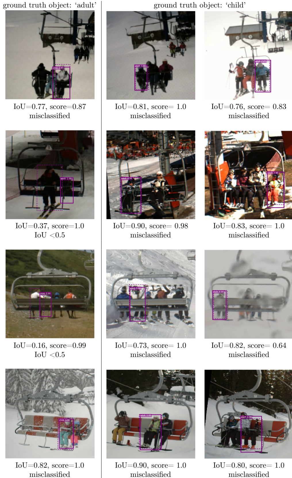
Figure 3.8 – Selected examples of adult/child object detection results using Faster R-CNN on 2019 chairlifts dataset. The dotted line represents the ground truth and the solid line represents the detection. All examples in this figure are false detections. Under each image we provide the softmax score \in [0,1] , and the highest IoU between a ground truth bounding box and the predicted one.
