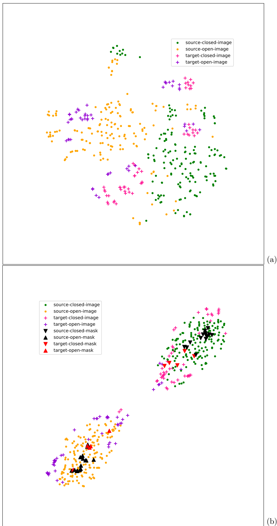
Figure 6.7 – Source and target images and masks visualised using TSNE. (a) Embedding space of the baseline classifier, (b) Embedding space of the Siamese model with the corresponding open and closed masks. See text for explanation.
