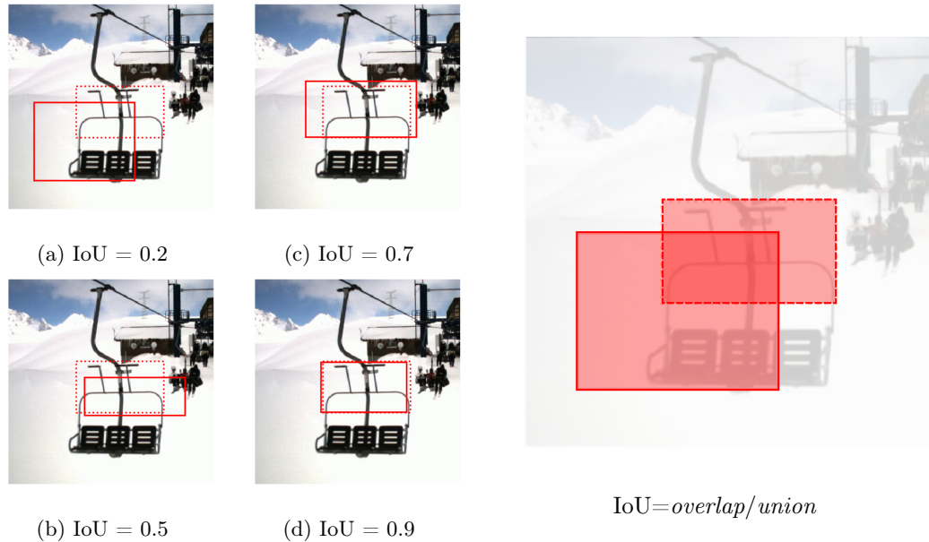
Figure 3.4 – The overlap and union for the ground truth bounding box (dotted) and different predicted bounding boxes (solid) leading to different IoU values.
