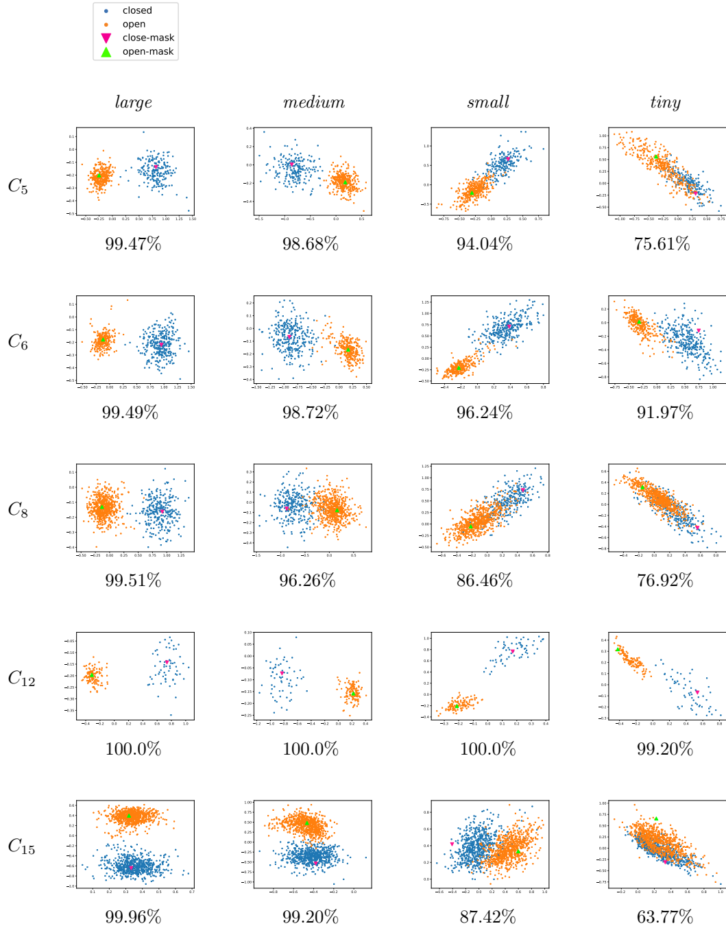
Figure 5.5 – Projections in the 2D embedding space of the masks and test images of 5 different chairlifts C_5, C_6, C_8, C_{12} and C_{15} , after training a Siamese model on the large , medium , small and tiny chairlifts datasets. We provide the accuracy under each sub-figure.
