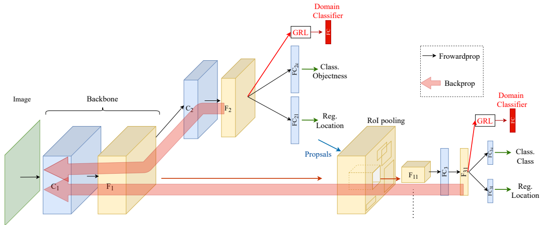
Figure 4.3 – Our domain adaptation for Faster R-CNN. See text for details.
