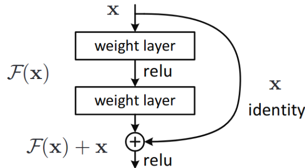
Figure 2.4 – Residual block (Figure from [2]).
