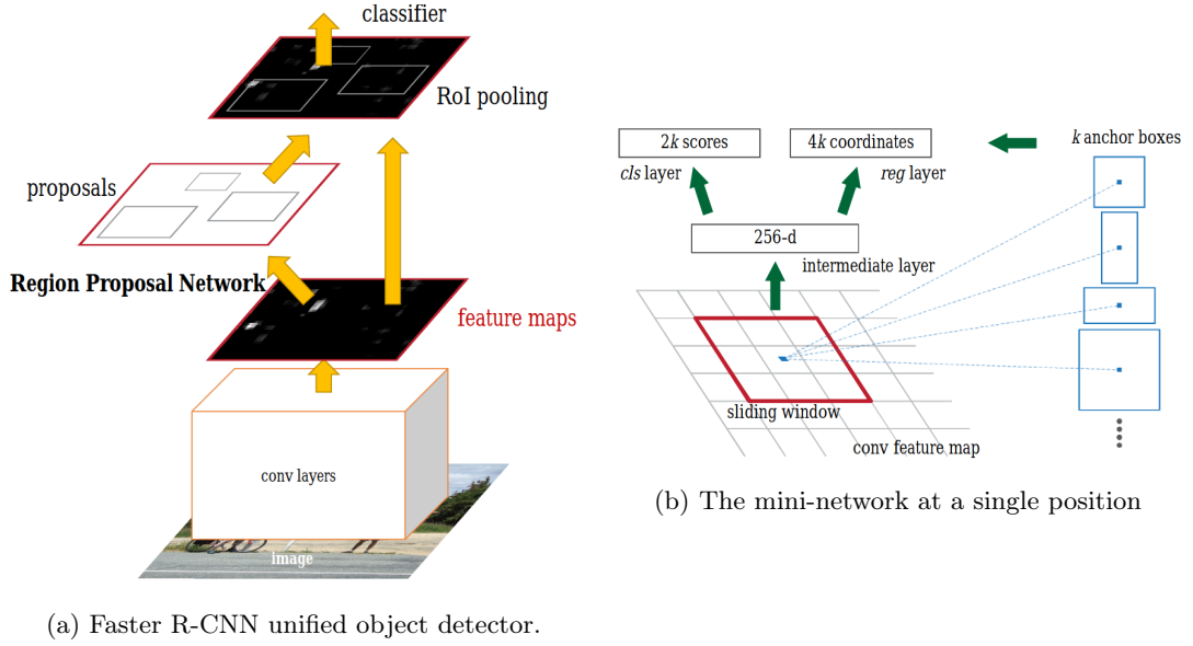
Figure 3.2 – Faster R-CNN model (Figures from [3]).
