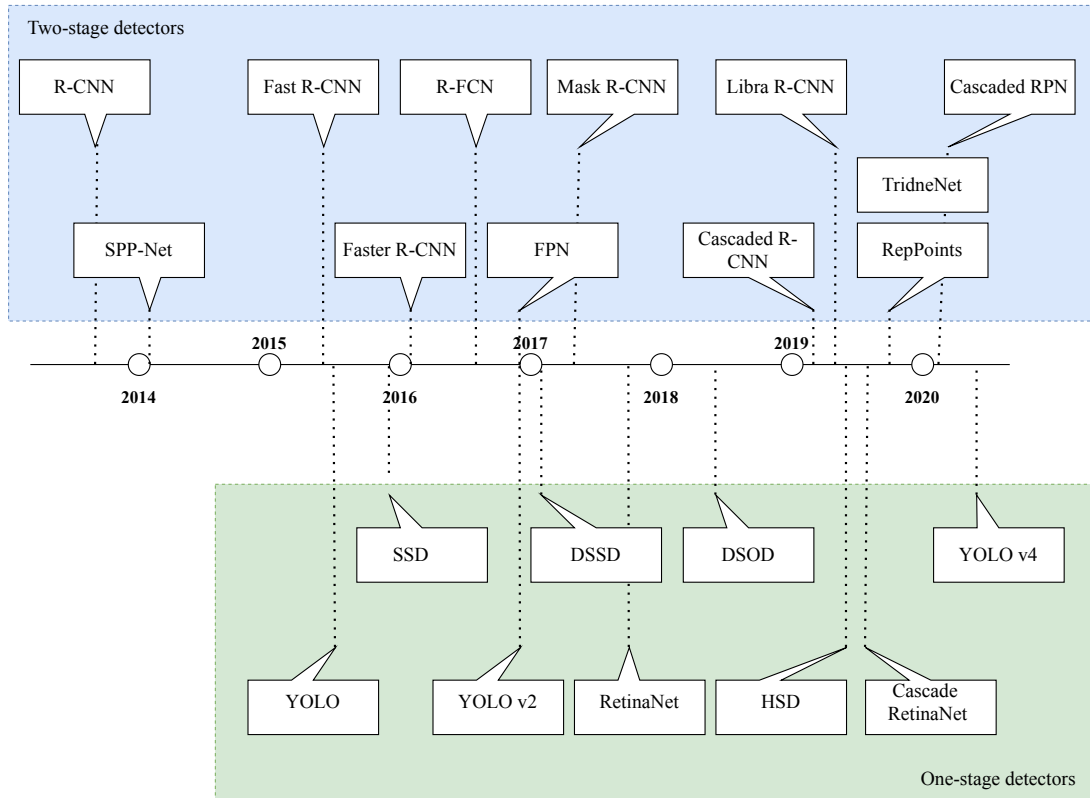
Figure 2.5 – Timeline of leading object detection frameworks into their two categories: (1) two-stage and (2) one-stage.
