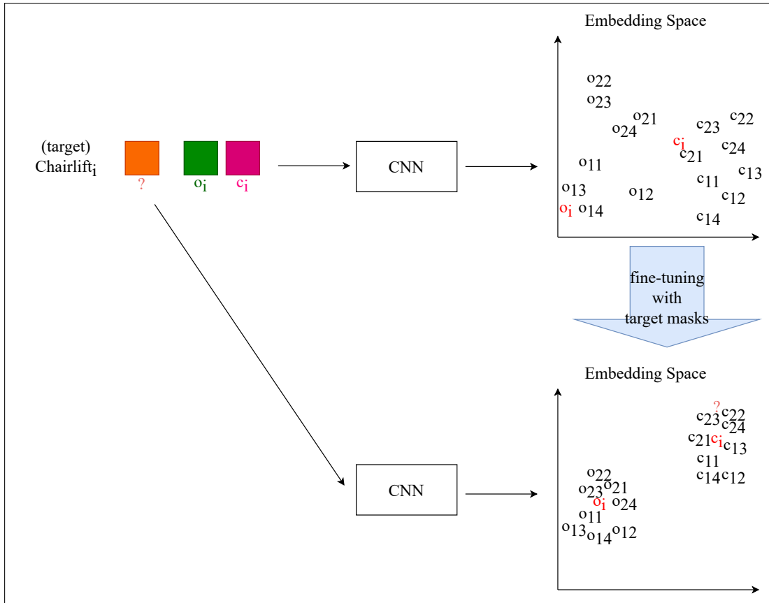
Figure 6.5 – Fine-tuning step with target masks.
