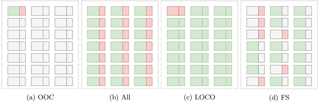
Figure 3.3 – Experimental settings. Each small rectangle represents one chairlift, the training set in green and the test set in red.
