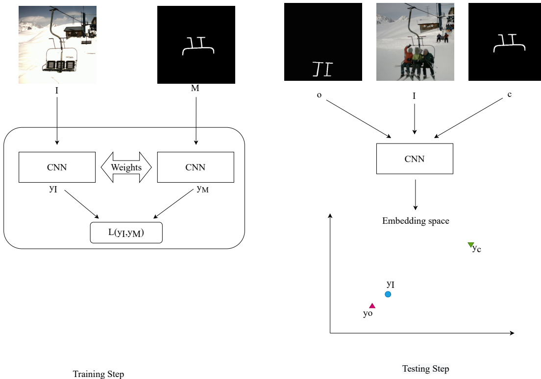
Figure 5.3 – Principle of our Mask-Guided image classification approach using Siamese networks.
