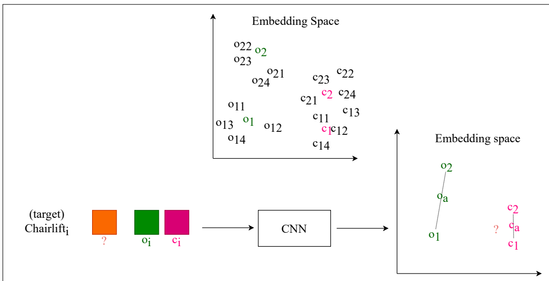
Figure 6.4 – Test on the target domain with average source masks as reference.
