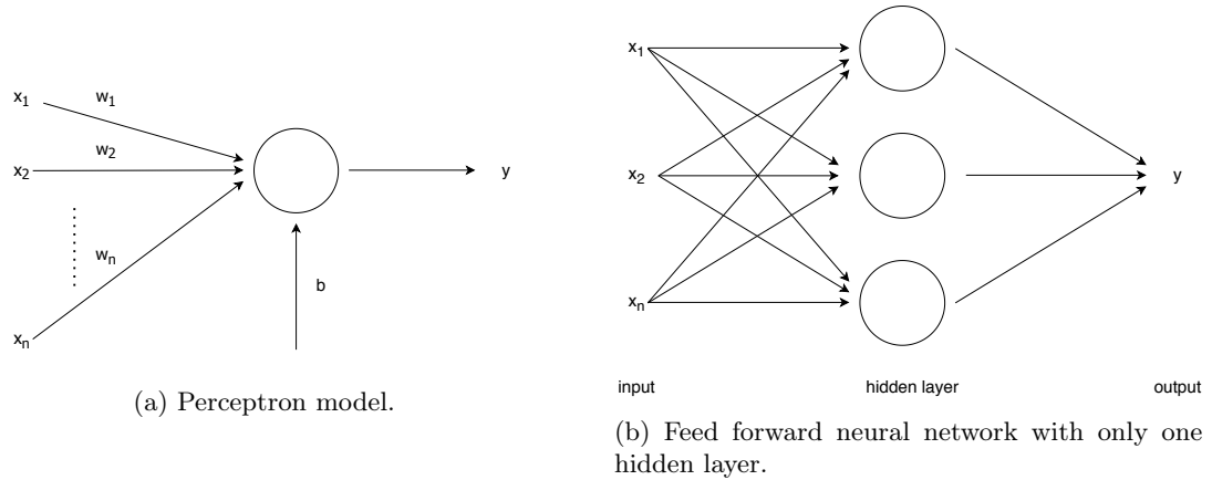
Figure 2.2 – Perceptron and multilayer perceptrons.
