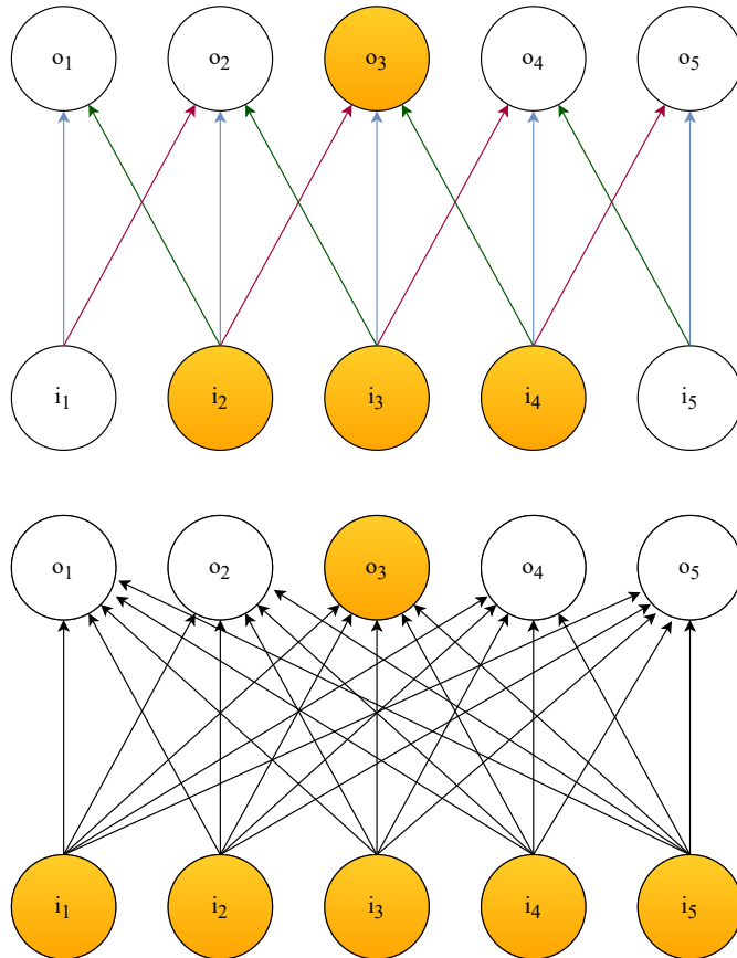
Figure 2.3 – Sparse connectivity and weight sharing. Convolution (top): the green, blue and red arrows indicate uses of the first, second and third (respectively) element of a 3-element kernel, each element is used at all inputs i.e. weight sharing. Because the kernel size is 3, each output unit is affected by only 3 input units. For example, the highlighted input units i_2, i_3 and i_4 affect the highlighted output unit o_3 , and this is the receptive field of o_3 i.e. sparse connectivity. Fully connected (bottom): each black arrow indicates an element of the weight matrix, note that each arrow is used only once i.e. no weights sharing. Each output unit is affected by all the inputs. For example, o_3 is affected by i_1, i_2, i_3, i_4 and i_5 i.e. no sparse connectivity.
