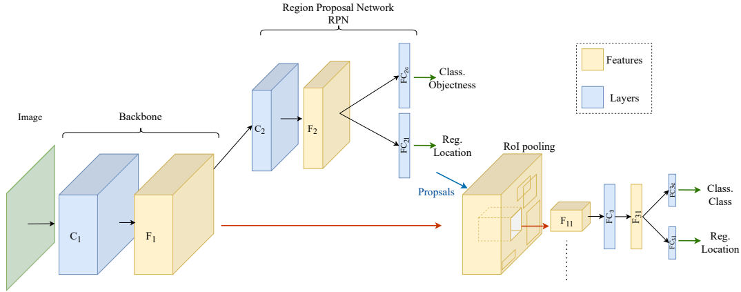
Figure 4.2 – Faster R-CNN Workflow.
