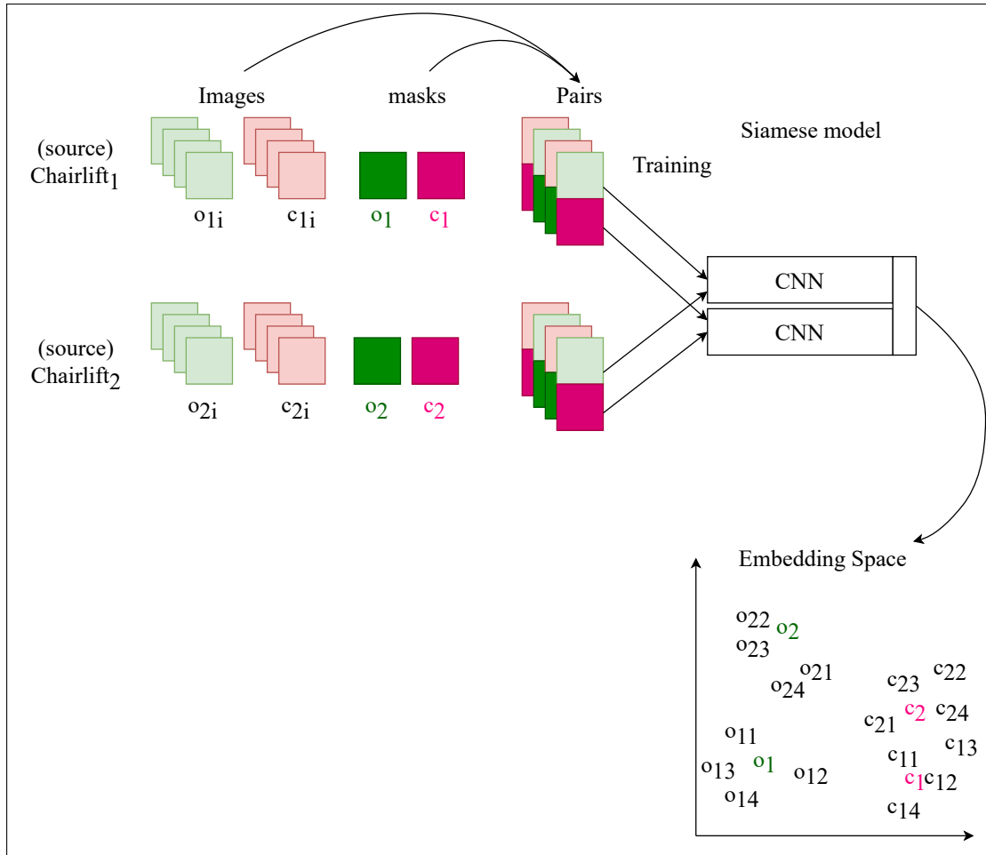
Figure 6.2 – Train on the source domain with image-mask pairs.
