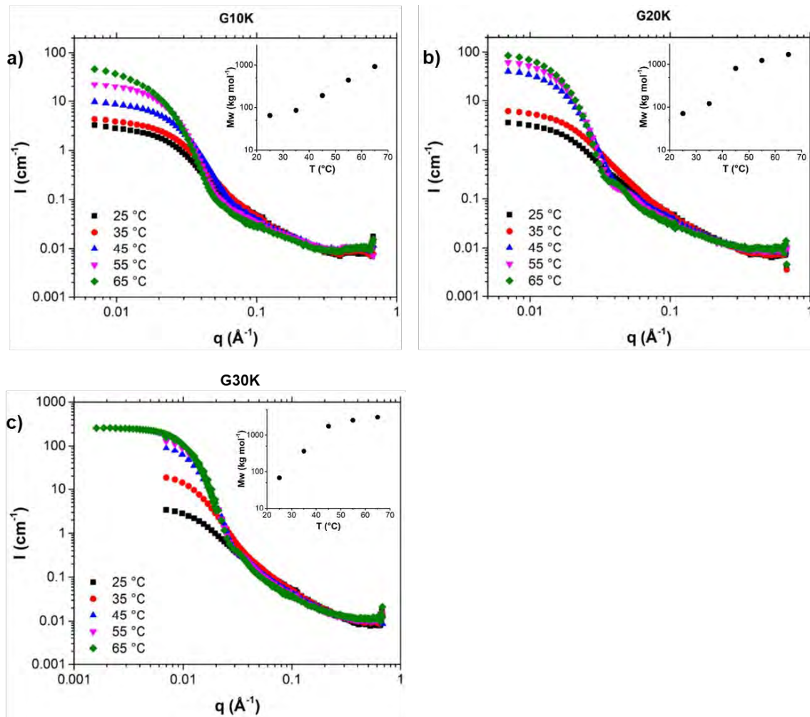
Figure 4.14. SANS curves at different temperatures for gradient copolymers a) 10 \text{kg mol}^{-1} , b) 20 \text{kg mol}^{-1} and c) 30 \text{kg mol}^{-1} . Concentration = 1 wt% in \text{D}_2\text{O} .
