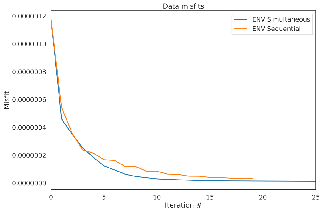
FIGURE 5.8: Data Misfits for the different inversion strategies. Sequential inversion method was not able to decrease the misfit after 19 iterations.
