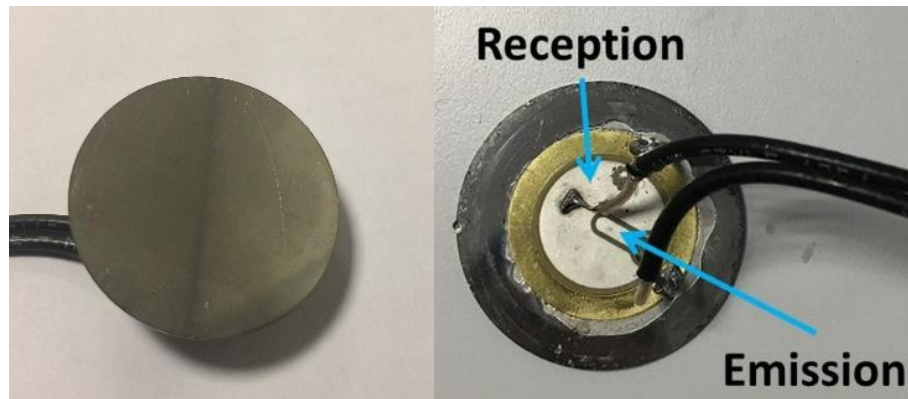
FIGURE 4.3 – Piezoelectric transducer used for the acquisition
