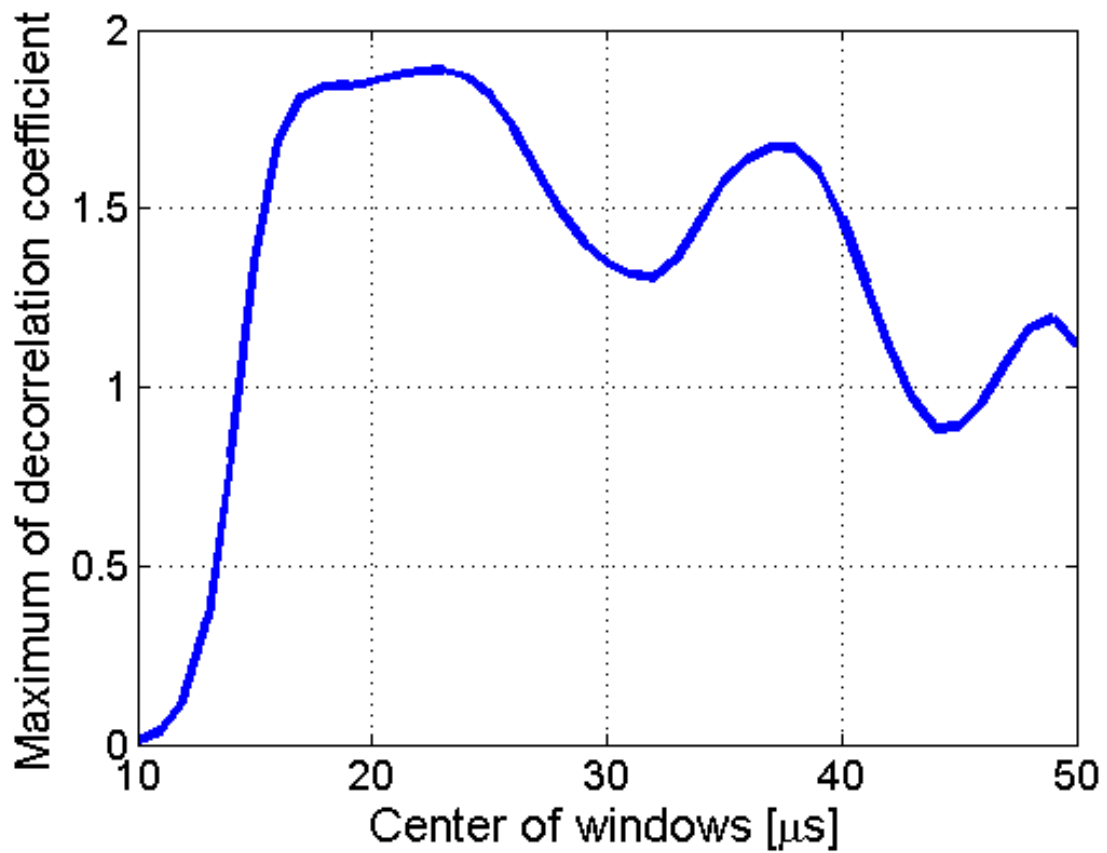
FIGURE 3.8 – The stable value (maximum value) of the decorrelation coefficient as a function of the center of the windows. The windows are always 10 \mu\text{s} wide.
