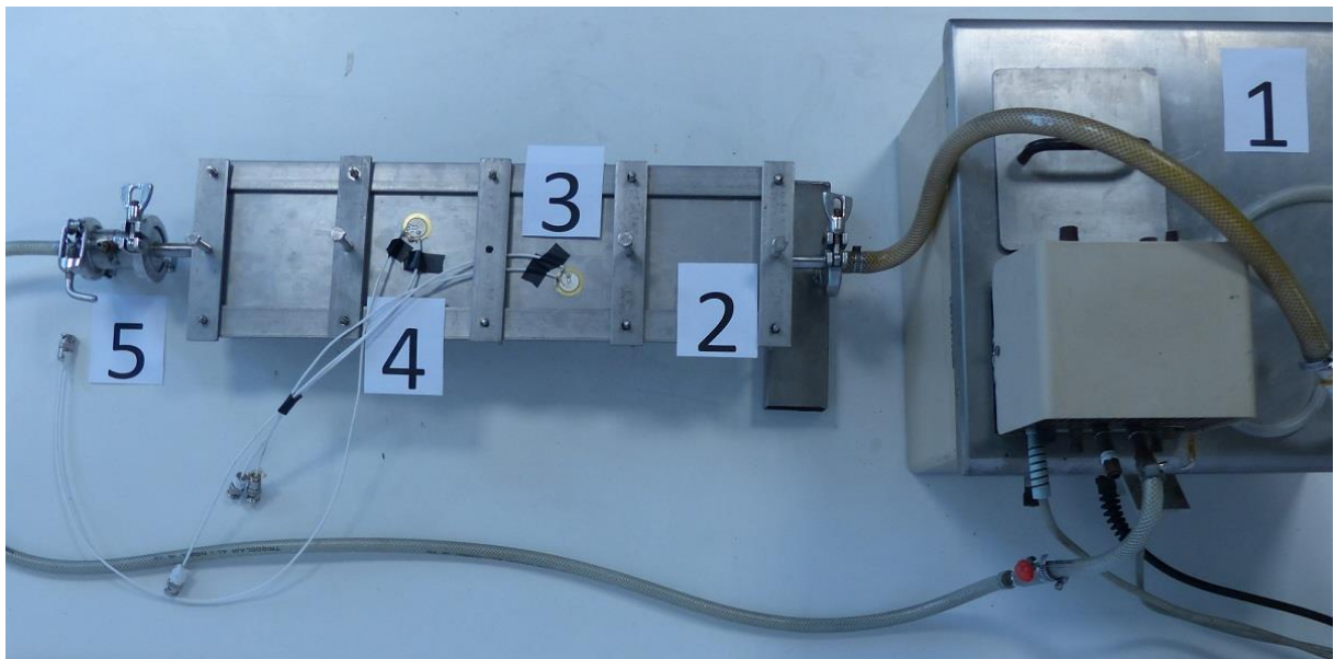
FIGURE 3.1 – Diagram of the monitoring system (top); Photo of the cleaning system (bottom), 1 : water bath; 2 : duct; 3 : measurement sensor with wax; 4 : control sensor without wax; 5 : connection of duct and hosepipe with thermometer
