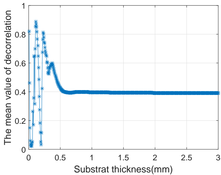
FIGURE 2.7 – Mean value of decorrelation coefficient with different time windows in function of the substrate thickness.
