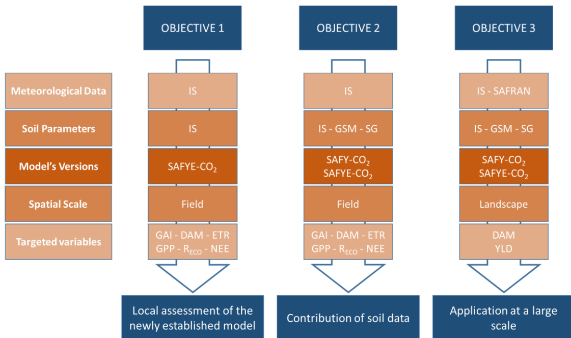
Figure II-9 : Summary of the validation strategy in terms of upscaling the SAFY-CO 2 and SAFYE-CO 2 models. IS is in situ, GSM is GlobalSoilMap and SG is SoilGrids.
