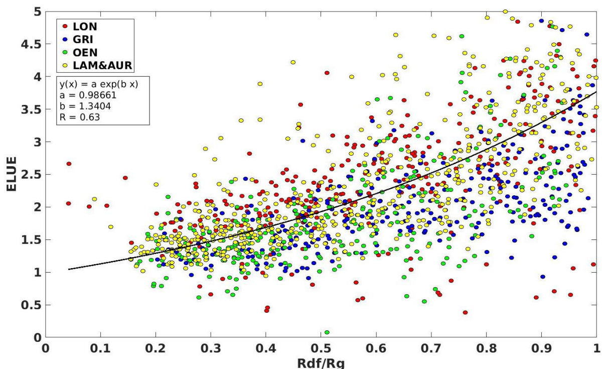
Figure I-14 : Relationship between the ELUE and the ratio between diffuse (Rdf) and global (Rg) radiation measured at 5 European flux sites (Lonze, Grignon, Oensingen, Lamasquère & Auradé).
