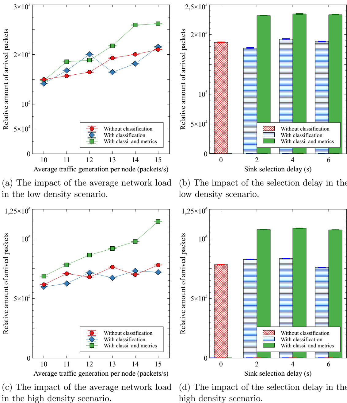
Figure 4.13: The relative amount of packets that reached their final destination.
