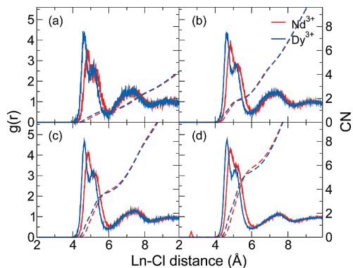
Figure 4. Ln–Cl radial distribution functions (solid lines) and coordination number (dashed lines) obtained for binary aqueous solutions of \text{NdCl}_3 (red) and \text{DyCl}_3 (blue) at different concentrations: (a) 0.5, (b) 1.0, (c) 2.0, and (d) 3.0 mol \text{kg}^{-1} .
