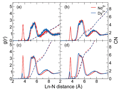
Figure 5. Ln–N radial distribution functions (solid lines) and coordination numbers (dashed lines) obtained for binary aqueous solutions of \text{Nd}(\text{NO}_3)_3 (red) and \text{Dy}(\text{NO}_3)_3 (blue) solutions at different concentrations: (a) 0.5, (b) 1.0, (c) 2.0, and (d) 3.0 mol \text{kg}^{-1} .
