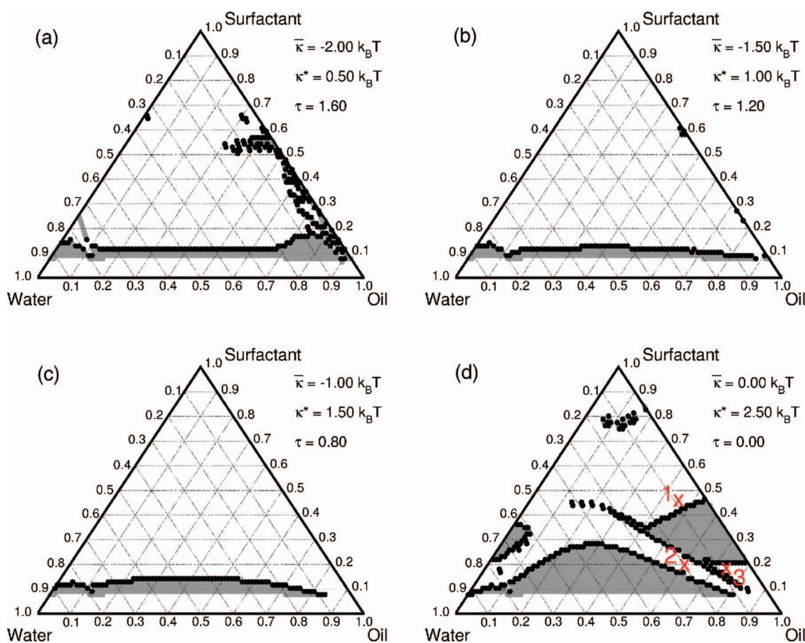
FIG. 2. Ternary stability diagrams calculated for \kappa = 1.25 k_B T and \bar{\kappa} = (a) -2.00 , (b) -1.50 , (c) -1.00 , and (d) 0.00 k_B T , and a zero spontaneous curvature H_0 . Points represent the spinodal instabilities. The shaded areas at the bottom of the triangles are two- or three-phase domains. The unshaded areas correspond to stable one-phase microemulsions. Compositions of points labelled (1), (2), and (3) in the (d) panel are given in Table I.
