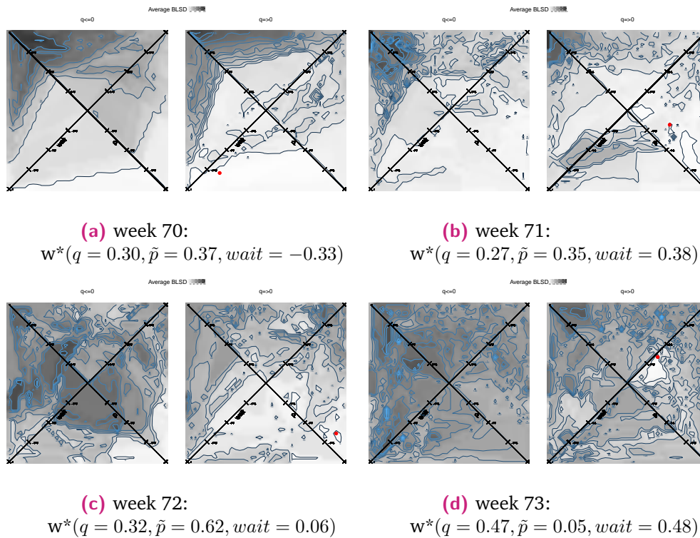
Fig. 5.4: Visualization of the search space for 4 consecutive weeks 70, 71, 72, and 73. The two diagonal axis represent \tilde{p} and wait . The lighter the area is, the better the performance (lower average BSLD ). The optimal area change from one week to the next. The red dot (in the lightest area) represents w^* and the blue triangle represents w^{*train} .
