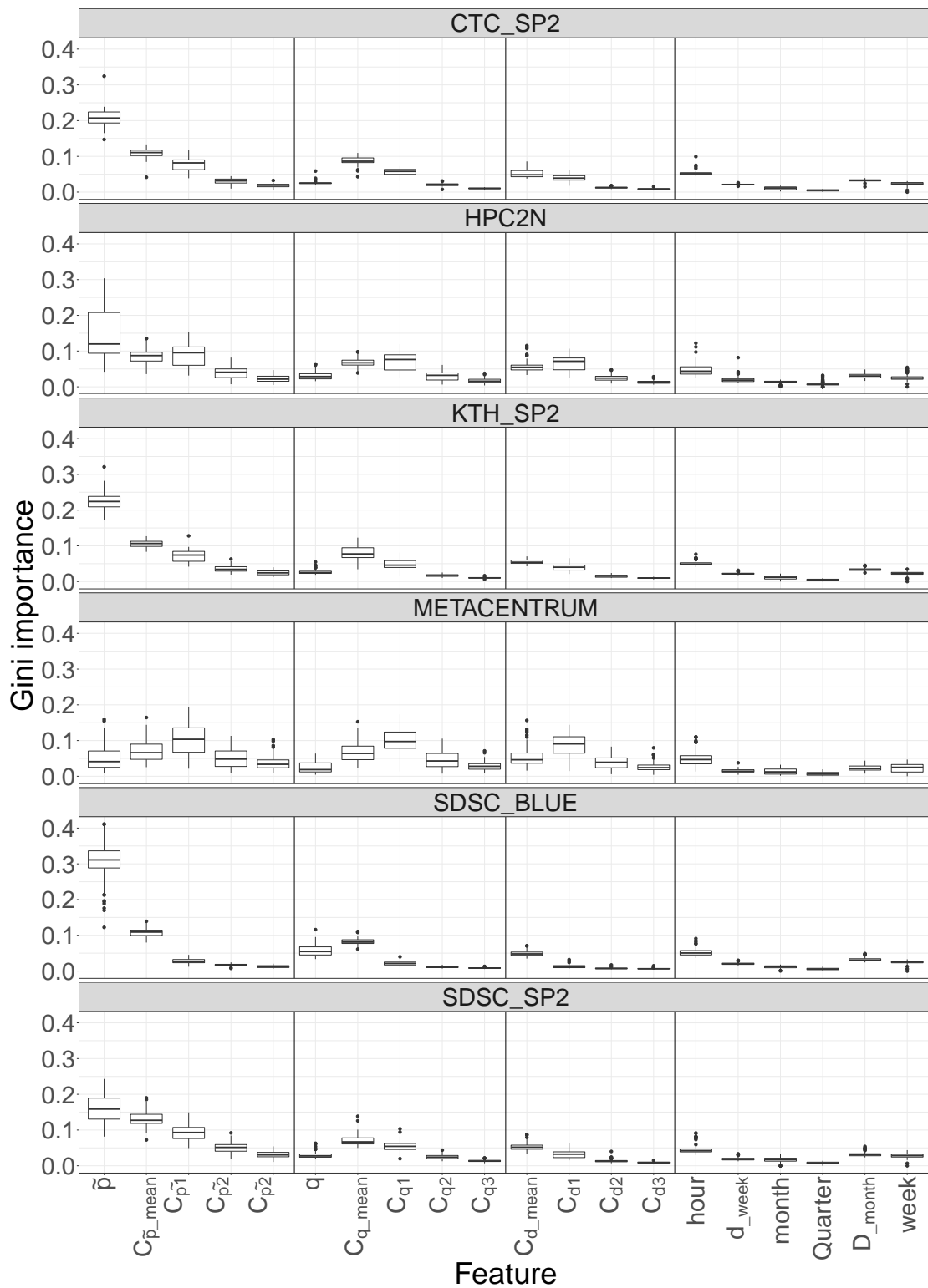
Fig. 6.5: Importance of individual features during the weekly learning process. The larger the weights, the more important the feature in the classification. Weights are normalized such that their sum equals 1.
