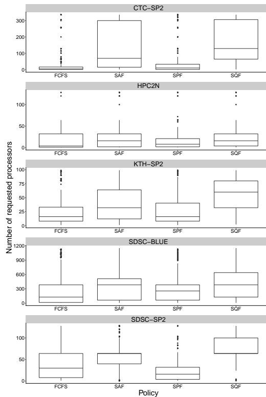
Fig. 4.2: Number of processors of the top 100 jobs with highest slowdown values.
