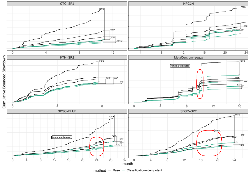
Fig. 6.7: Evolution of the Cumulative Bounded Slowdown for the six platforms, using the base policies (black) and the same policies augmented with job size classification and idempotence (cyan). The cumulative bounded slowdown is always such that SAF \approx SPF < WFP < FCFS , which is expected as prioritizing small jobs is known to optimize the average slowdown whereas FCFS rather bounds the largest waiting time. Since these heuristics solely rely on the requested runtime, they cannot be very efficient. Activating our classification-based prioritization systematically and significantly improves the performance of all heuristics at any point in time and not simply at the end of the evaluation period. In steady state (see SDSC-SP2), it is clear that the cumulative bounded slowdown increases more slowly when our classification-based mechanism is activated. It may happen that burst of jobs are submitted and incur sudden and large jumps in the cumulative bounded slowdown. These jumps are always significantly reduced (see Megacentrum-zegox) with our mechanism and even sometimes completely avoided (see SDSC-BLUE).
