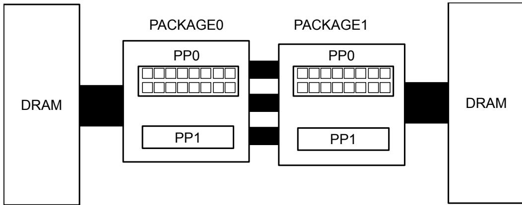
Fig. 7.1: Overview of the Intel RAPL architecture of a dual-socket system
