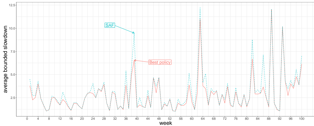
Fig. 5.6: SDSC-BLUE: Comparing SAF, the best pure policy on average, with the best pure policy for every week.
