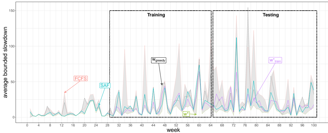
Fig. 5.3: Comparing the performance of various policies on the SDSC-SP2 trace. w^* represents the best policy in hindsight for every week. w^*_{train} is the policy obtained from learning on the Training weeks, and w_{greedy} gives the results of testing the best policy of one week on the next.
