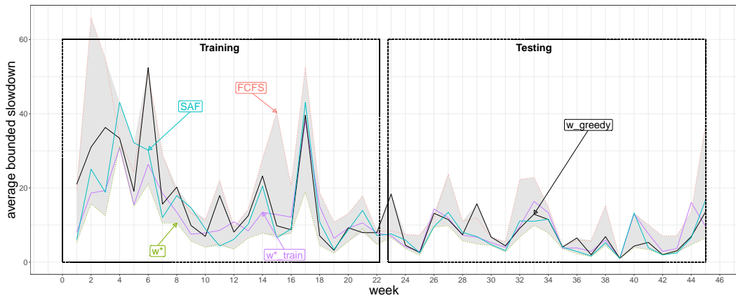
Fig. 5.13: KTH-SP2: comparing the performance of various policies. w^* present the optimal policy for every week. w_{train}^* is the optimal policy obtained from learning on the training weeks, and w_{greedy} is the results of testing the optimal policies of one week on the next.
