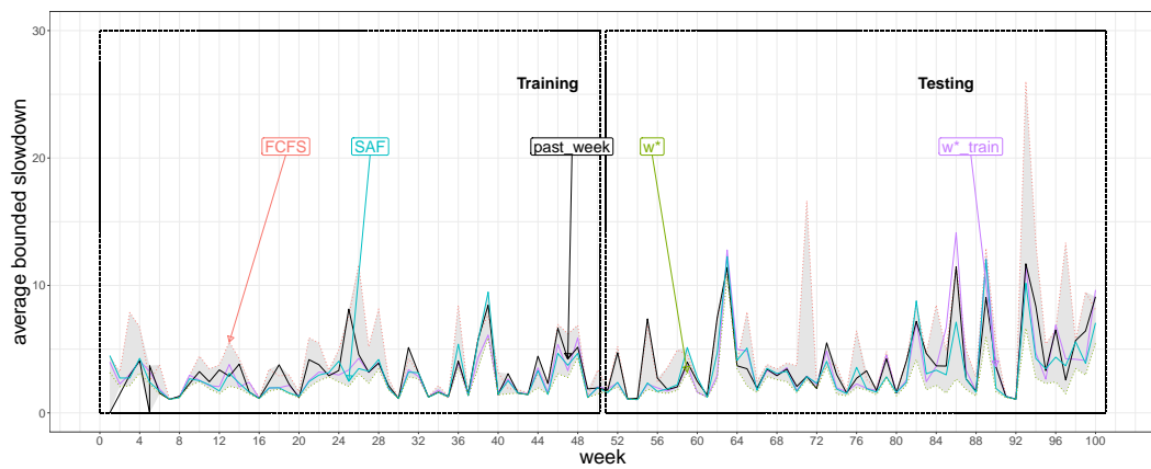
Fig. 5.7: SDSC-BLUE: Comparing the performance of various policies. w^* present the optimal policy for every week. w_{train}^* is the optimal policy obtained from learning on the training weeks, and w_{greedy} is the results of testing the optimal policies of one week on the next.
