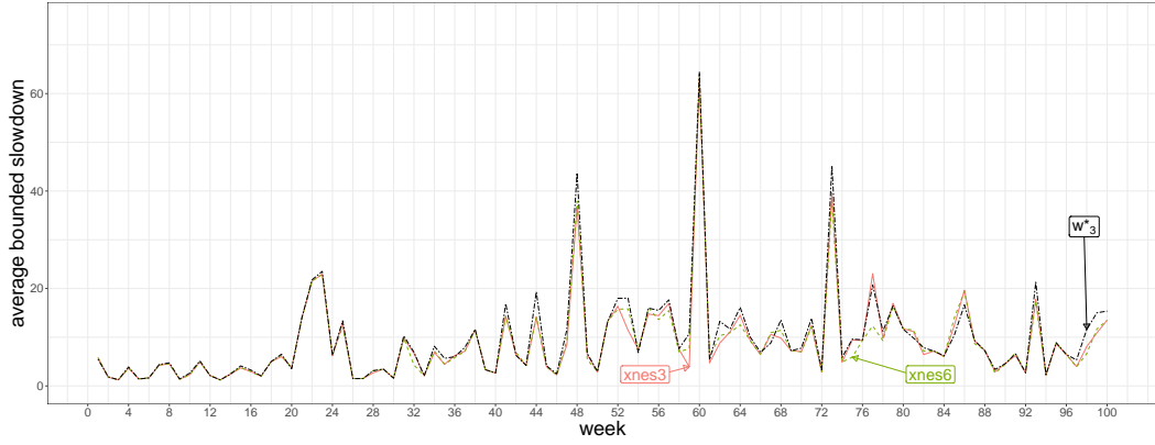
Fig. 5.5: Comparing average BSLD of the vectors of the 3 original features ( xnes3 ) with the extended vector of 6 features ( xnes6 ) and the minimum we obtain from space coverage ( w^*_3 )
