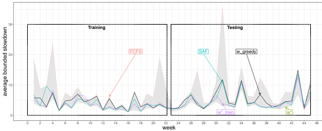
Fig. 5.10: CTC-SP2: comparing the performance of various policies on the CTC-SP2 trace. w^* present the optimal policy for every week. w_{train}^* is the optimal policy obtained from learning on the training weeks, and w_{greedy} is the results of testing the optimal policies of one week on the next.
