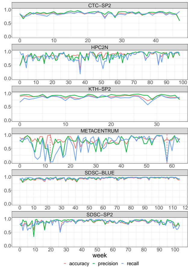
Fig. 6.4: Evolution of the quality of the learning for individual weeks
