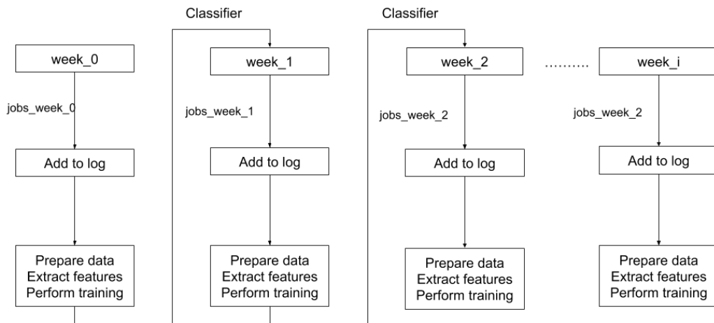
Fig. 6.3: Learning process: At the end of each week the new jobs are added to the dataset and a new training process is performed
