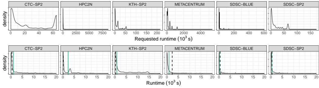
Fig. 6.1: Distribution of requested (upper row) and actual (bottom row) execution times of jobs for the six workload traces. (1) Note the scale/range difference on the X-axis, which indicates how the distribution of both variables are very different and shows that the requested runtime is a quite unreliable information. (2) The distribution of the actual runtime exhibits a sharp spike toward short jobs for all workloads. The green vertical line and the dashed black vertical line respectively represent the median value of the runtimes and the result of a clustering algorithm (Section 6.2) and allow to easily discriminate between “small” and “large” jobs.
