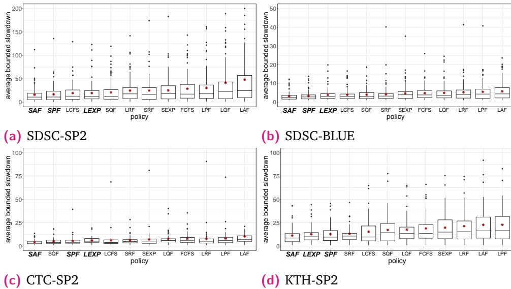
Fig. 5.1: Tukey box-plot of the weekly average bounded slowdown of pure policies for the 4 traces. The policies are sorted in an increasing order by the mean of the weekly average bounded slowdown for all the weeks. The three most efficient policies are highlighted.
