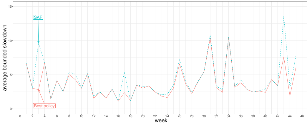
Fig. 5.9: CTC-SP2: comparing SAF, the best pure policy on average, with the best pure policy for every week.
