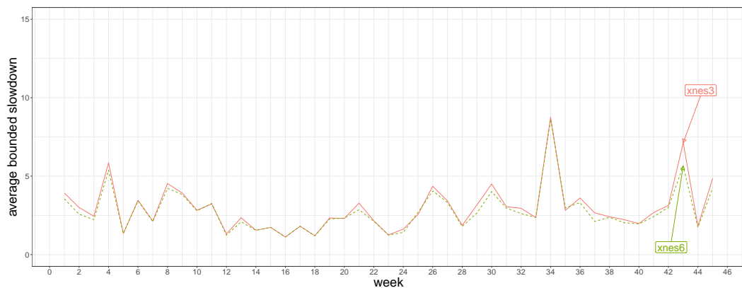
Fig. 5.8: SDSC-BLUE: Comparing average BSLD of the vectors of the 3 original features (xnes3) with the extended vector of 6 features (xnes6)
