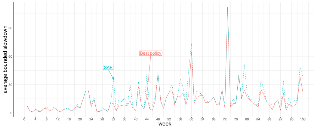
Fig. 5.2: Comparing SAF, the best pure policy on average, with the best pure policy for every week for the SDSC-SP2 trace.
