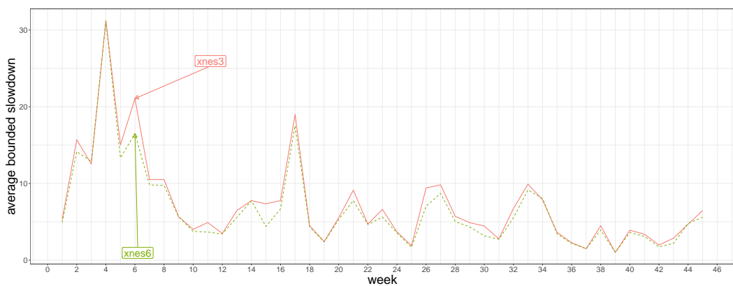
Fig. 5.14: KTH-SP2: comparing average BSLD of the vectors of the 3 original features (xnes3) with the extended vector of 6 features (xnes6)
