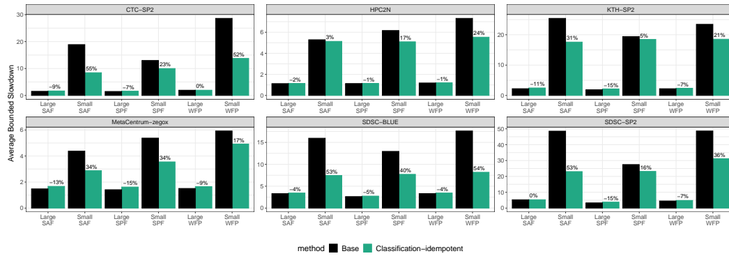
Fig. 6.8: Average bounded slowdown for small and large jobs, using the four base policies and the corresponding classification-idempotent schedulers. Breaking down the average bounded slowdown between small and large jobs allows to evaluate how both classes benefit from the classification and whether one is unfairly treated compared to the other. The benefit for the Small job class is huge and can go up to 55% while the loss for the Large job class never exceeds 15% (the higher losses always occur in trace/policies with extremely small base slowdown). The difference for Large jobs is therefore negligible and would be barely noticeable by users. Last, note that, although there are visible differences between the base policies (SAF, SPF, WFP, in black), they tend to vanish whenever using our classification (in green).
