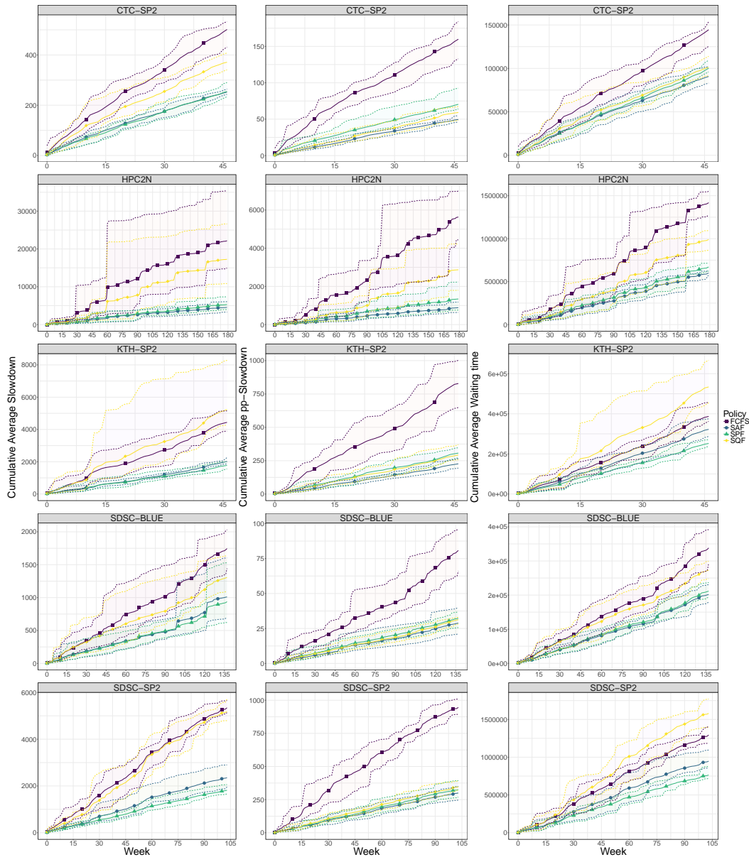
Fig. 4.1: Cumulative weekly average slowdown, pp-slowdown and waiting time: For each trace, the middle solid line represents the mean and the two dashed lines represent the lower and upper 10-90 percentiles.
