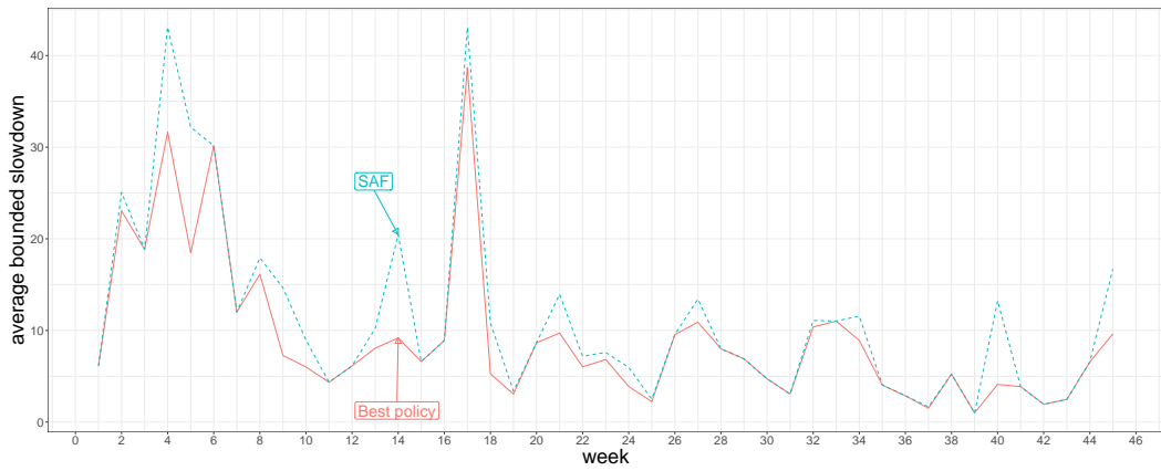
Fig. 5.12: KTH-SP2: comparing SAF, the best pure policy on average, with the best pure policy for every week.
