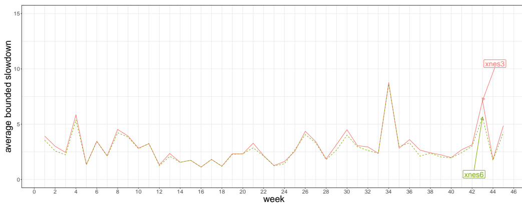
Fig. 5.11: CTC-SP2: comparing average BSLD of the vectors of the 3 original features (xnes3) with the extended vector of 6 features (xnes6)
