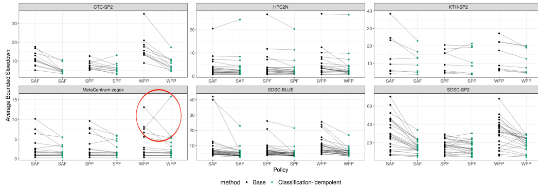
Fig. 6.6: Monthly average bounded slowdown. Each line links the values from the same month when using the base and classification-idempotent schedulers.
