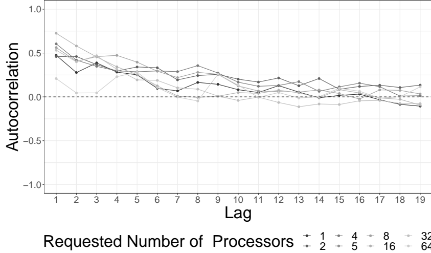
Fig. 6.2: Each category c allows to extract a series (ordered by submission dates) of actual runtimes p^{(c)} for which we can estimate the autocorrelation coefficient for each lag value l as follows: \rho_{p^{(c)}}(l) = \frac{\frac{1}{n-l} \sum_{i=1}^{n-l} (p_i^{(c)} - \mu_{p^{(c)}}) \cdot (p_{i+l}^{(c)} - \mu_{p^{(c)}})}{\sigma_{p^{(c)}}^2} , where \mu_{p^{(c)}} and \sigma_{p^{(c)}} are respectively the sample average and sample standard deviation of p^{(c)} . This autocorrelation coefficient lies in [-1, 1] and indicates how strongly p_i^{(c)} is correlated with p_{i+l}^{(c)} . The graph illustrates how the distribution of the autocorrelation coefficient evolves with the lag between the jobs that belong to the same category (u, q) of a specific user.
