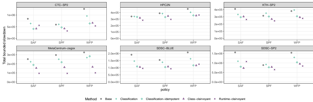
Fig. 6.9: Total accumulated bounded slowdown for the base schedulers (base), schedulers with perfect classification (class-clairvoyant), schedulers with classification and job-killing mechanism (classification-idempotent), and schedulers with perfect execution time information (runtimes-clairvoyant). Regardless the heuristic, it is interesting to note that, in general, Base \approx Classification > Classification-Idempotent \approx Class-clairvoyant > Runtime-clairvoyant, which is consistent with the fact that more accurate information allow to produce better schedules
