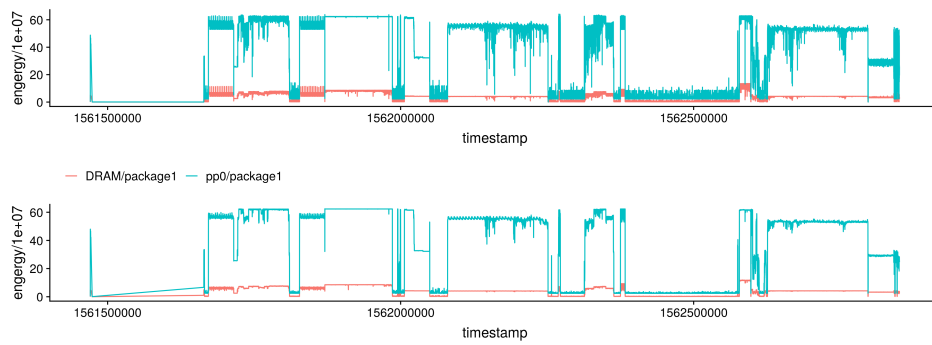
Fig. 7.4: Energy measurement aggregations; The upper figure represents the measurements as taken from Colmet. The bottom figure represents the results of the aggregation process.
