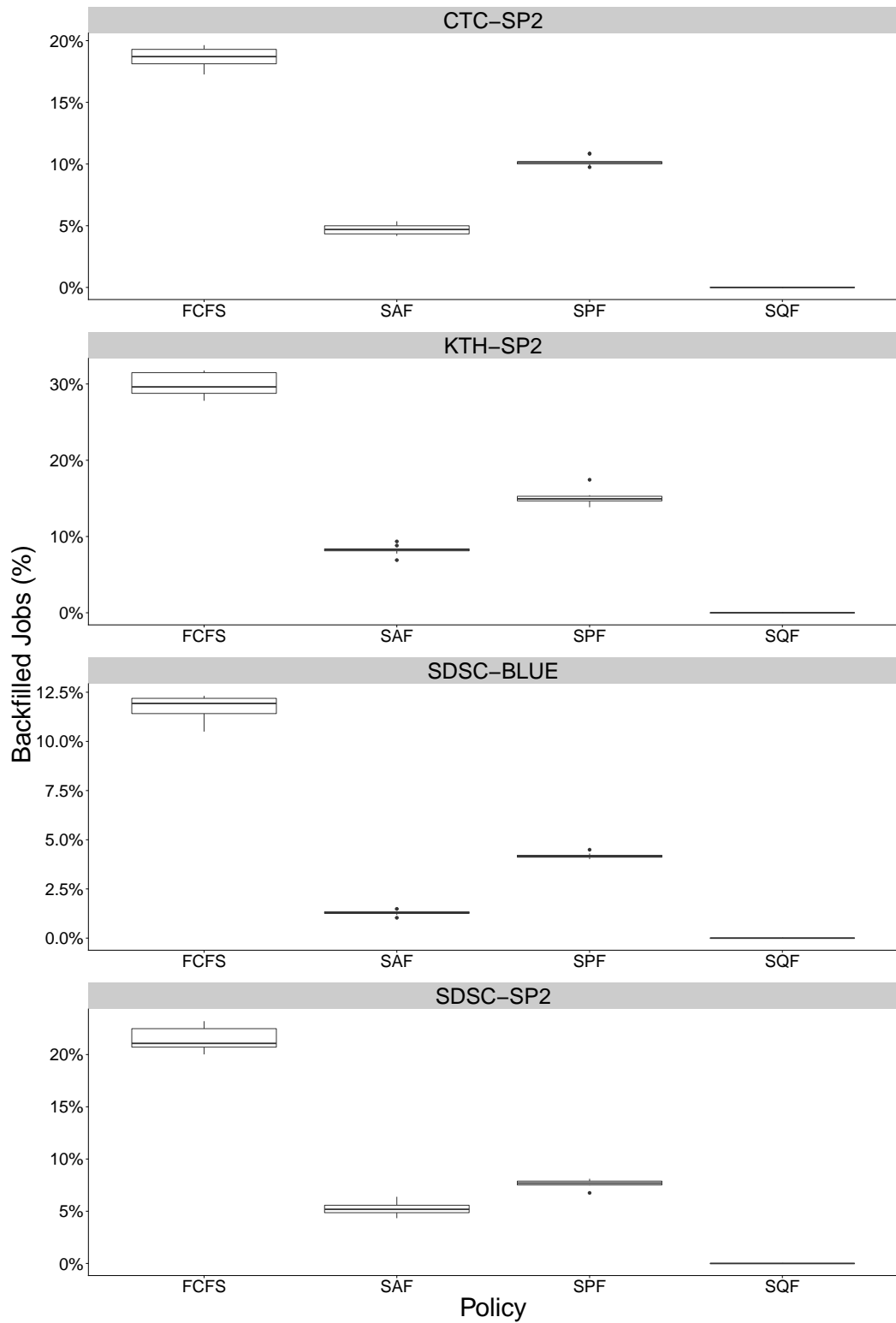
Fig. 4.4: Distribution of backfilled jobs between resamplings.
