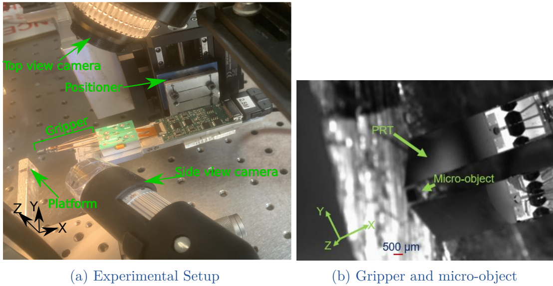
Figure V.6 – Experimental setup and the Gripper-object view
