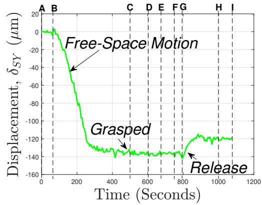
(c) Displacement of PRT tip
