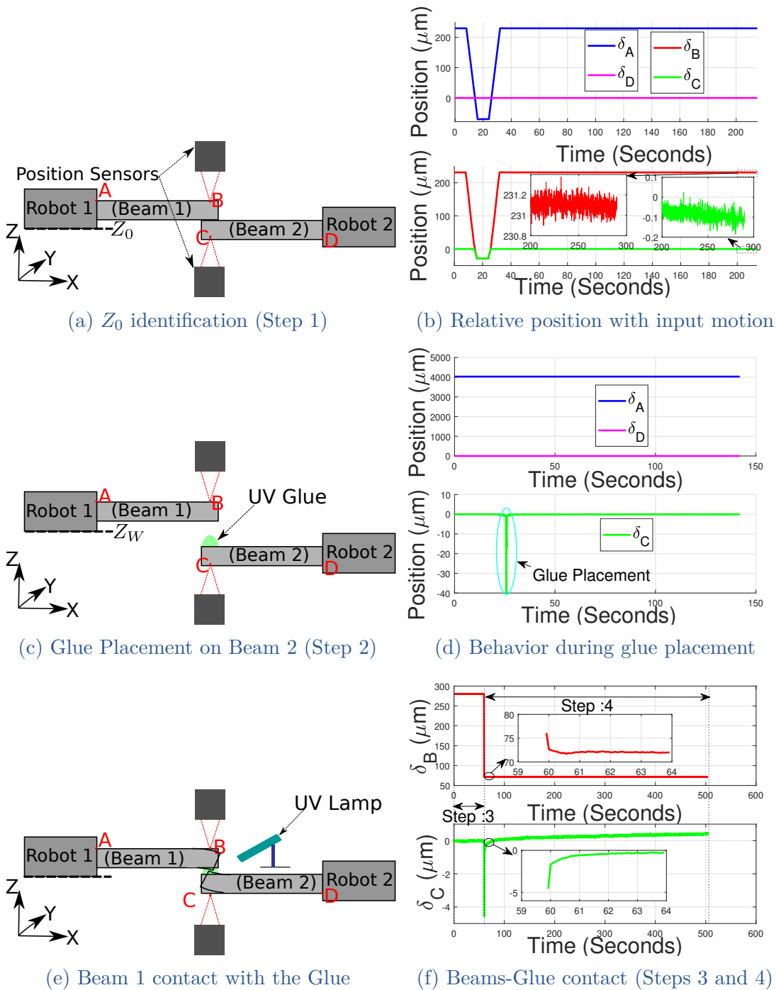
Figure II.16 – Different Steps before use of control
