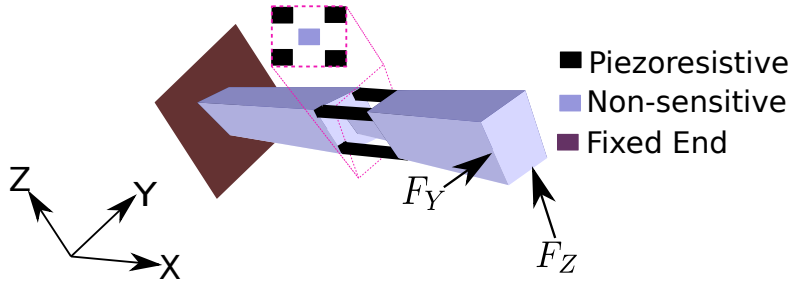
Figure IV.2 – Sensing Principle
