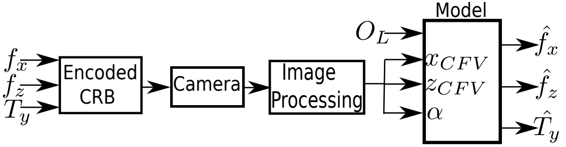
Figure III.3 – Principle scheme of the force-torque sensing platform
