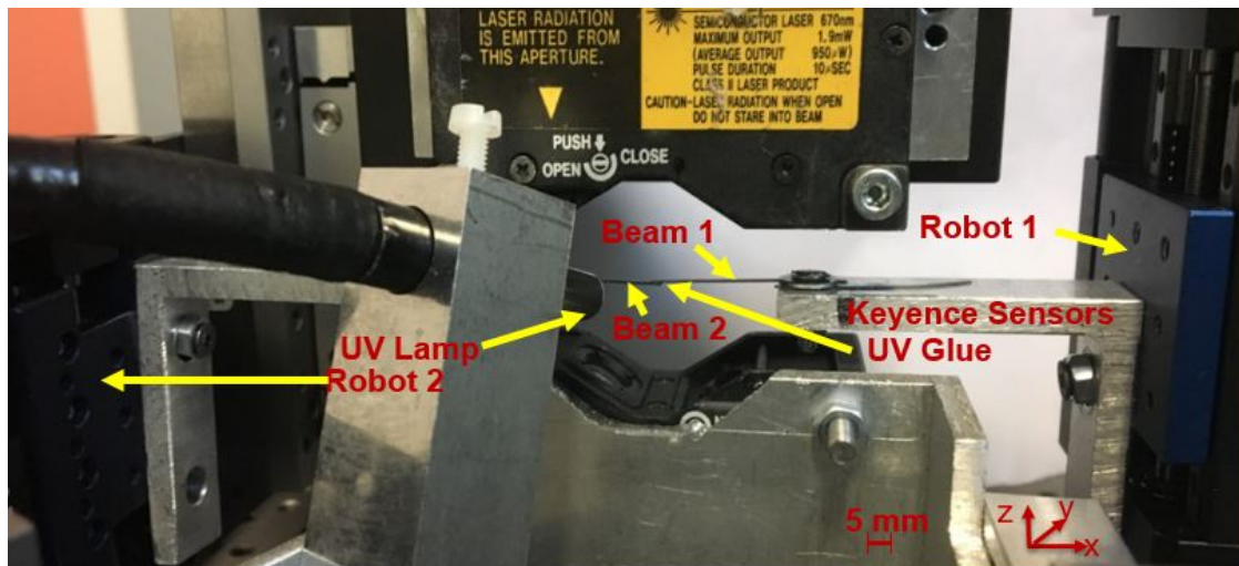
Figure II.14 – Experimental Setup used for the analysis
