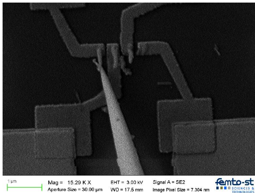
Figure I.2 – Electrical characterization of a carbon nano-tube in contact with a probe [Clévy 19]
