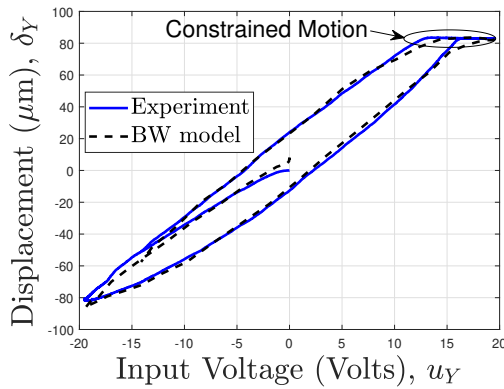
(a) Along Y, Actuation with Hysteresis
