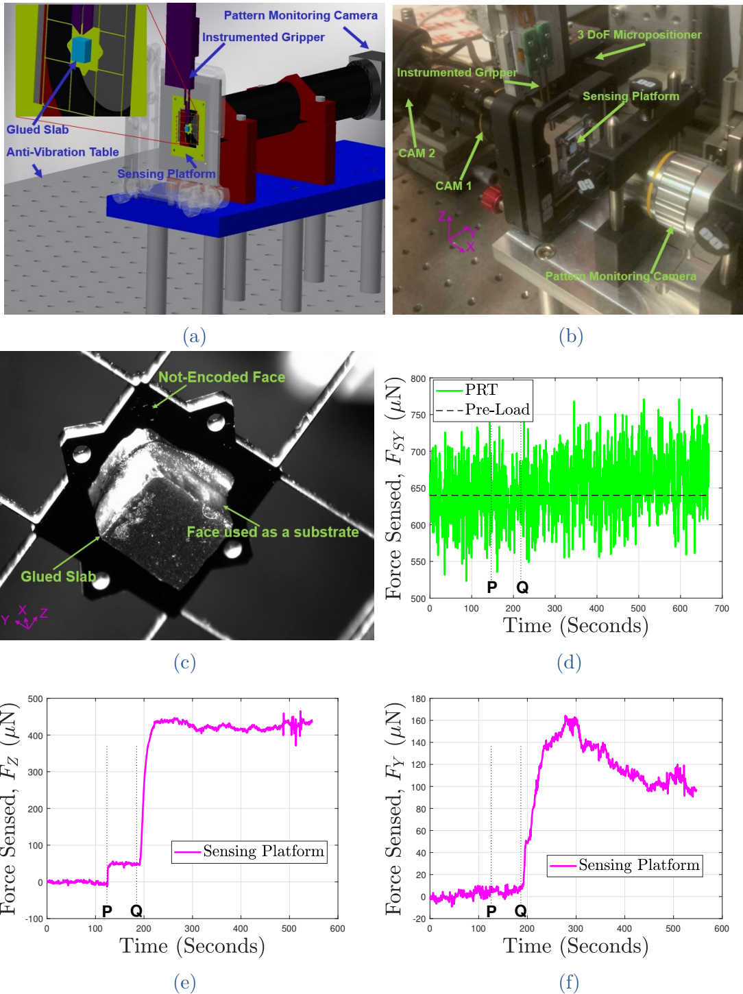
Figure V.9 – Gluing with developed micro-systems; (a) CAD version of the gluing system; (b) Experimental Setup; (c) Sensing platform with Slab; (d) Force sensed by PRT along Y (P: glue-slab contact, Q: UV ON); (e) Force sensed by sensing platform along Z; (f) Force sensed by sensing platform along Y
