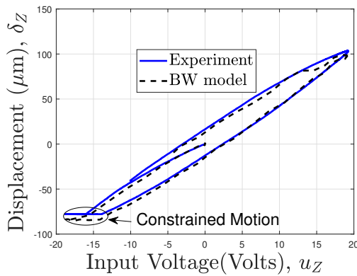
(c) Along Z, Actuation with Hysteresis
