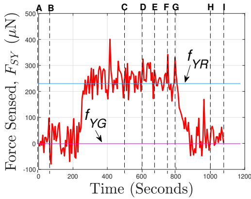
(b) Force sensed by PRT
