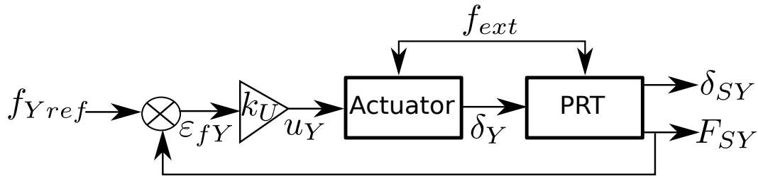
(a) Force controlled gripping and release scheme
