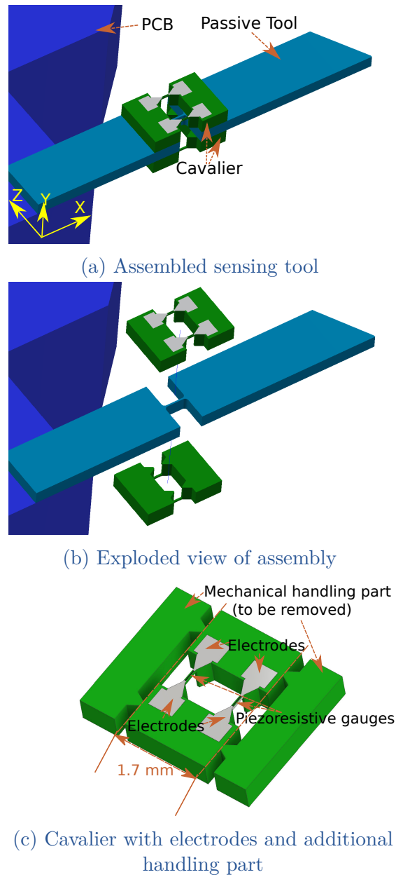
Figure IV.3 – Proposed design of the sensing tool
