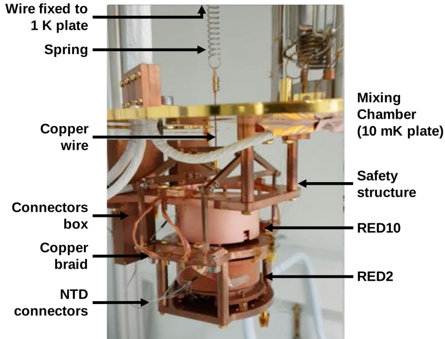
Figure 2.4: Photo of the suspended tower containing the two 200 g bolometers RED10 and RED2. This device mechanically decouples the detector load from the mixing chamber while assuring its thermalization. Figure taken from [39].
