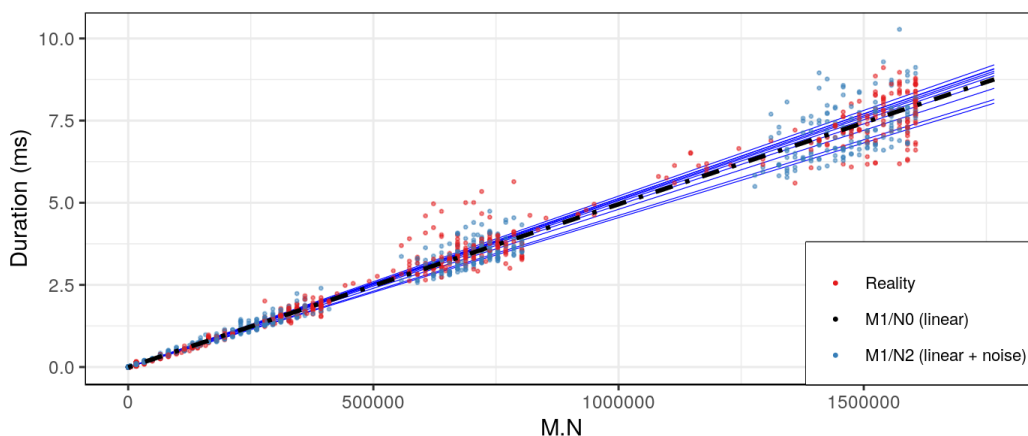
Figure 5.2.: Illustrating the realism of modeling for HPL_d1atcpy function.
