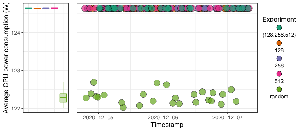
Figure 10.14.: Average CPU power consumption, observed on CPU 1 of dahu-5 , each point represents one experiment.
