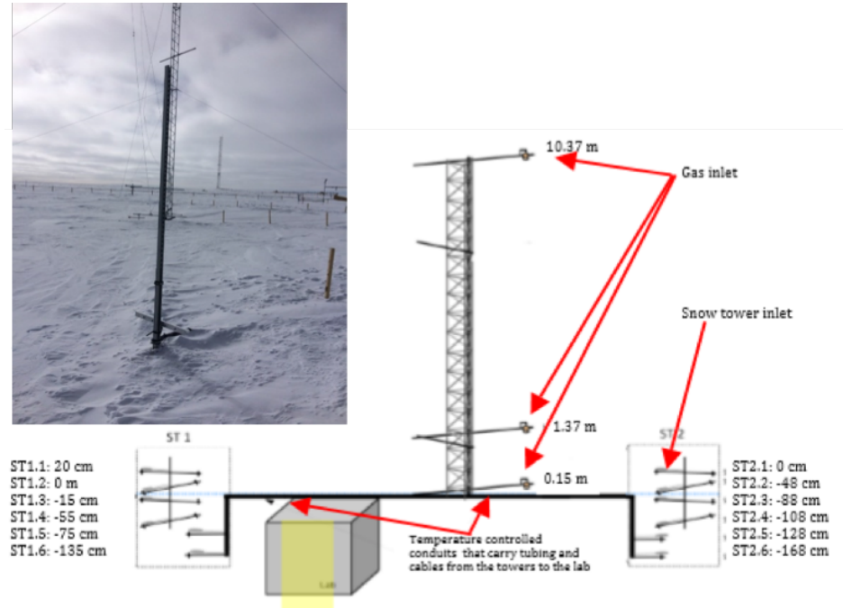
Figure B.6 – Snow-Tower installation at Dome C.
