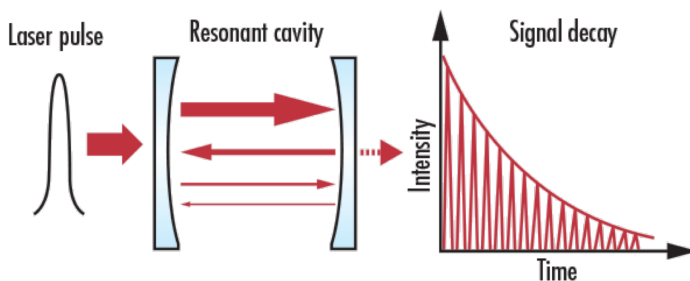
Figure 1.12 – Principle of CRDS
