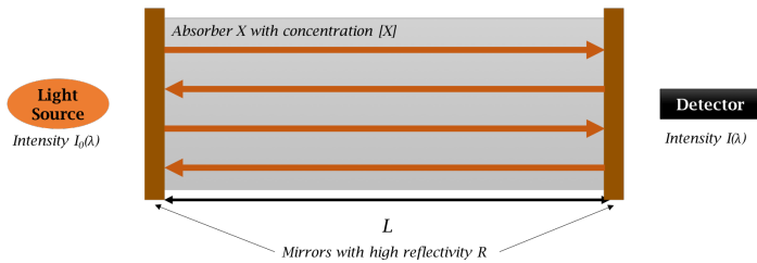
Figure 1.11 – Principle of an optical cavity
