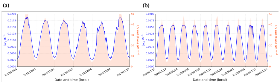
Figure 4.4 – J_{NO_2} (blue solid lines) reconstruction following the 2 degrees polynomial regression fit with UV radiations (shaded orange) measured by a broadband UV radiometer, spectral range 305–385 nm for both December (a) and January (b) observation periods.
