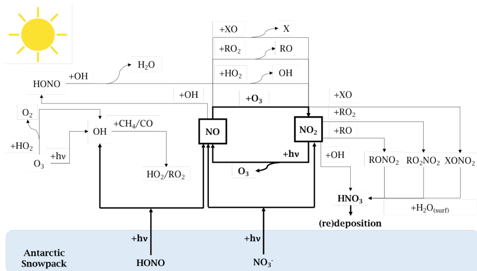
Figure 4.1 – Schematic of the gas phase chemistry of \text{NO}_x in the Antarctic Plateau. In bold the \text{NO}_x cycle and the \text{NO}_x direct snow-sources.
