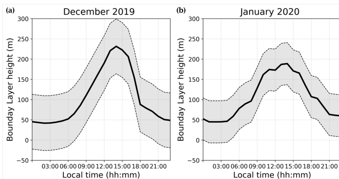
Figure B.10 – Atmospheric Boundary Layer height (PBL) (solid lines) ± 1 \sigma (dashed lines) estimated for both periods by the MAR regional model.
