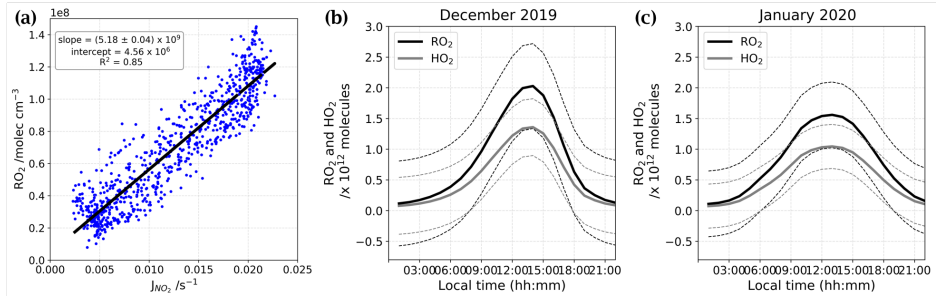
Figure B.9 – (a) linear correlation between RO 2 and J_{NO_2} taken from Kukui et al. (2014) . (b) and (c) total number of molecules of RO 2 (black) and HO 2 (grey) estimated for both periods of observations.
