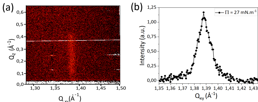
Figure 4.27: (a) The GIXD diffraction map and (b) the integrated intensity over Q_z of the GIXD signal from (GO + IL)_{NMP} Langmuir mixed film at \Pi = 27 \text{ mN.m}^{-1} .
