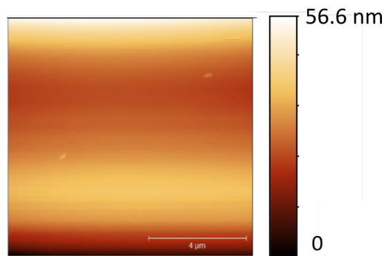
Figure 3.6: AFM topographic image measured on [\text{C}_{20}\text{mim}]^+[\text{NTf}_2]^- Langmuir-Blodgett film deposited on \text{Si}/\text{SiO}_2 at \Pi = 15 \text{ mN.m}^{-1} .
