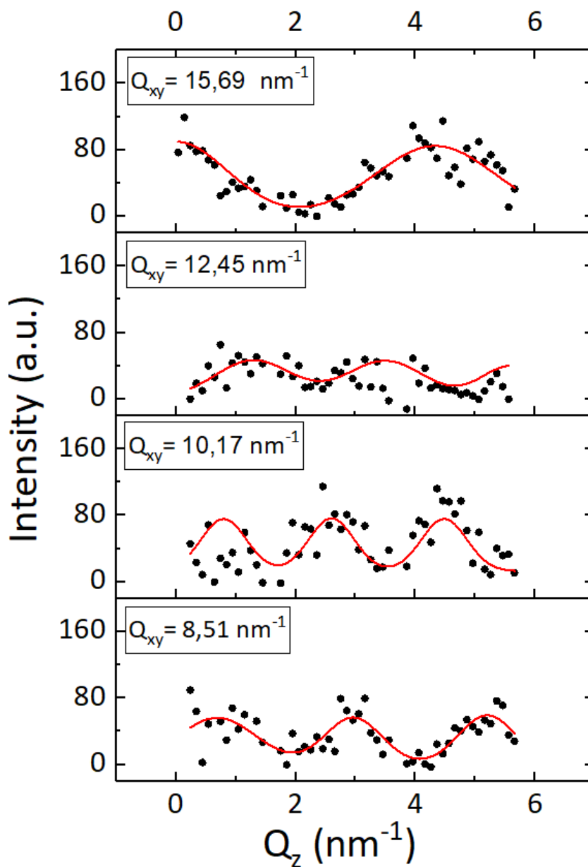
Figure 5.28: "Profile B" of the rods of the diffraction peaks relative to the organization of the inorganic structure coexisting with the IL Langmuir film at \Pi = 35 \text{ mN}\cdot\text{m}^{-1} .
