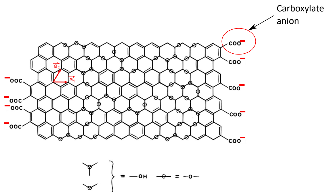
Figure 3.15: The structure of GO sheet dispersed in water. It shows the formation of carboxylate anions at its edges as a result of deprotonation of carboxyl groups in water.
