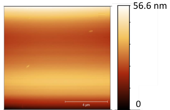
Figure 3.6: AFM topographic image measured on [\text{C}_{20}\text{mim}]^+[\text{NTf}_2]^- Langmuir-Blodgett film deposited on \text{Si}/\text{SiO}_2 at \Pi = 15 \text{ mN}\cdot\text{m}^{-1} .
