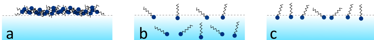
Figure 1.3: a. 3D film of amphiphilic molecules with hydrophobic tendency, b. Gibbs film and c. Langmuir film.
