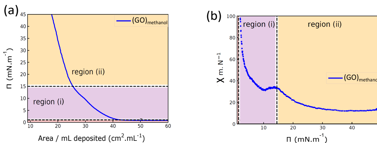
Figure 4.5: \Pi -A isotherm of (GO)_{methanol} Langmuir film deposited at the air-water interface at 20^\circ\text{C} (reproduced from [39], [99]).
