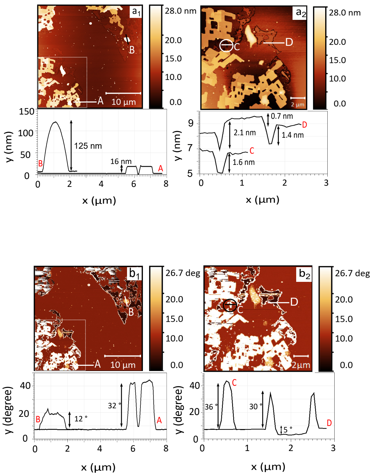
Figure 5.6: AFM topographic ( a_1 , a_2 ) and phase ( b_1 , b_2 ) images measured on [\text{C}_{20}\text{mim}]^+[\text{NTf}_2]^- Langmuir films, spread over a subphase containing 30 [\text{AuCl}_4]^-/\text{IL} transferred by Langmuir-Blodgett on Si/SiO 2 wafers \Pi = 32 \text{ mN}\cdot\text{m}^{-1} .
