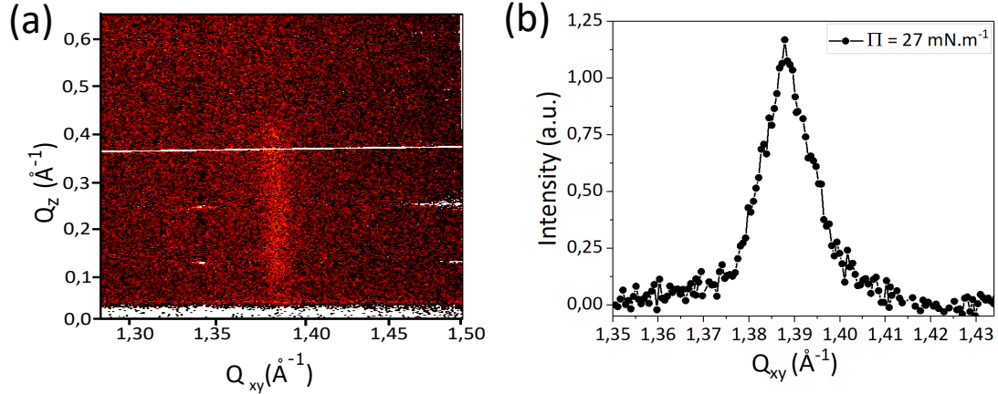
Figure 4.27: (a) The GIXD diffraction map and (b) the integrated intensity over Q_z of the GIXD signal from (GO + IL)_{NMP} Langmuir mixed film at \Pi = 27 \text{ mN.m}^{-1} .
