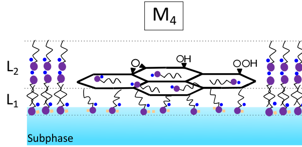
Figure 4.20: Schematic representation of the model M_4 describing the IL and GO stack configurations at \Pi = 21 \text{ mN.m}^{-1} .
