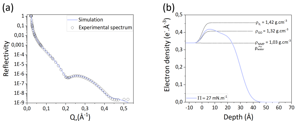
Figure 4.22: (a) XRR spectrum obtained at \Pi = 27 mN.m ^{-1} adjusted and (b) its corresponding electron density profile.
