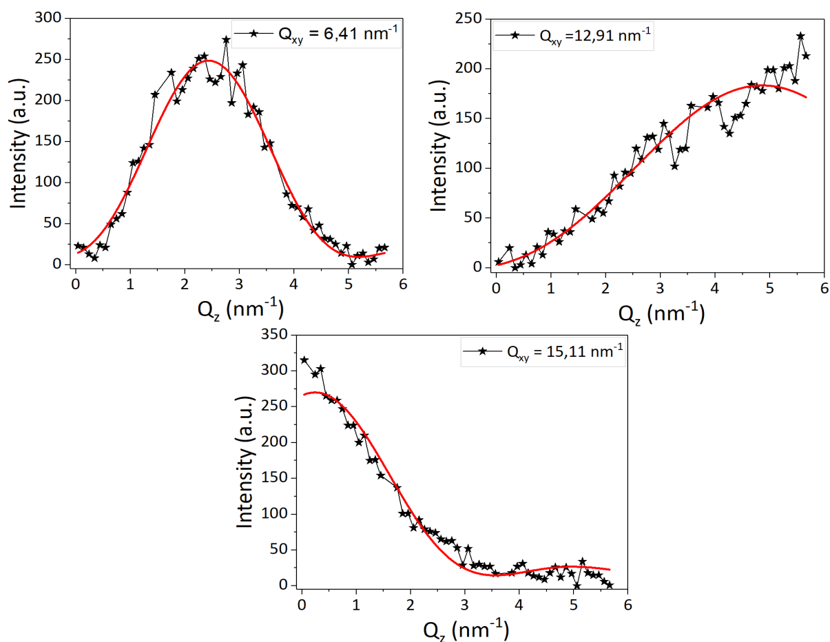
Figure 5.27: "Profile A" of the rodscaans of the diffraction peaks relative to the organization of the IL Langmuir film at \Pi = 35 \text{ mN}\cdot\text{m}^{-1} .
