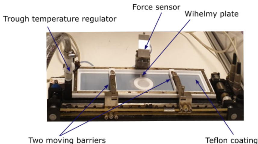
Figure 1.5: Photo of a Langmuir trough.
