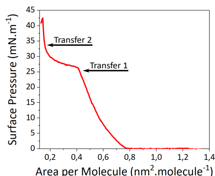
Figure 5.19: \Pi -A isotherm of the IL Langmuir film spread over a subphase containing 600 [\text{AuCl}_4]^-/\text{IL} .
