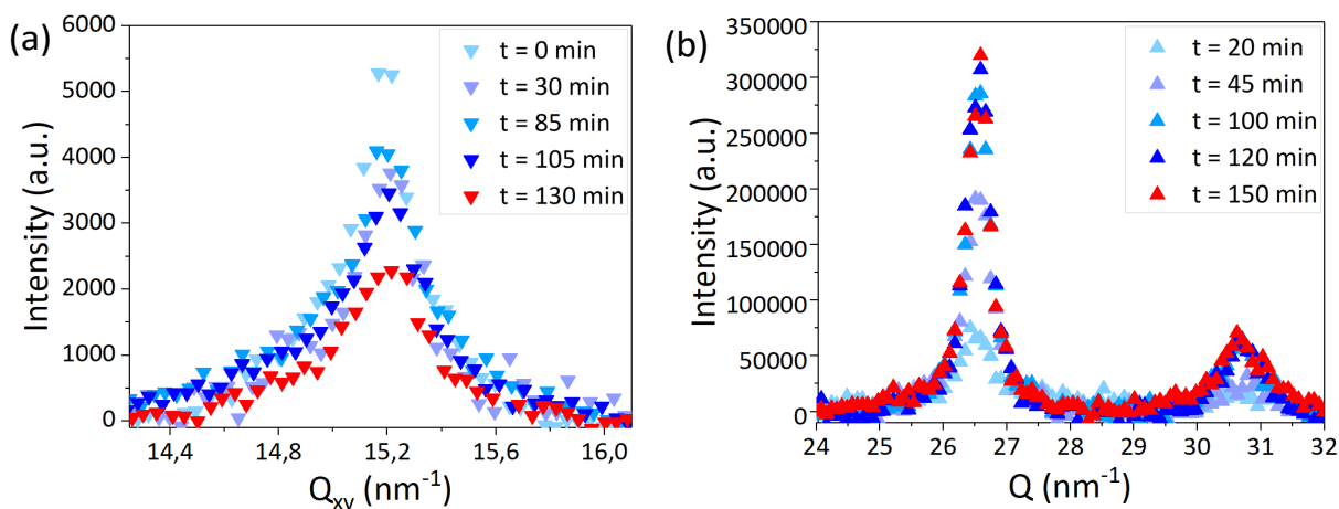
Figure 5.11: The GIXD signals as a function of the time irradiation coming from (a) the organic structure and (b) the inorganic structure.
