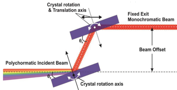
Figure 2.17: Schematic illustration of the double crystal monochromator in the beamline. This image is taken from [50].
