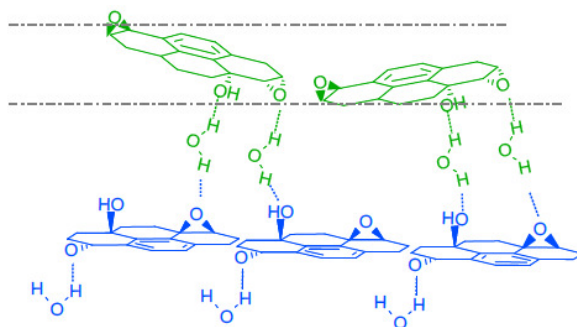
Figure 3.19: Schematic representation of the bilayer model of GO Langmuir film deposited on water surface as proposed by Bonatout et al.(reproduced from [39, 99]).
