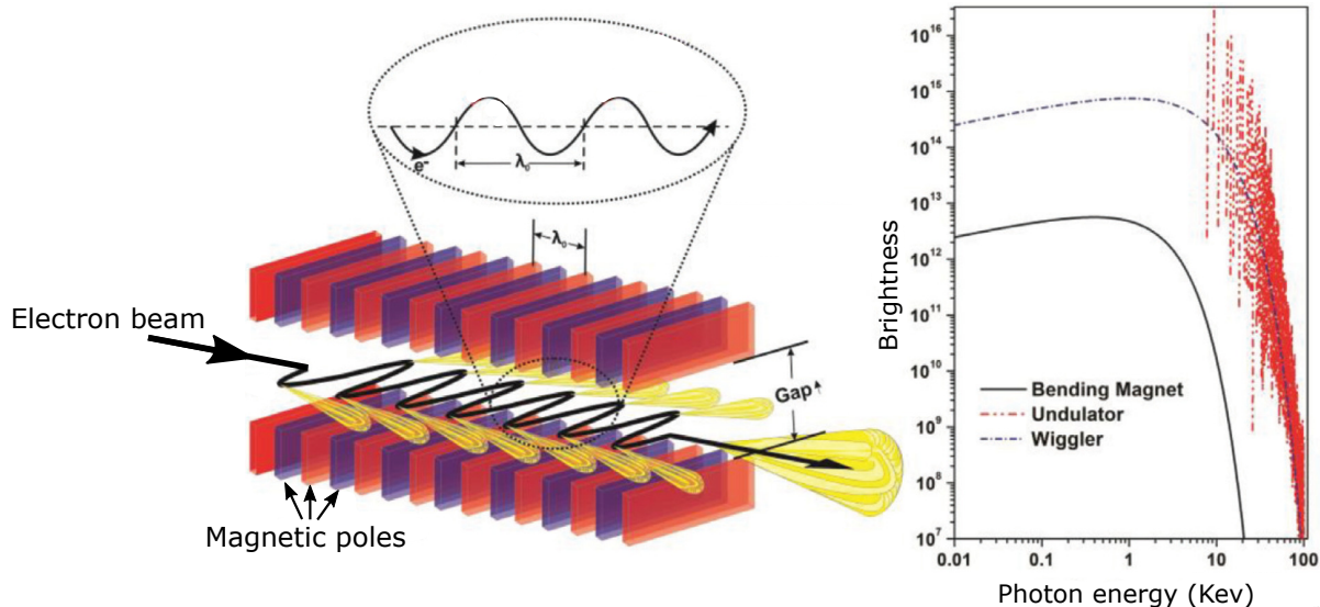
Figure 2.15: On the left, a diagram showing the movement of an electron beam through the wigglers inserted at the straight section of the storage ring. On the right, a spectrum comparing the brightness as a function of the energy of the synchrotron radiation emitted through the bending magnets, undulators and wigglers [50].
