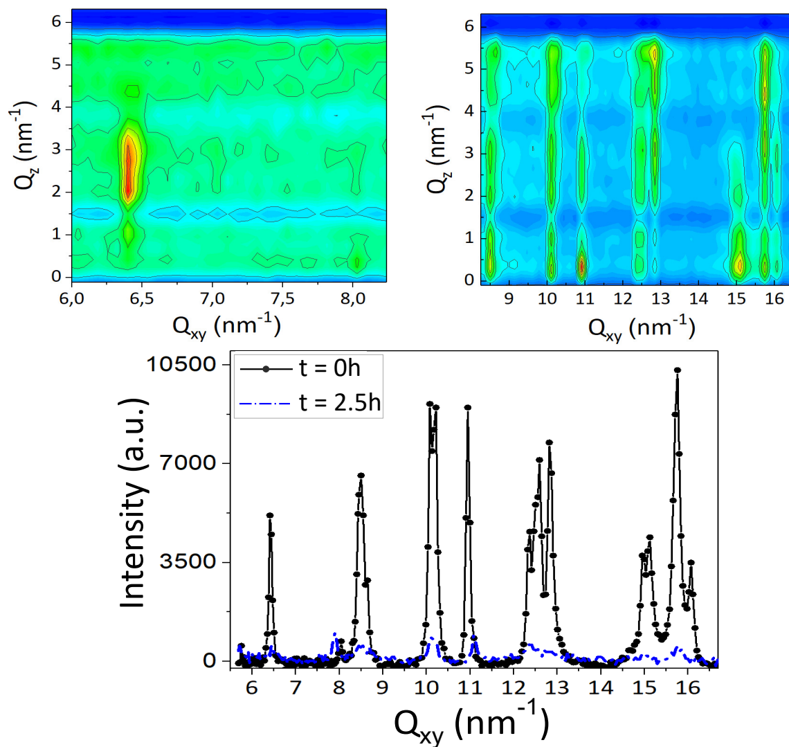
Figure 5.23: The X-ray diffraction (a) map and (b) intensities integrated over Q_z of the IL Langmuir film over a subphase containing 600 [\text{AuCl}_4]^- / IL, at \Pi = 20 \text{ mN}\cdot\text{m}^{-1} .
