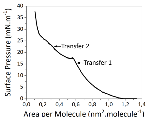
Figure 3.5: \Pi -A isotherm of [\text{C}_{20}\text{mim}]^+[\text{NTf}_2]^- Langmuir film deposited at the air-water interface.
