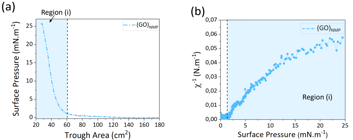
Figure 4.6: \Pi -A isotherm of (\text{GO})_{\text{NMP}} Langmuir film deposited at the air-water interface at 20^\circ\text{C} .
