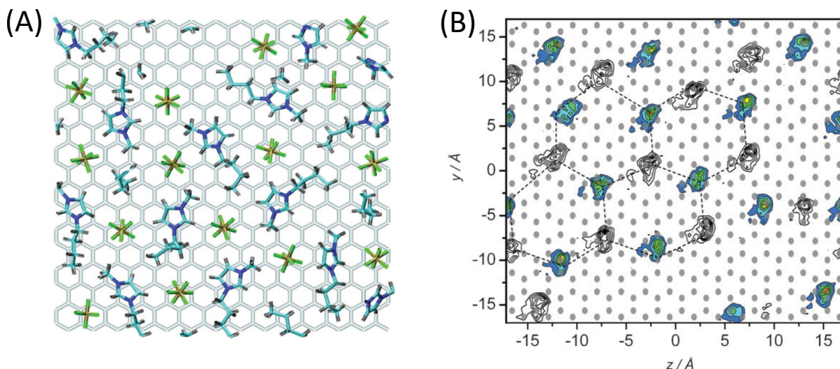
Figure 3.24: (A) snapshot taken from the MDS showing the orientation and positions of cations as well the anion in the adsorbed layer to an uncharged graphene surface (cations are represented in blue and anions in green). (B) The density contour map for the adsorbed ions formed in a 2D hexagonal lattice in the adsorbed layer. Grey circles indicate surface carbon atoms. The color map corresponds to [\text{PF}_6]^- anions; the black-and-white contour map corresponds to Imidazolium rings.
