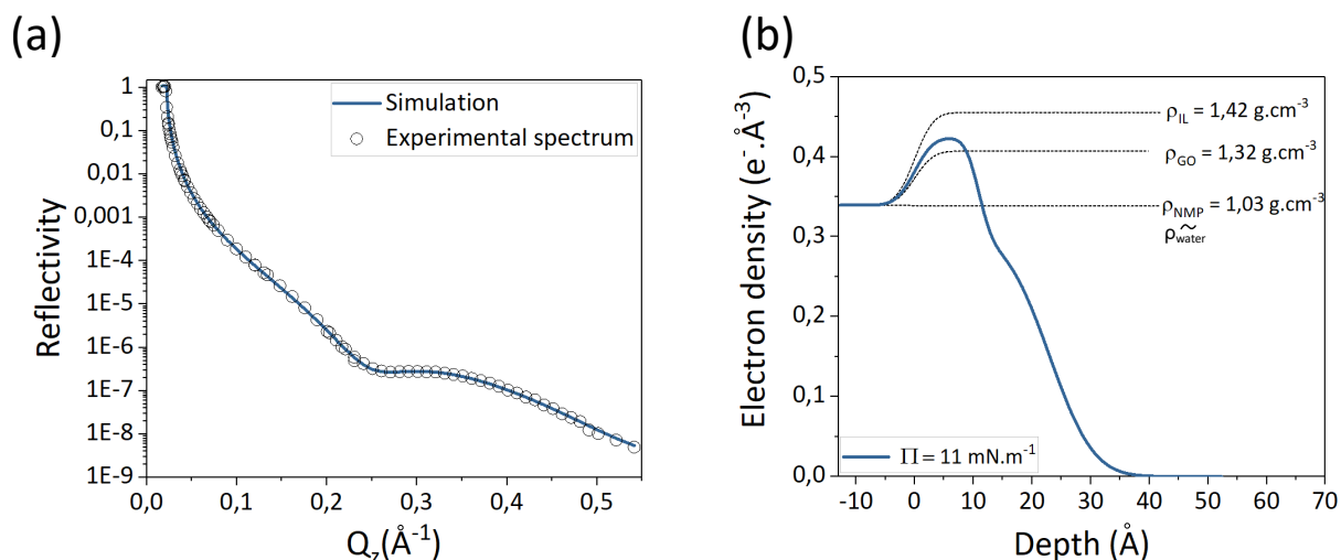
Figure 4.15: (a) XRR spectrum obtained at \Pi = 11 \text{ mN.m}^{-1} adjusted by a model of a bilayer and (b) its corresponding electron density profiles.
