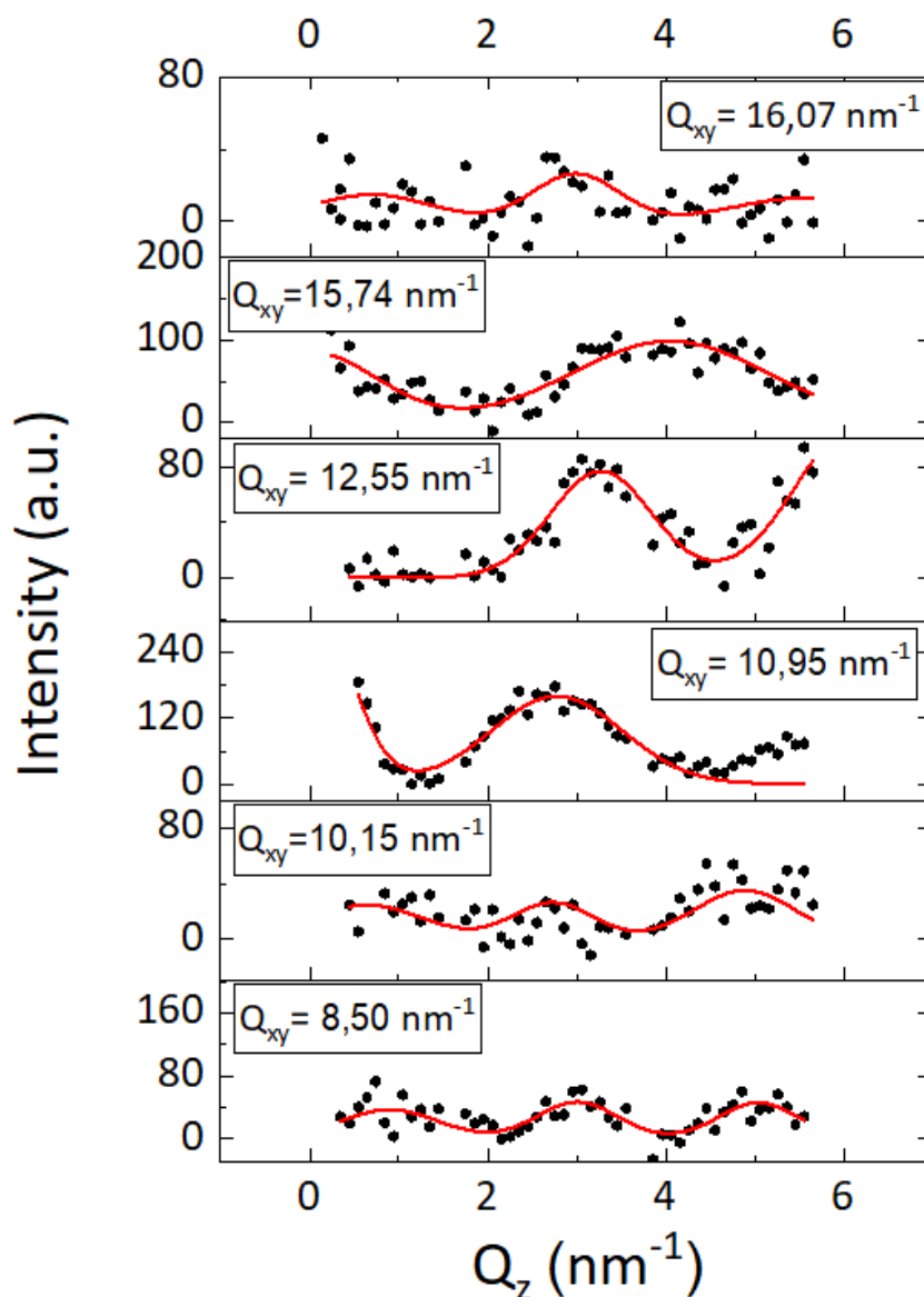
Figure 5.25: "Profile B" of the rodscons of the diffraction peaks relative to the organization of the inorganic structure coexisting with the IL Langmuir film at \Pi = 20 \text{ mN.m}^{-1} .
