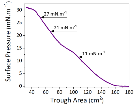
Figure 4.25: \Pi -A isotherm of (IL+GO) NMP Langmuir film deposited at the air-water interface.
