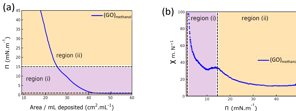
Figure 4.5: \Pi -A isotherm of (\text{GO})_{\text{methanol}} Langmuir film deposited at the air-water interface at 20^\circ\text{C} (reproduced from [39], [99]).
