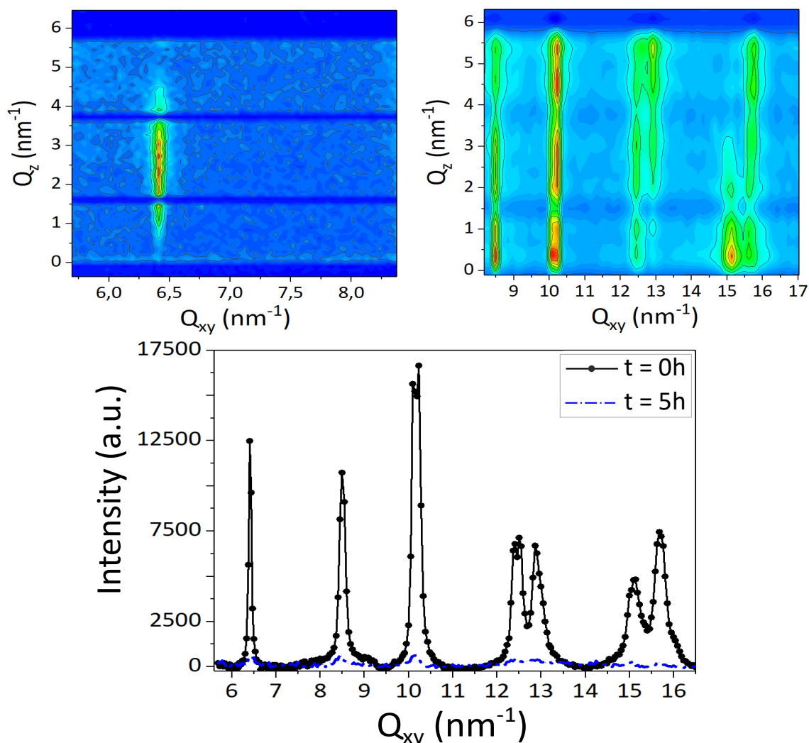
Figure 5.26: The X-ray diffraction (a) map and (b) intensities integrated over Q_z in the horizontal plane of the [C_{20}mim]^+[NTf_2]^- Langmuir film spread over a subphase containing 600 [AuCl_4]^-/IL , at \Pi = 35 mN.m -1 .
