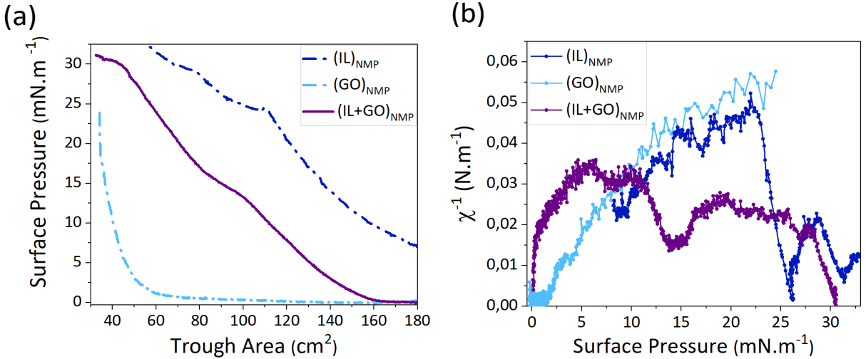
Figure 4.3: \Pi -A isotherms of ([\text{C}_{20}\text{mim}]^+[\text{NTf}_2]^-)_{\text{NMP}} , (\text{GO})_{\text{NMP}} and (\text{GO} + [\text{C}_{20}\text{mim}]^+[\text{NTf}_2]^-)_{\text{NMP}} Langmuir films deposited at the air-water interface at 20^\circ\text{C} .
