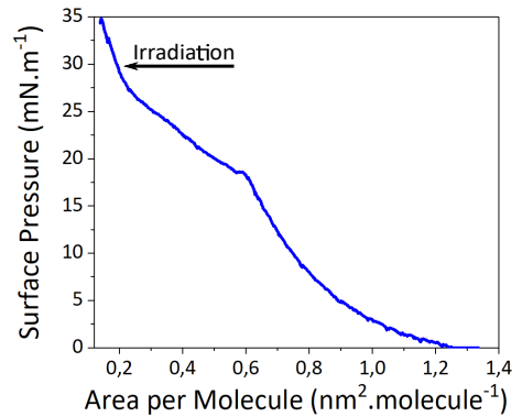
Figure 5.7: \Pi -A isotherm of the IL Langmuir film spread over a subphase containing 30 [\text{AuCl}_4]^-/\text{IL} .
