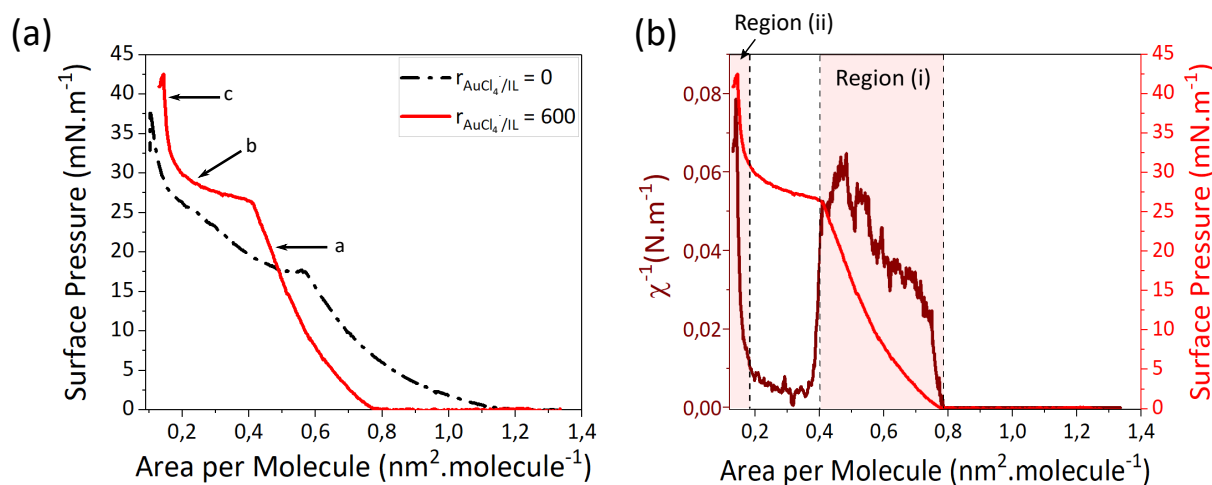
Figure 5.16: (a) II-A isotherm and (b) inverse of the compressibility of [\text{C}_{20}\text{mim}]^+[\text{NTf}_2]^- Langmuir film spread over a subphase containing 600 [\text{AuCl}_4]^-/\text{IL} .
