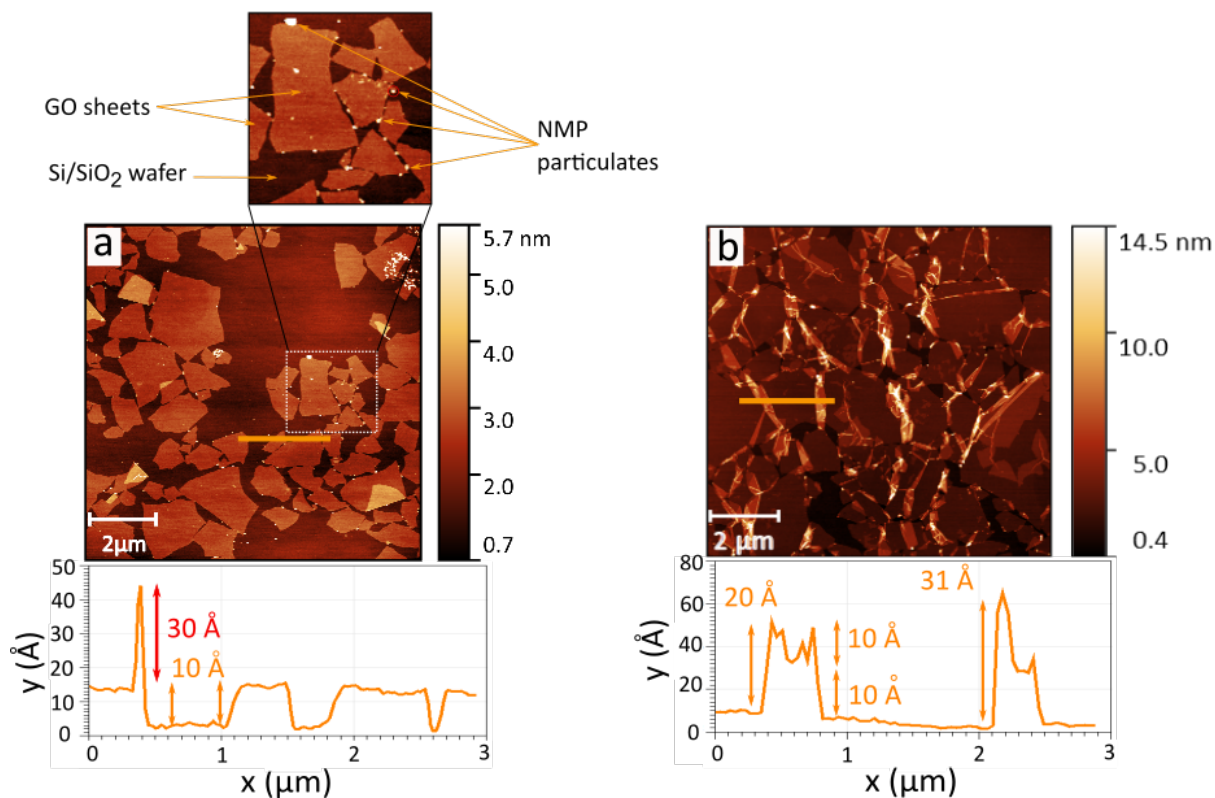
Figure 4.33: AFM topographic images and their corresponding profiles of (\text{GO})_{\text{NMP}} Langmuir film transferred on \text{Si}/\text{SiO}_2 substrates by Langmuir-Blodgett technique at (a) \Pi = 11 \text{ mN}\cdot\text{m}^{-1} and at (b) \Pi = 25 \text{ mN}\cdot\text{m}^{-1} .
