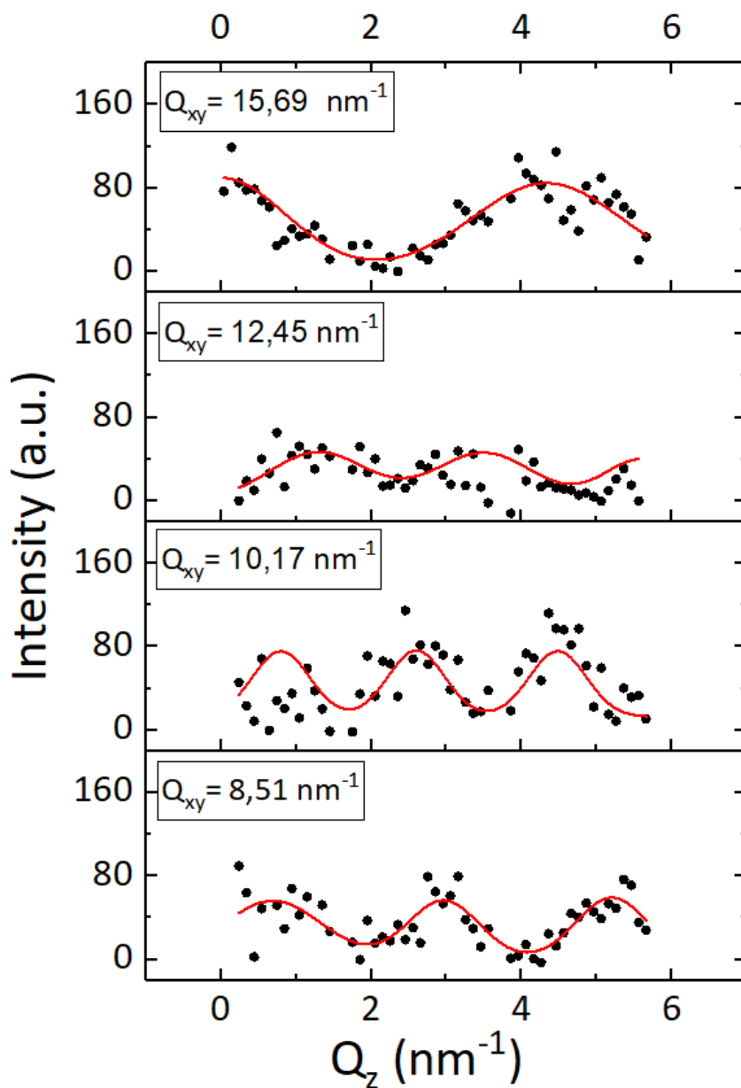
Figure 5.28: "Profile B" of the rodscaans of the diffraction peaks relative to the organization of the inorganic structure coexisting with the IL Langmuir film at \Pi = 35 \text{ mN}\cdot\text{m}^{-1} .
