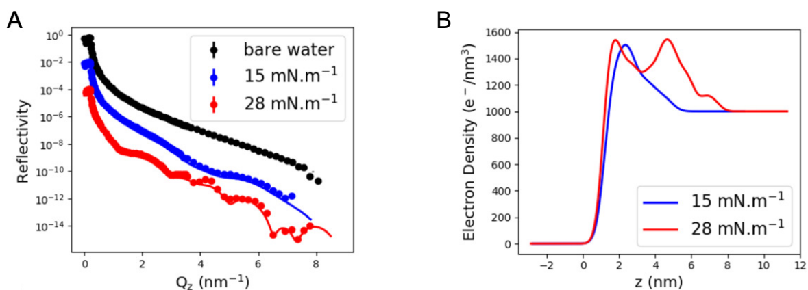
Figure 3.8: The evolution of : (A) XRR measurements and (B) the electron density profile of the [\text{C}_{20}\text{mim}]^+[\text{NTf}_2]^- Langmuir film deposited at the air-water interface (reproduced from [11]).
