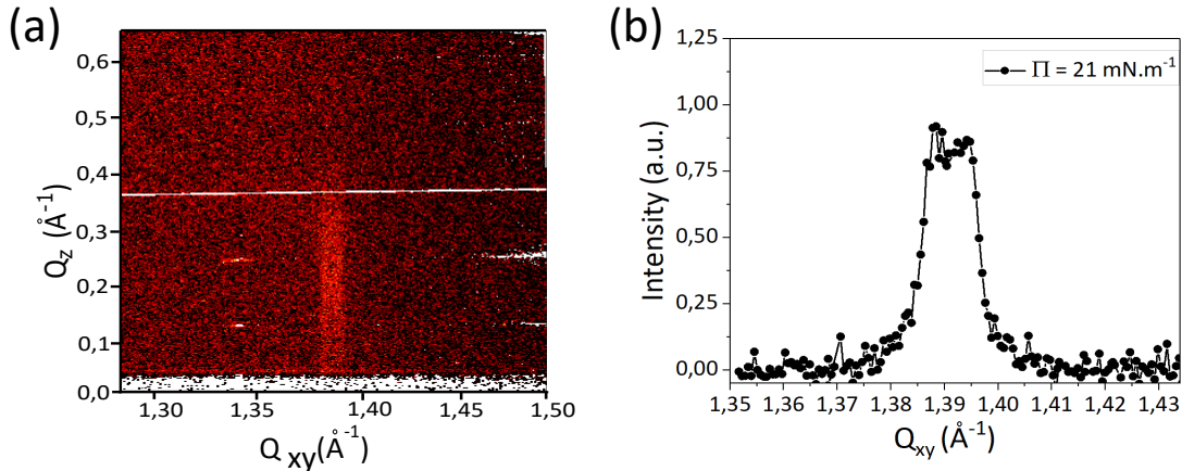
Figure 4.26: (a) The GIXD diffraction map and (b) the integrated intensity over Q_z of the GIXD signal from (GO + IL) NMP Langmuir mixed film at \Pi = 21 mN.m -1 .
