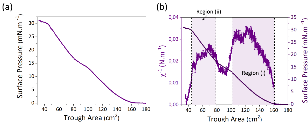
Figure 4.7: (a) \Pi -A isotherm of (IL+GO)_{NMP} Langmuir film deposited at the air-water interface and (b) its inverse compressibility.
