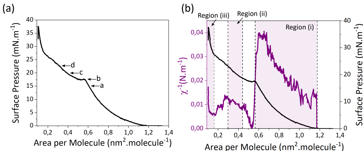
Figure 3.3: \Pi -A isotherm of [\text{C}_{20}\text{mim}]^+[\text{NTf}_2]^- Langmuir film deposited at the air-water interface.
