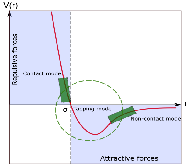
Figure 2.24: The Lennard-Jones potential shown as a function of the tip-sample distance. It also shows the different AFM imaging modes.
