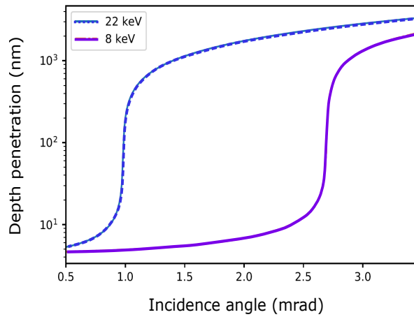
Figure 2.2: The evolution of the depth penetration of the evanescent wave in relation to the angle of incidence, for two energies.
