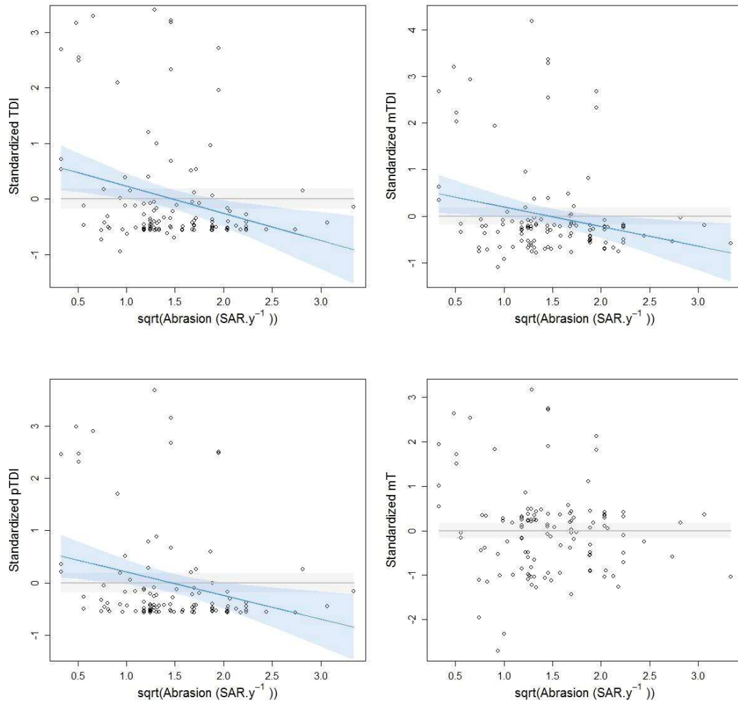
Figure E.6: Indices modelled relationships to fishery abrasion in habitat A5.25/26: Circolittoral fine sand/muddy sand. Null model (grey lines and 95% confidence interval in grey shading) was the only fitting model for mT but neglinear models (blue lines and 95% confidence interval in blue shading) were more suited for TDI, mTDI and pTDI. No significant thresholds could be detected.
