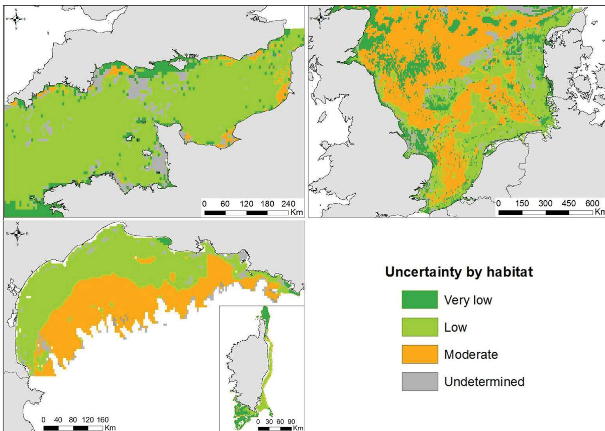
Figure 7: Models uncertainties by habitat in the three studied areas.
