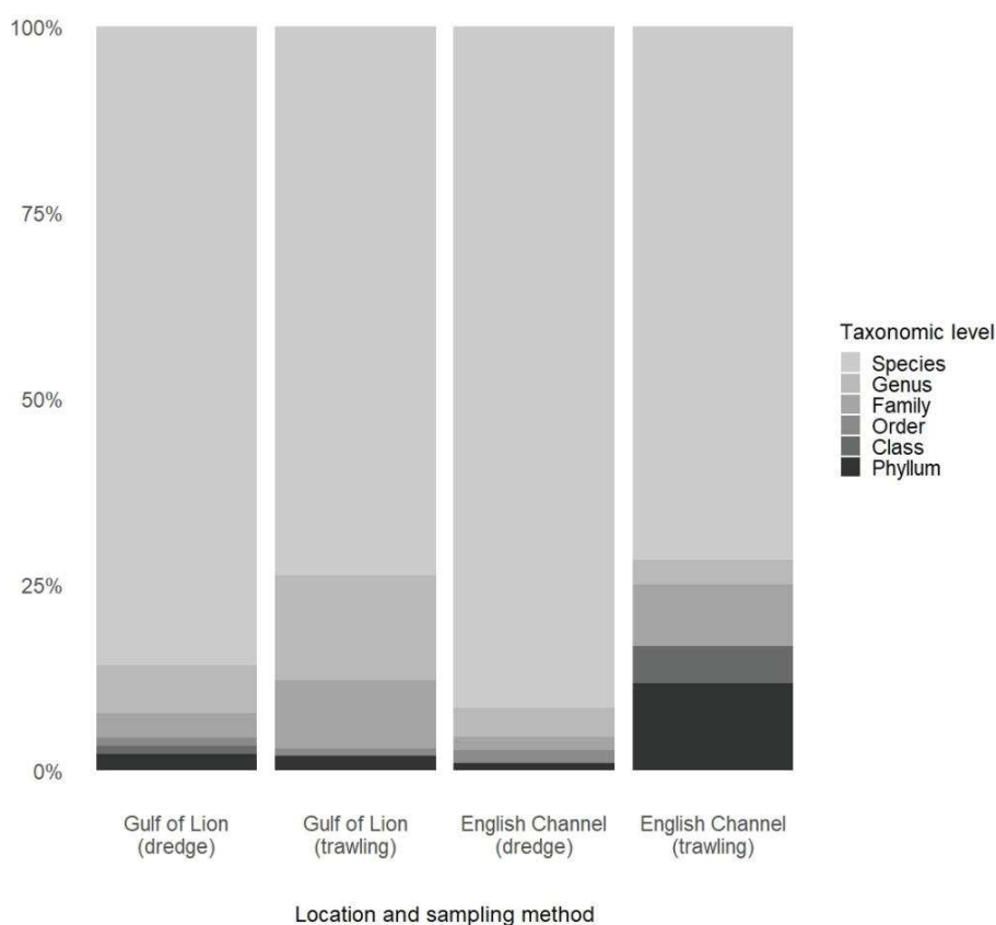
Figure 34: Proportion of each taxonomic level identified with the two sampling method in the two studied areas
