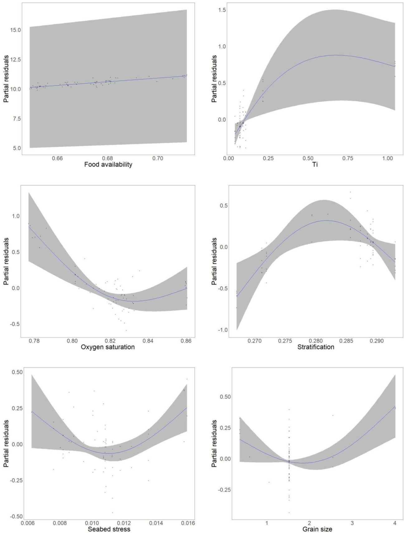
Figure G.5: Modelled relationships between environmental variables and TDI in Corsica.
