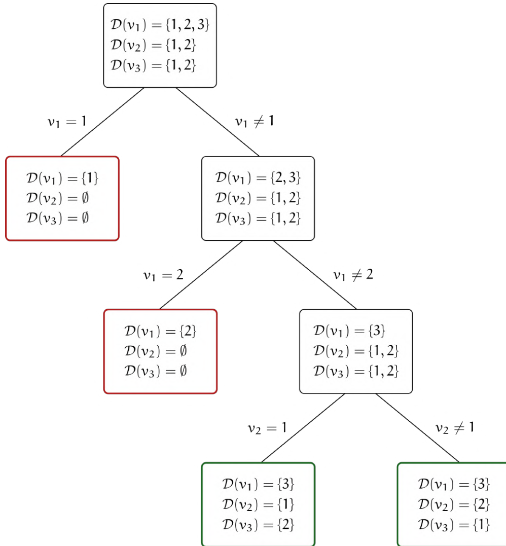
Figure 4.10: Illustration of the binary search tree associated with the deduction process depicted in Table 4.1. The root of the tree corresponds to the initial state, and each edge corresponds to a decision whose impacts on domains are indicated on the next level vertex. Red leaves correspond to contradictions and green leaves to solutions. This search tree is complete (i.e. all possible solutions are enumerated).
