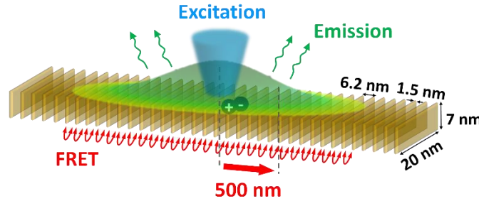
Figure 2-17. Schematic of the proposed FRET migration mechanism.
