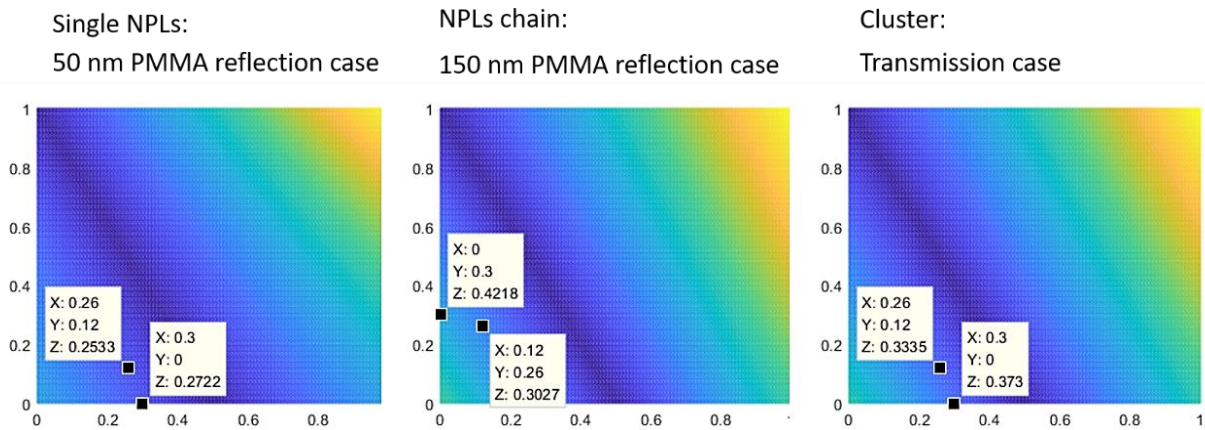
Figure 4-56. Theoretical delta difference ( \delta_{diff} ) in the single NPL, the cluster, or the chain.
