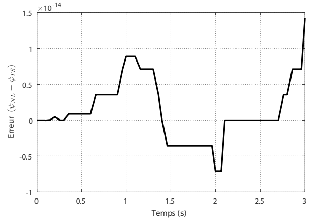
FIGURE 1.26 – Erreur \psi_{NL} - \psi_{TS} .
