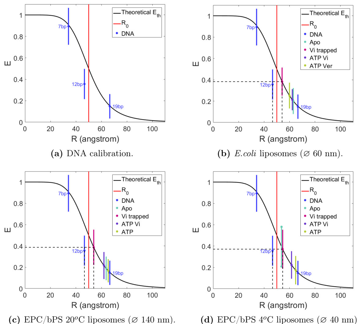
Figure 6.1: BmrA NBDs separation distances. Based on theoretical FRET efficiency (black line) calculated with R_0 = 50 Å (red line) and on the FRET efficiency calibration performed with three different interdye distances (light blue data), the distance between BmrA NBDs (positions C436) in the different conditions is estimated. Circles indicate the position of the mean in the E distribution and the bars correspond to the standard deviation, measured from the gaussian fit. For EPC/bPS 4°C liposomes, in the apo conformation, since the distribution did not exhibit a clear maximum, the circles indicate the two mean positions found with a two gaussians fit. The distance R was calculated using the theoretical E_{th} equation (6.1) and R_0 = 50 Å for visualisation purpose. The distance estimation is done using the DNA calibration data.
