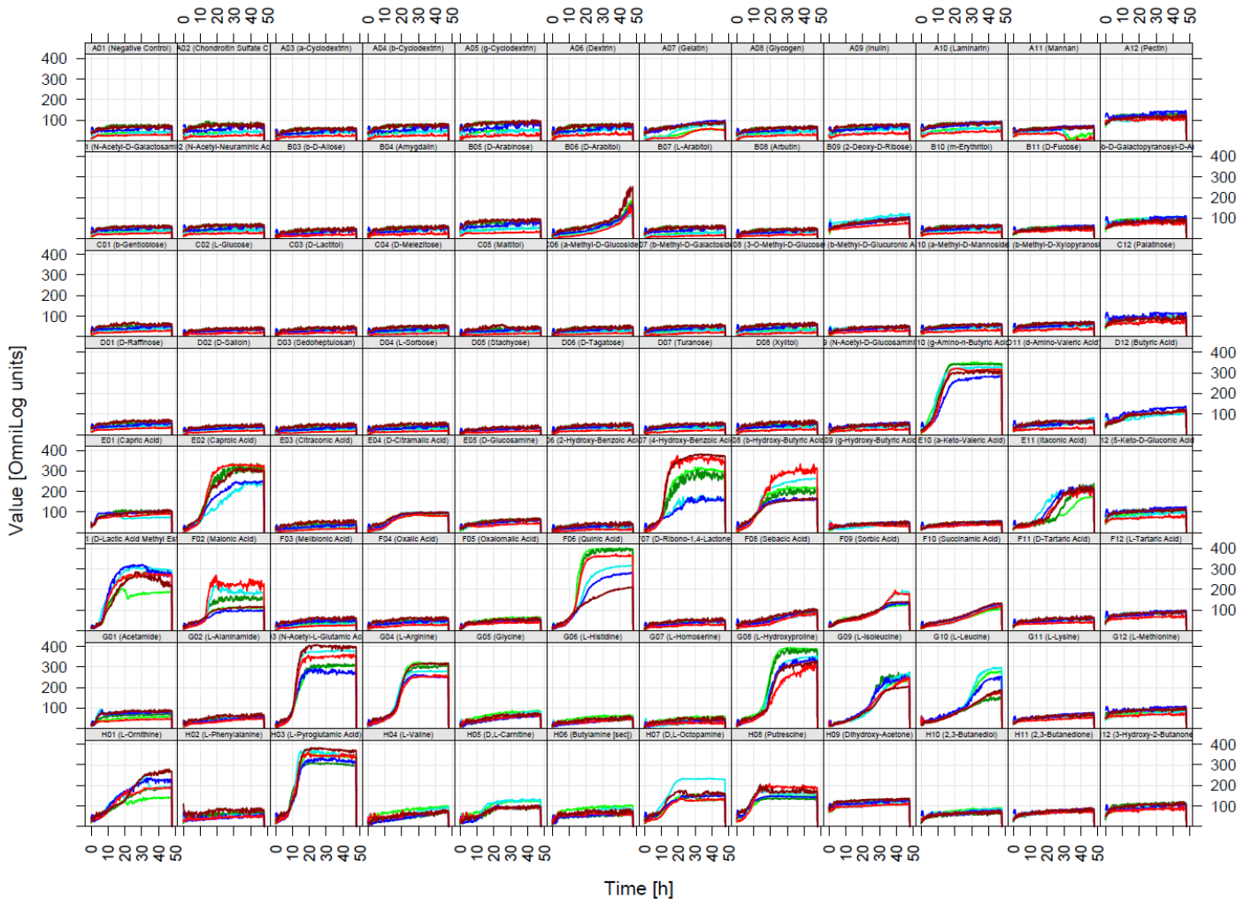
Figure 4.9: Growth fitness screen to assess ErgAB function. Biolog screen results on the PM02 plate using wild-type (reds), erfA (blues) and erfA-ergAB (greens) mutant strains in duplicates.
