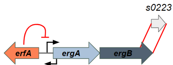
Figure 5.5: The erfA-ergAB genomic region. The s0223 sRNA is encoded at the 3'-end of the ergB gene. Transcription start sites are shown as black arrows, as predicted with BPR0M (Salamov and Solovyev, 2011).
