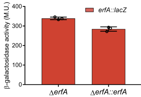
Supplementary Figure 4. ErfA binding on PergAB only has a mild effect on erfA transcription. \beta -galactosidase activities of IHMA87 strains harboring erfA::lacZ transcriptional fusion. Activities are expressed in Miller Units and are represented as mean \pm SD from three independent experiments. ErfA binding on PergAB in the intergenic region between ergAB and erfA strongly impacts ergAB transcription but only slightly diminishes erfA transcription. This mild effect does not reflect autoregulation but is probably due to steric hindrance between the RNA polymerase transcribing erfA and ErfA binding on PergAB as the two promoters are facing each other.
