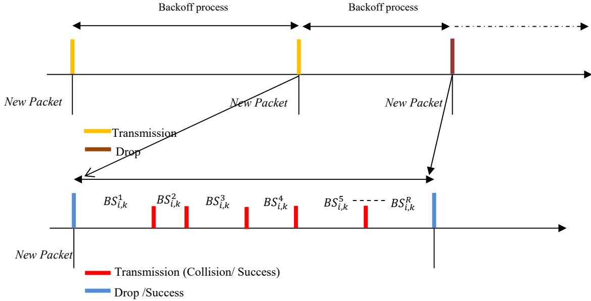
Figure 30: IEEE 802.15.6 Backoff process as a Renewal reward process
