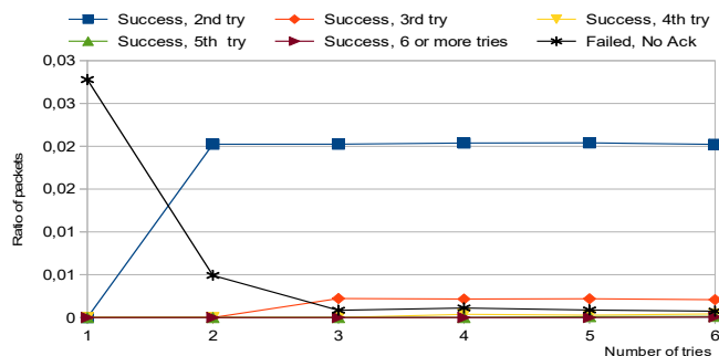
Figure 52: The effect of the max number of tries on packets breakdown at Mac Layer (arrival rate = 100 p/s)
