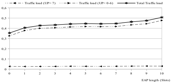
Figure 51: The effect of the EAP length on queuing traffic load (arrival rate = 100 p/s)
