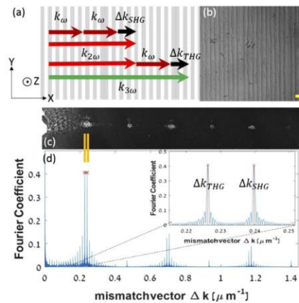
Fig. 1. (a) A schematic picture of the cascaded processes; (x,y,z) refers to the dielectric frame; k_{\omega,2\omega,3\omega} stands for the wave vectors and \Delta k_{SHG,THG} for the phase-mismatches, with no metric matching between the vector sizes and the pattern in the background. (b) Microscopy picture of the QPPKTP crystal exhibiting the poling pattern; the yellow scale bar is 28 \mu\text{m} long. (c) Far field diffraction pattern from the crystal. In orange are the peaks that correspond to the peaks used for the design. (d) Fourier Transform of the nonlinear modulation pattern, exhibiting two peaks at the mismatch frequencies, i.e. \Delta k_{SHG} = 0.24441 \mu\text{m}^{-1} for the SHG and \Delta k_{THG} = 0.22031 \mu\text{m}^{-1} for the THG.
