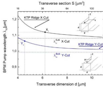
Fig. 3. Calculated SHG BPM fundamental wavelength \lambda_w versus the transversal dimension d of an x -cut (top curve) and a y -cut (bottom curve). The dashed lines indicate the bulk limit for an x -cut (top) and y -cut (bottom) KTP.
