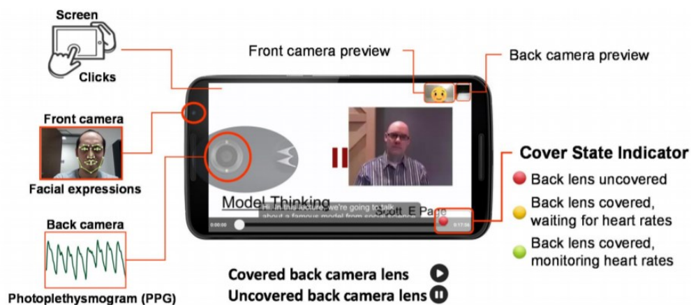
Figure 43. The primary interface of AttentiveReview [102].
