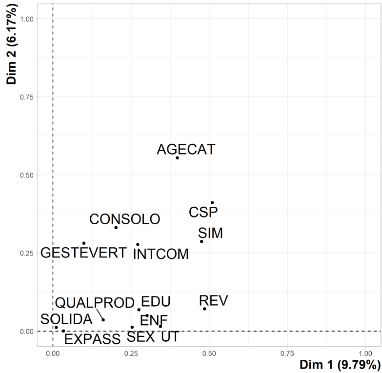
Figure 30: MCA variables graph
