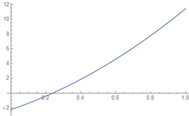
Figure 20: Scenario 4 for \pi_q
