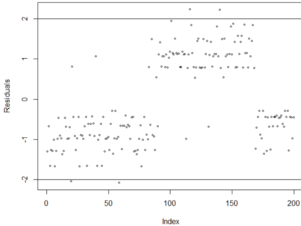
Figure 28: Residuals plot for the second estimation of M2
