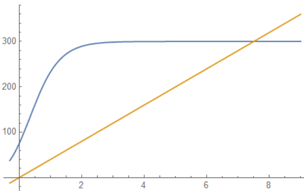
Figure 10: Scenario 3 for \pi_c
