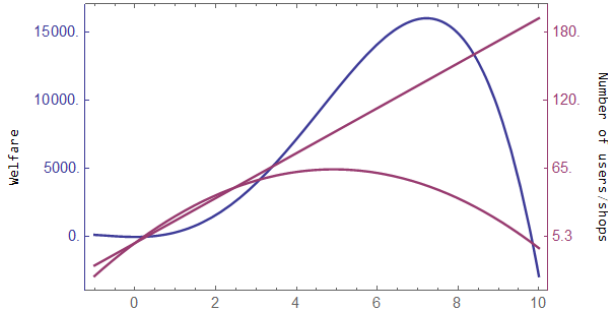
Figure 1: Scenario 1 for W
