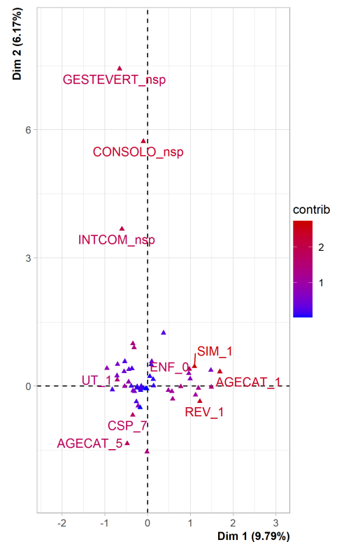
Figure 22: MCA variables graph
