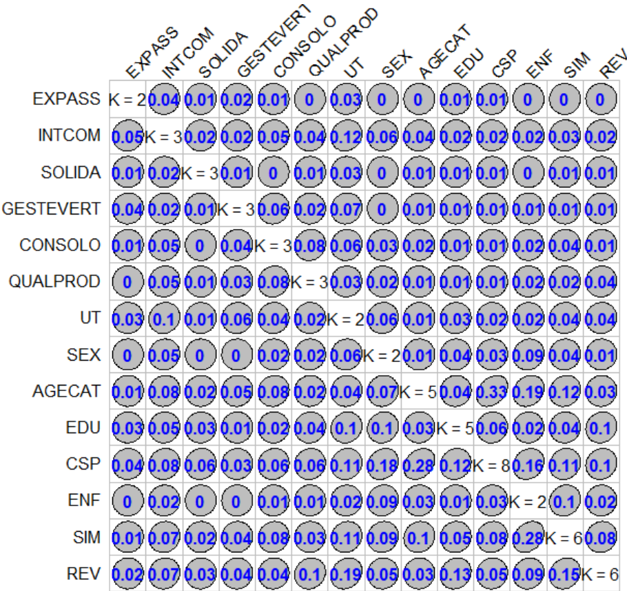
Figure 27: Goodman-Kruskal correlation matrix
