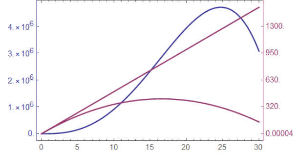
Figure 2: Scenario 2 for W
