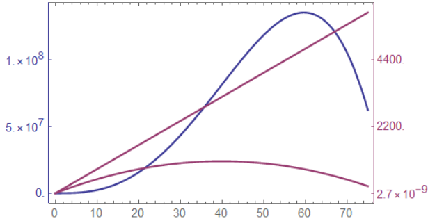
Figure 3: Scenario 3 for W
