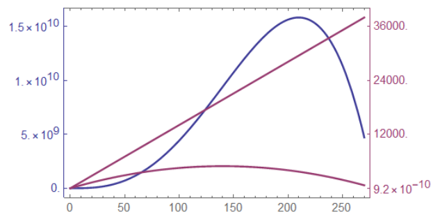
Figure 4: Scenario 4 for W
