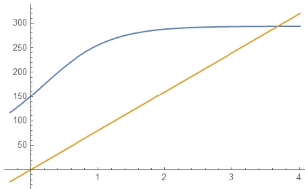
Figure 9: Scenario 2 for \pi_c
