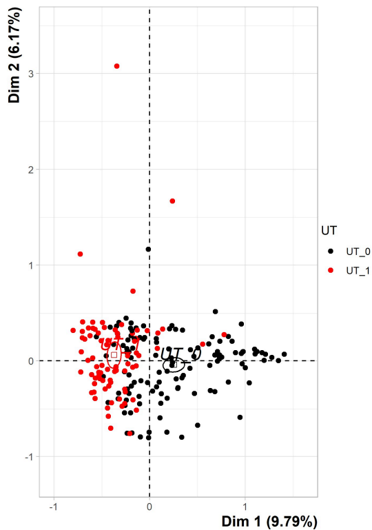
Figure 21: MCA individuals graph
