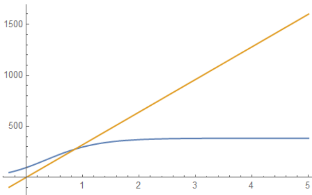
Figure 8: Scenario 1 for \pi_c
