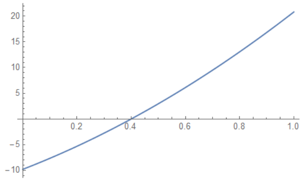
Figure 19: Scenario 3 for \pi_q
