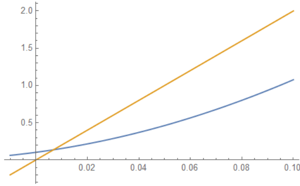
Figure 12: Scenario 4 for \pi_c scaled around zero
