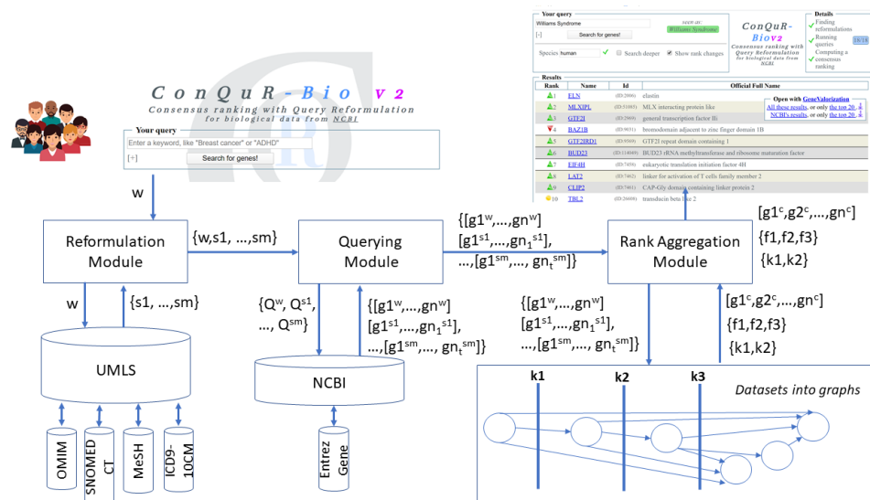
FIGURE 3.5 – Architecture de l'outil ConQuR-Bio
