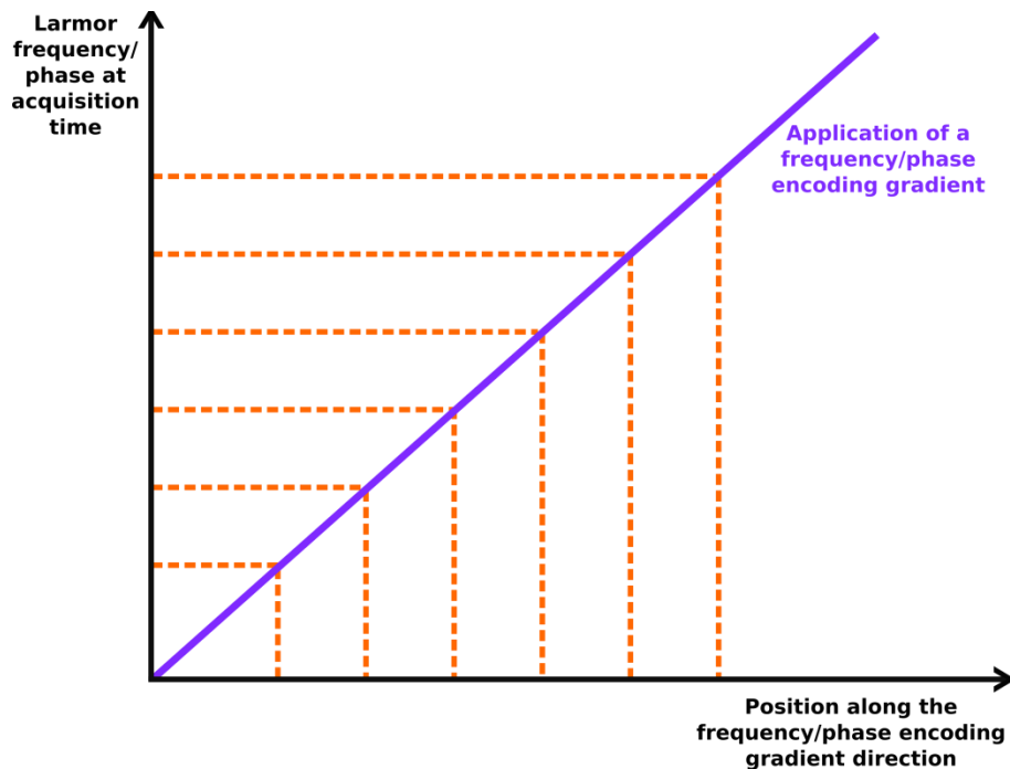
Figure 1.8: Principle of the frequency encoding of spin position.
