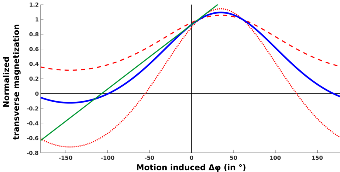
Figure 4.16: Representation of the average transverse magnetization \langle M_{xy} \rangle_{UTE\ Rep} as a function of the motion induced dephasing \Delta\varphi (blue curve), with the transverse magnetization available during the first (red dots) and the last (red dashes) UTE repetitions performed after any MSPREP pulse, and the affine approximation of \langle M_{xy} \rangle_{UTE\ Rep}(\Delta\varphi) around \Delta\varphi = 0 (green). We observe that, close to \Delta\varphi = 0 , we have a quasi-affine relationship between the average transverse magnetization and \Delta\varphi in the range of [-20^\circ + 20^\circ] . We also observe that transverse magnetization can vary a lot from the first to the last UTE repetition, which can cause artifacts in the final image.
