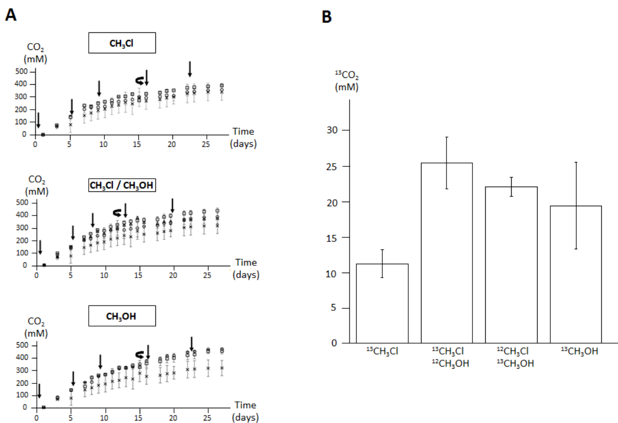
Figure 4.2. Carbon mineralization in the SIP experiment
