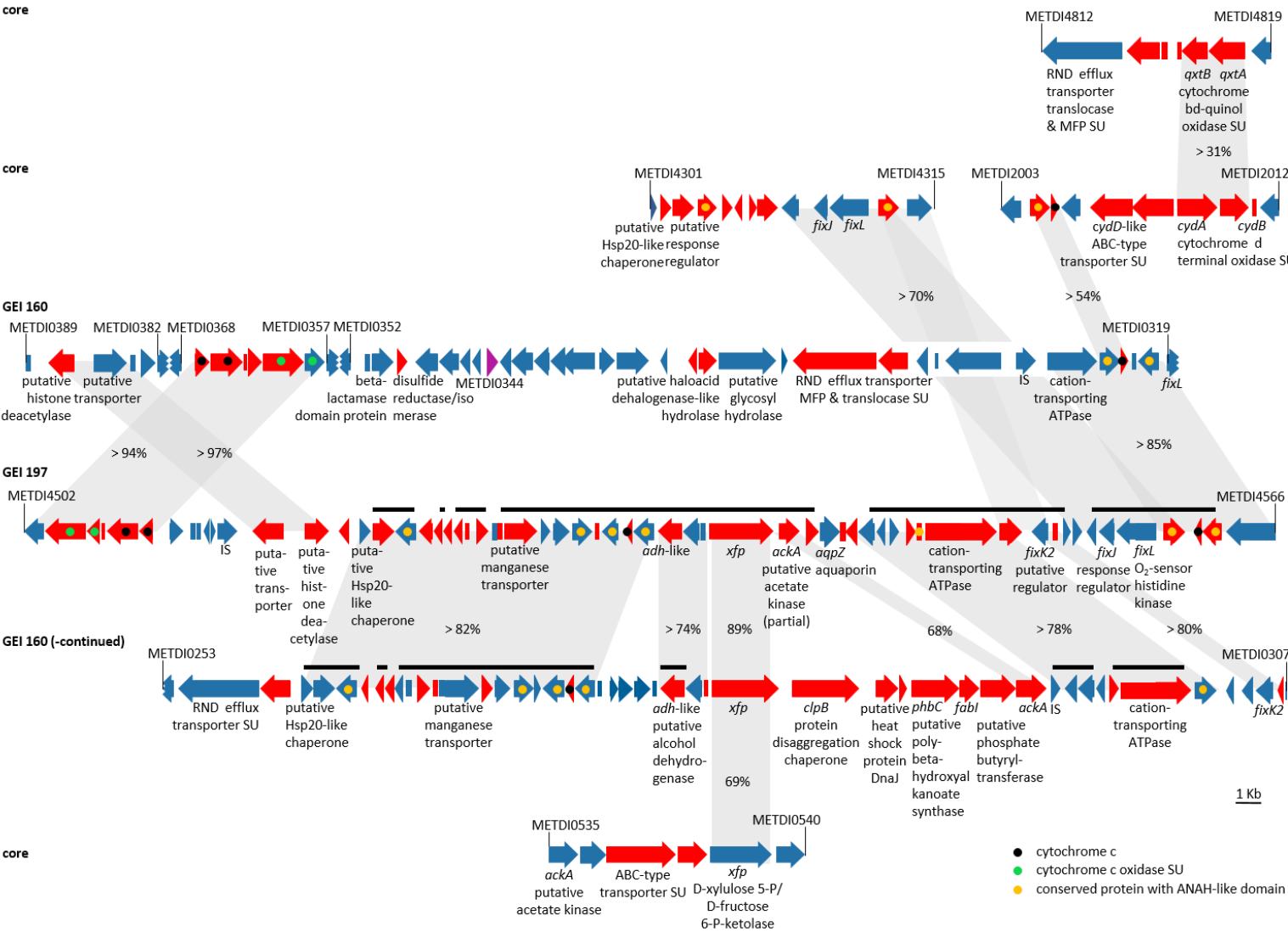
FIGURE S3 Transcription profiles and gene redundancy of key gene clusters more highly transcribed in methanol- than dichloromethane-grown cultures of M. extorquens DM4
