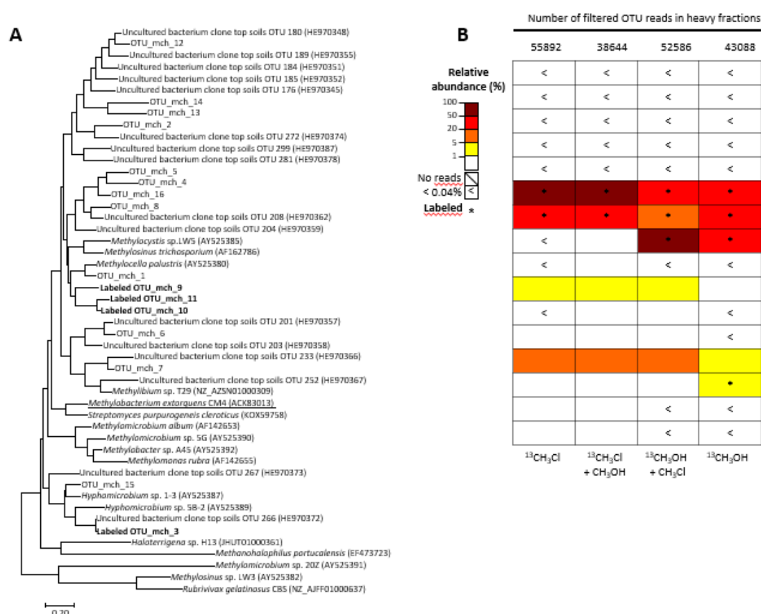
Figure 4.8. Affiliation and relative abundance of mch OTUs
