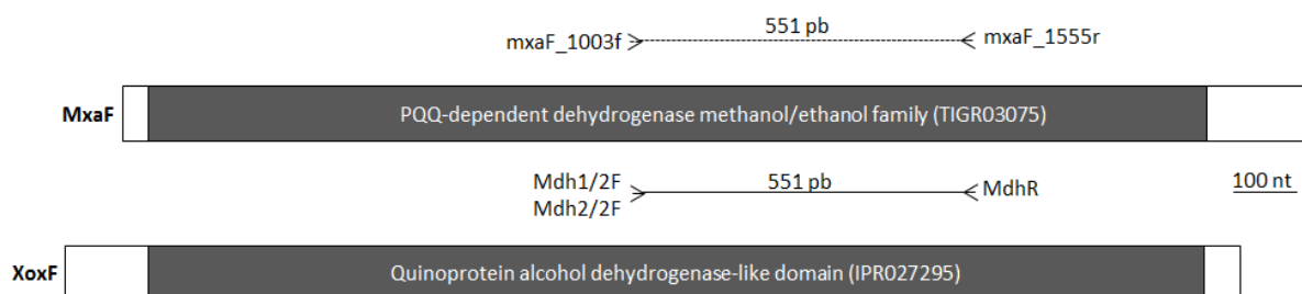
Figure 2.7. PCR amplification of methanol dehydrogenase-like MxoF and XoxF encoding genes
