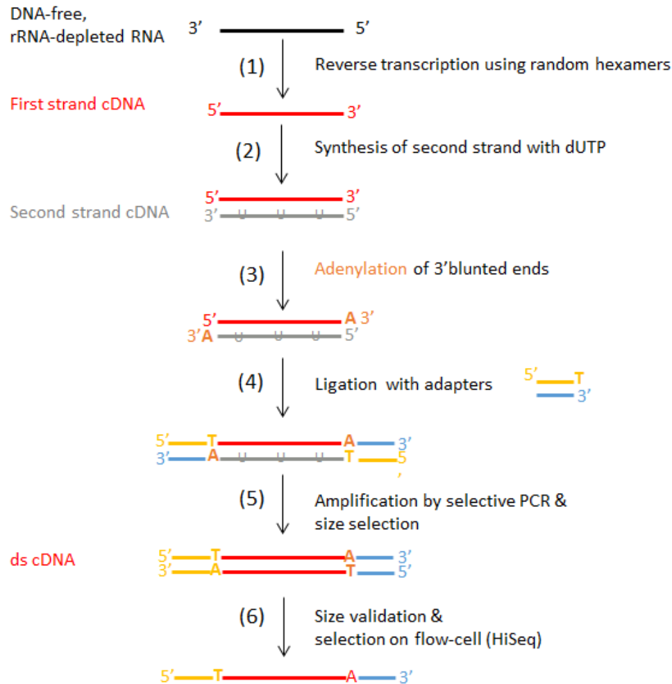
Figure 2.2. Directional cDNA bank construction
