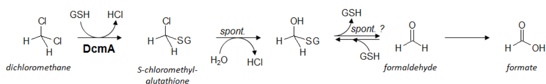
Figure 1.12. Dichloromethane degradation by the hydrolytic pathway of glutathione S-transferase
