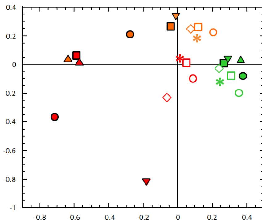
Figure 4.3. Clustering analysis of 16S rRNA gene amplicon sequence datasets from all microcosms
