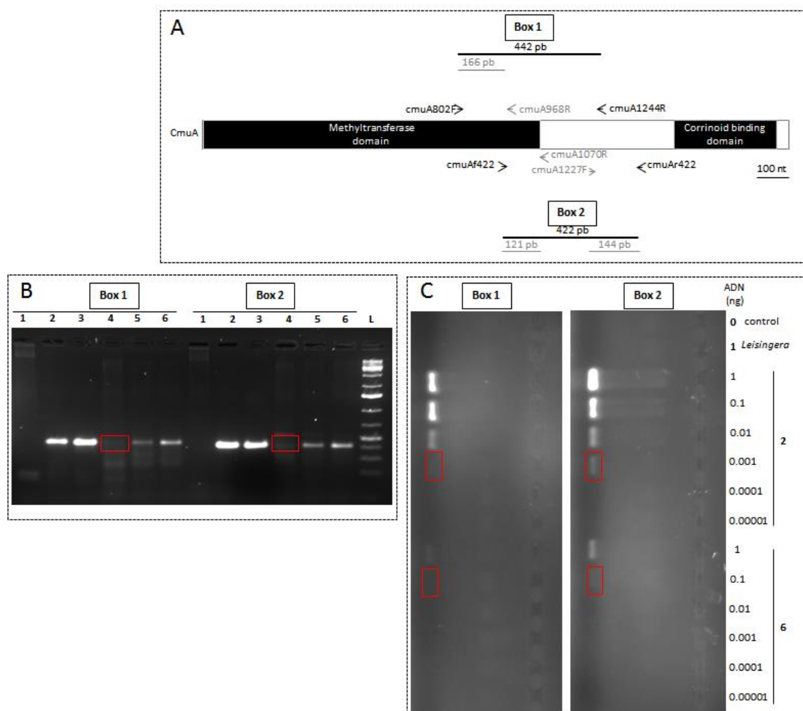
Figure 2.6. Comparing two sets of primers targeting environmental chloromethane dehalogenase CmuA-encoding gene
