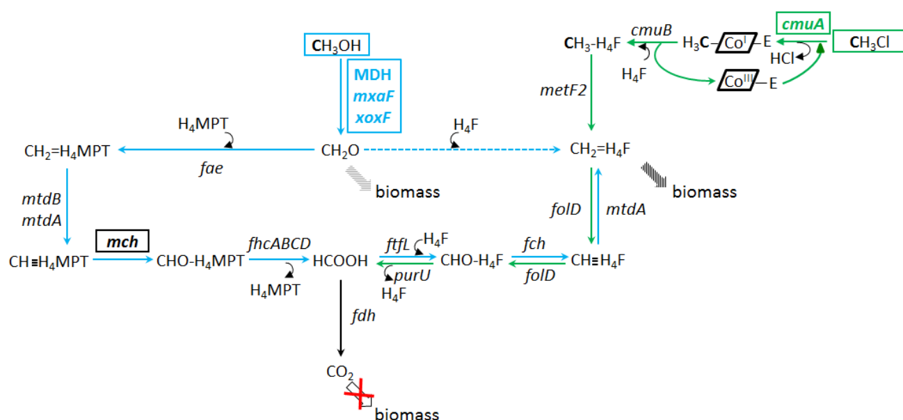
Figure 4.1. Targeted functional genes in methylotrophic utilization of chloromethane and methanol
