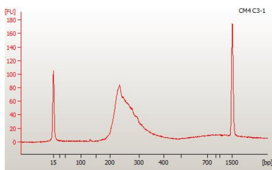
Figure 2.3. Validation of cDNA bank constructions with the 2100 Bioanalyzer
