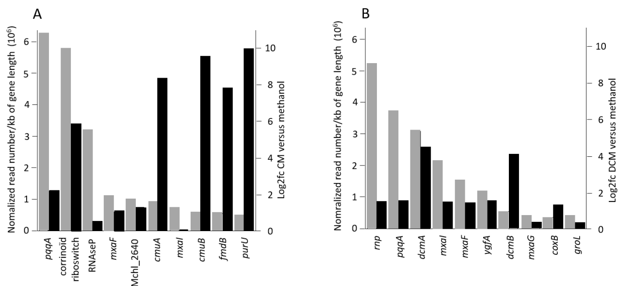
FIGURE S2 Genes with highest differential transcription in cultures grown with chlorinated methanes compared to methanol
