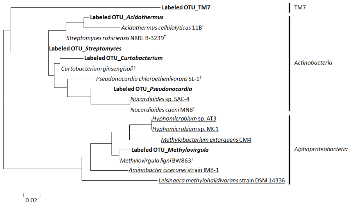
Figure 4.5. Phylogenetic relationships between partial sequences of the 16S rRNA gene of labeled OTUs and of reference chloromethane-utilizing strains
