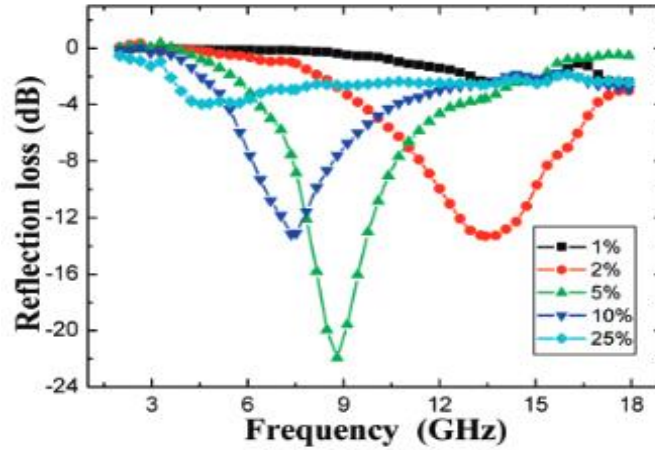
Figure I.37. Reflection coefficients of the SWNTs loaded polyurethane composites of 2 mm thickness using different wt.% of SWNTs (0-25 wt.%) [105].
