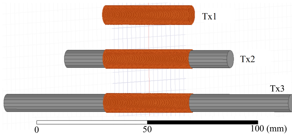
Figure 3.24: 3D models of different transmitter coils used during experimental work used for ANSYS Q3D simulation.
