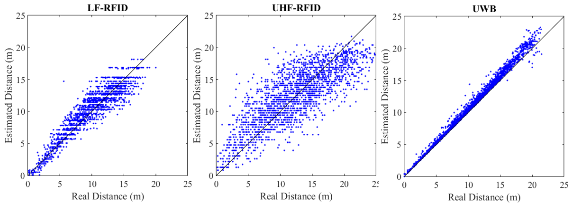
Figure 4.16: Actual versus estimated distances for all base stations in DOT, UHF-RFID and UWB systems.
