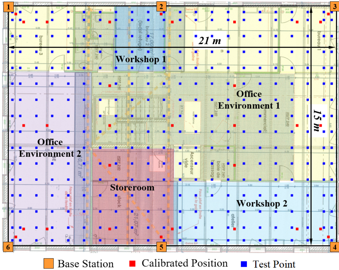
Figure 4.5: Experimental area showing different environments and positions of base stations for positioning experiment inside a building with DOT system.
