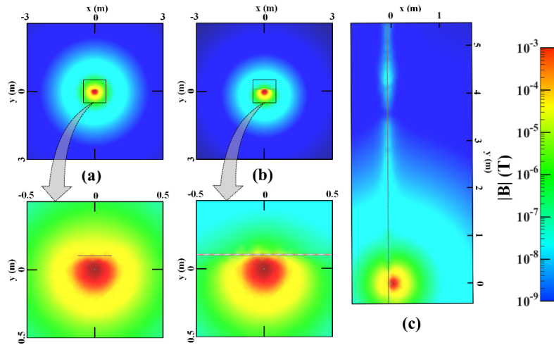
Figure 3.22: Simulation set 2: Magnetic field distribution around the transmitter with (a): obstacle size 0.25 \text{ m} \times 0.25 \text{ m} \times 0.004 \text{ m} ; (b): obstacle size 1 \text{ m} \times 1 \text{ m} \times 0.01 \text{ m} . (c): mesh of steel bars of diameter 0.01 \text{ m} .
