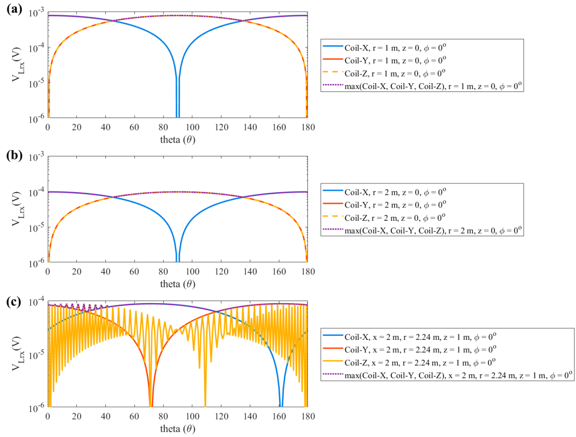
Figure 3.10: Voltage induced, obtained from (2.20), in individual coils of 3-axes receiver antenna due to field created by helical coil. Curves labeled as ‘max(Coil-X, Coil-Y and Coil-Z)’ represent the maximum induced voltage among three orthogonal coils of 3-Axes antenna.
